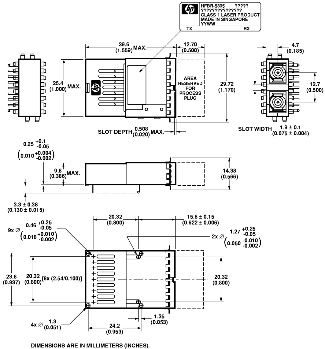
Figure 5. Package Outline Drawing for HFBR-5303F.
