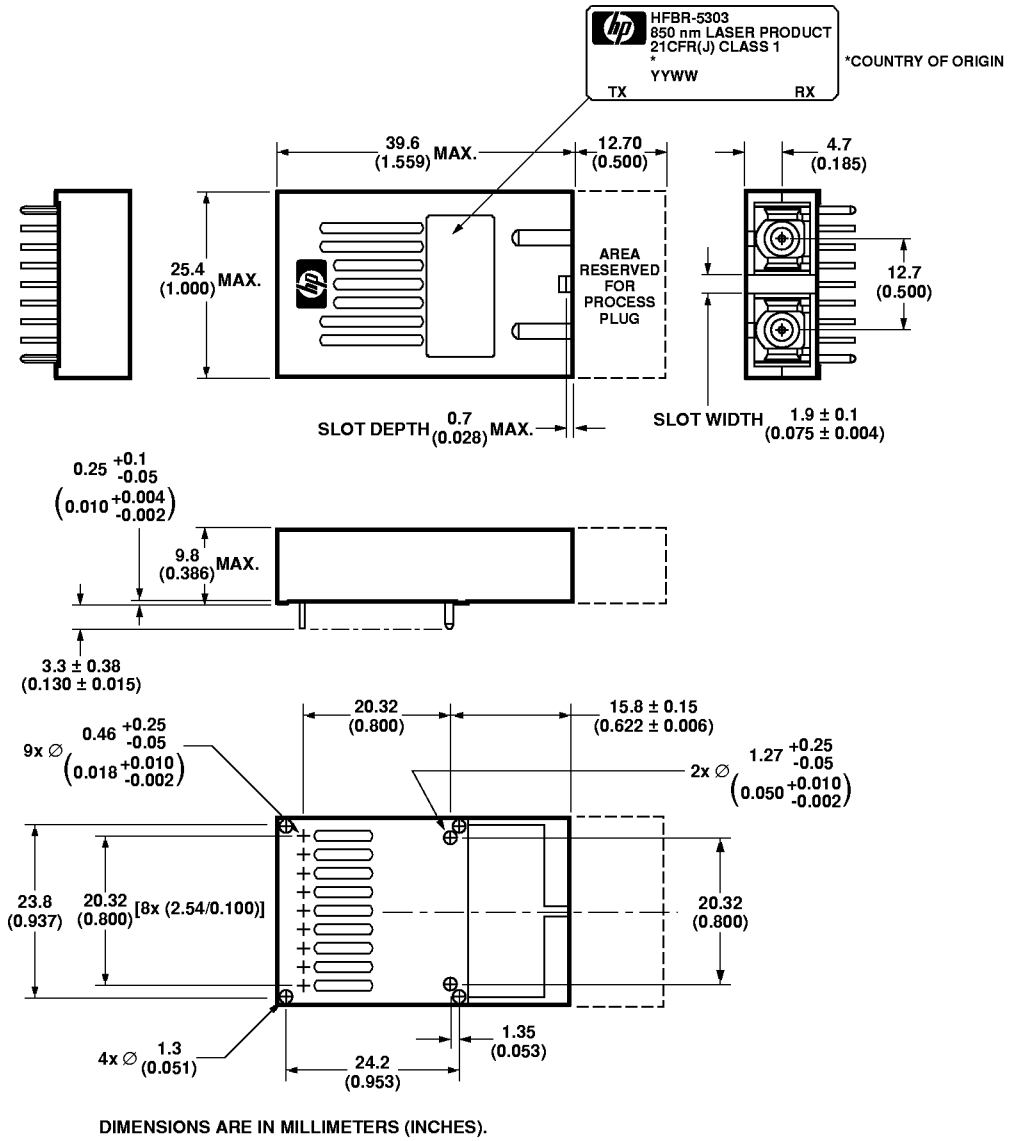
Figure 3. Package Outline Drawing of HFBR-5303.
