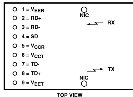
Figure 2. Pin-Out.
