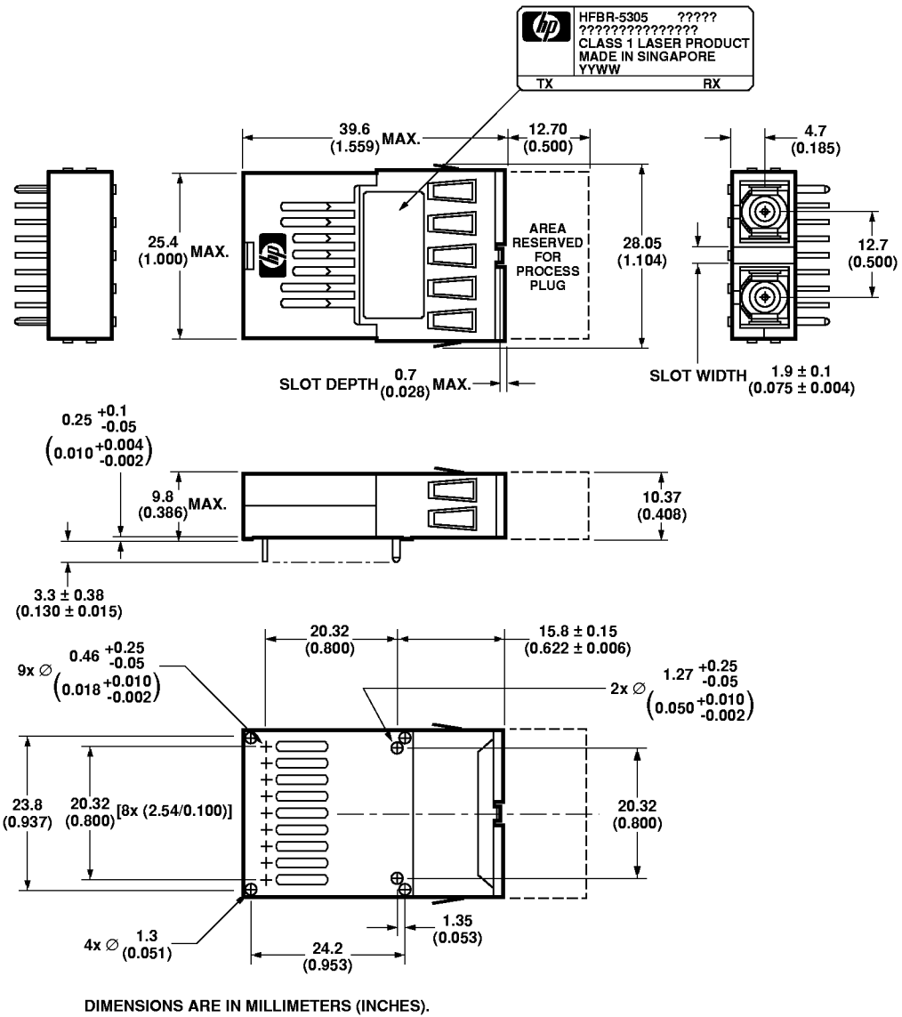
Figure 4. Package Outline for HFBR-5303E.
