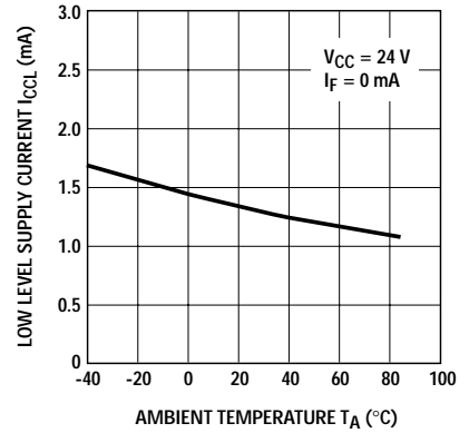
Figure 40. Typical Low Level Supply Current vs. Ambient Temperature, HCPL-3101.
