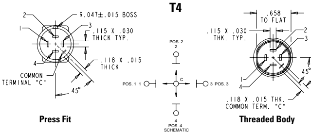
Threaded Body
