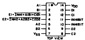
Terminal Assignment
