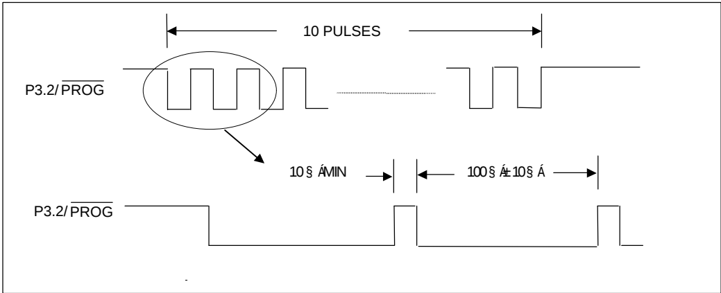
Figure 8. Programming Waveform
