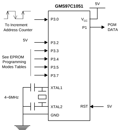
Figure 6. Verifying the EPROM Memory
