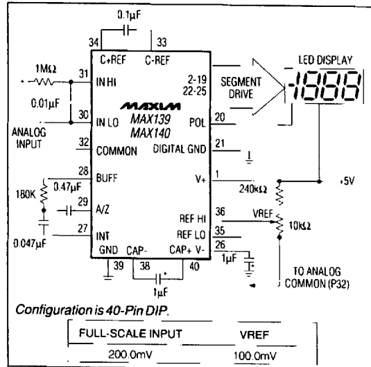
Figure 2. MAX139/MAX140 Typical Operating Circuit
