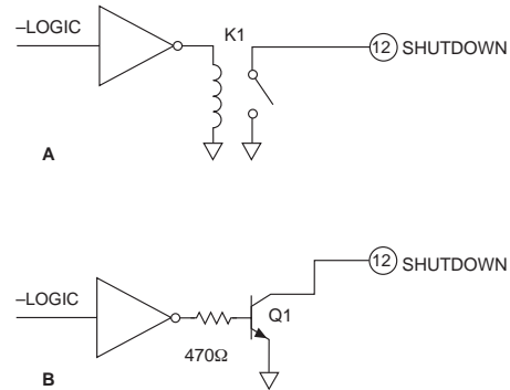
FIGURE 2. SHUTDOWN OPERATION
