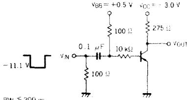
t_{on} SWITCHING
