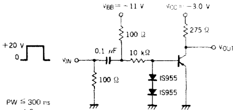
t_{off} SWITCHING
