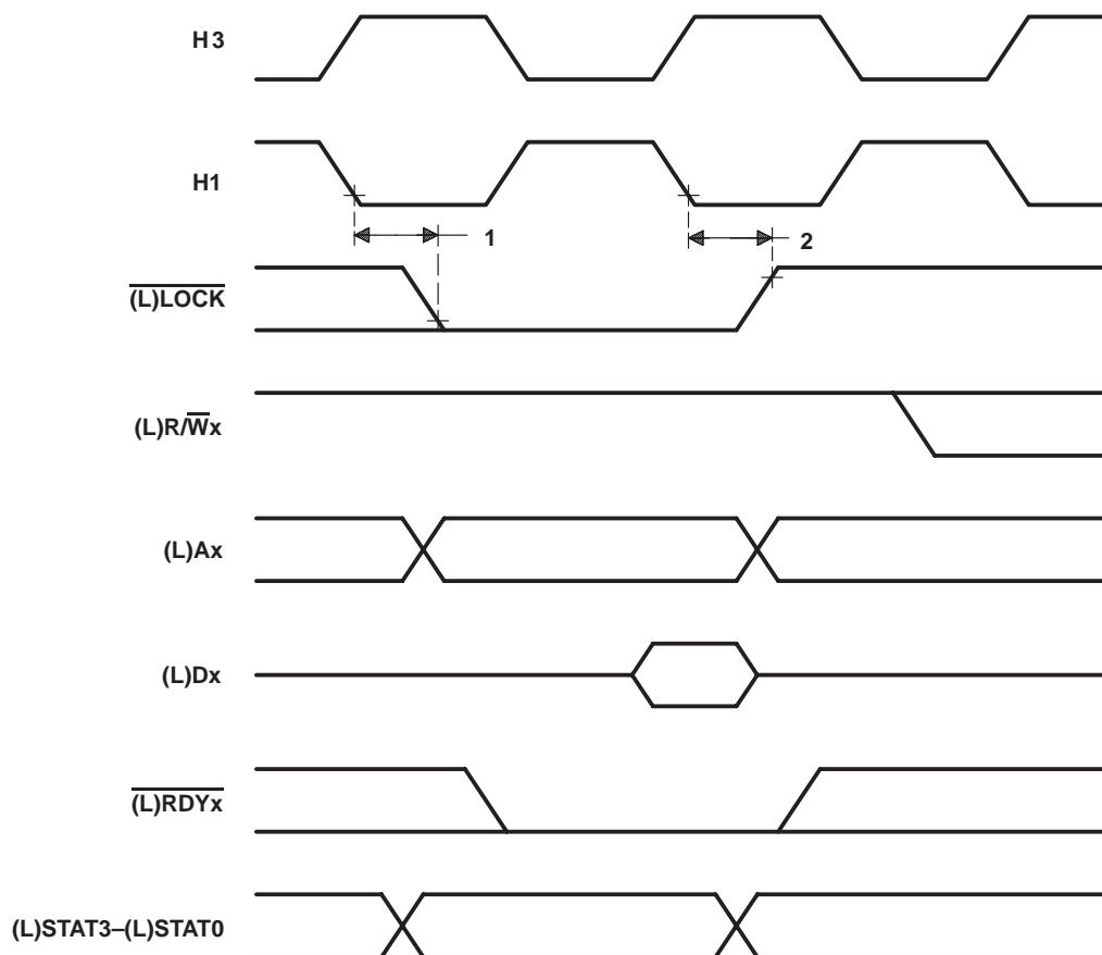
Figure 15. Timing for \overline{\text{(L)LOCK}} When Executing SIGI
