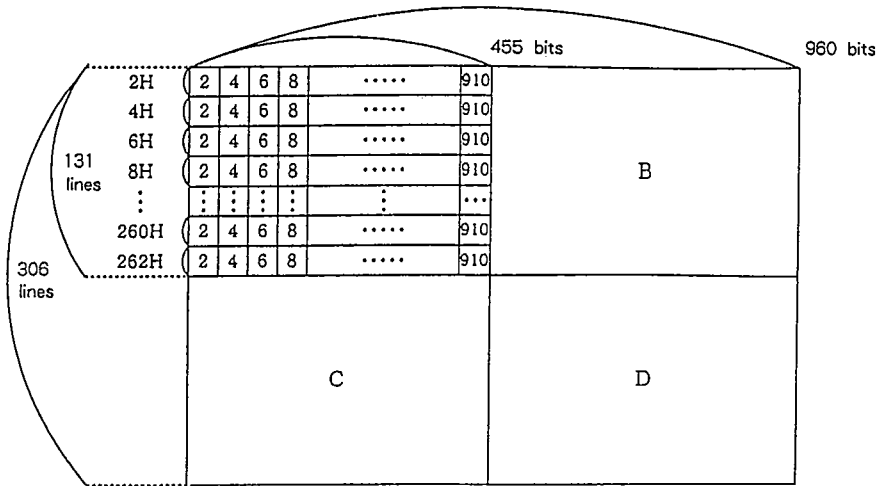
Fig. Inside of the memory
