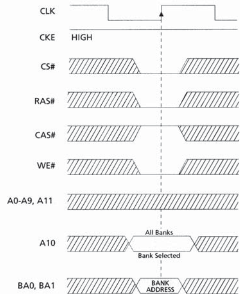
FIGURE 20: PRECHARGE Command
