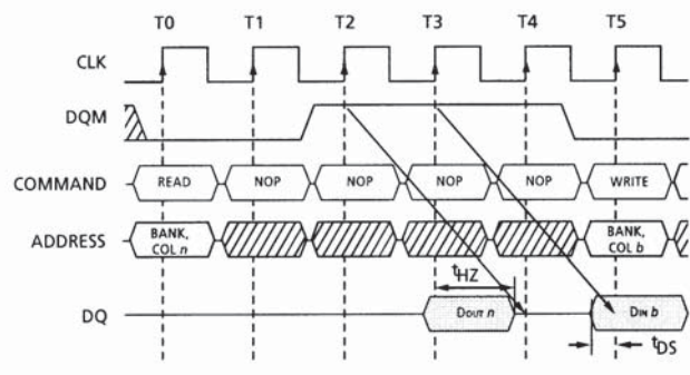
FIGURE 10: READ to WRITE With Extra Clock Cycle
