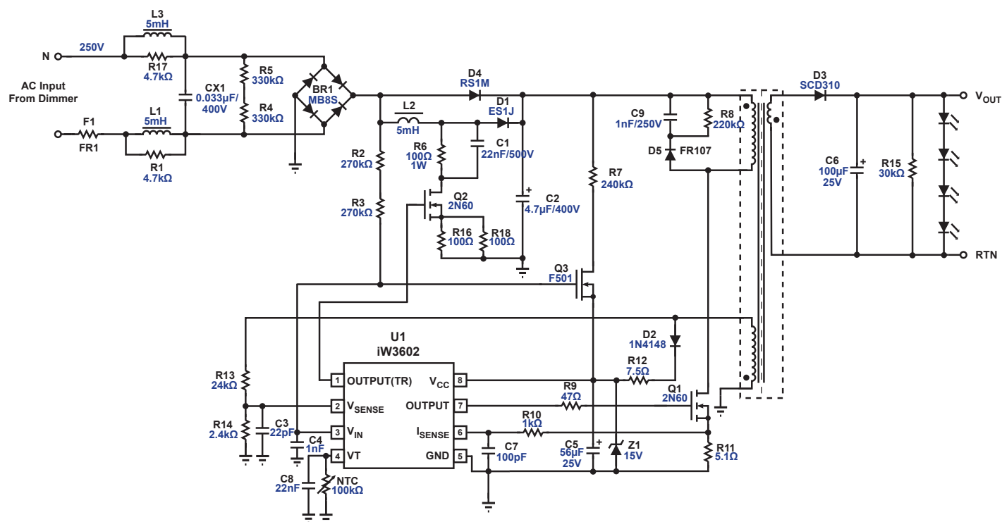
Figure 11.1 : iW3602 Typical Application Schematic
