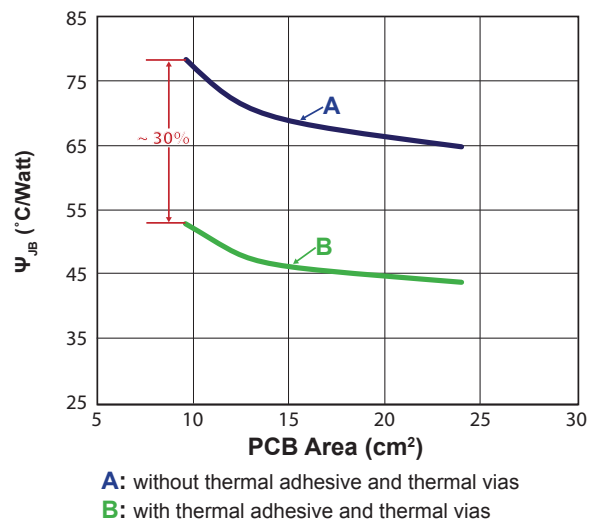
Figure 9.15 : Effect of Thermal Resistance Improvements
