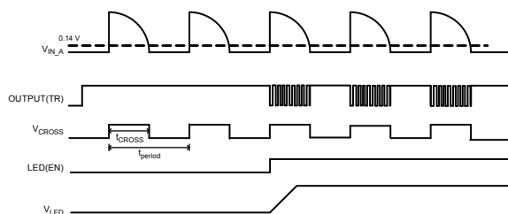
Figure 9.3 : Dimmer Detection
