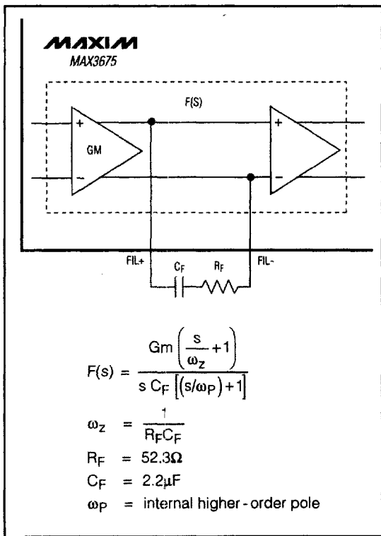
Figure 2. Loop Filter
