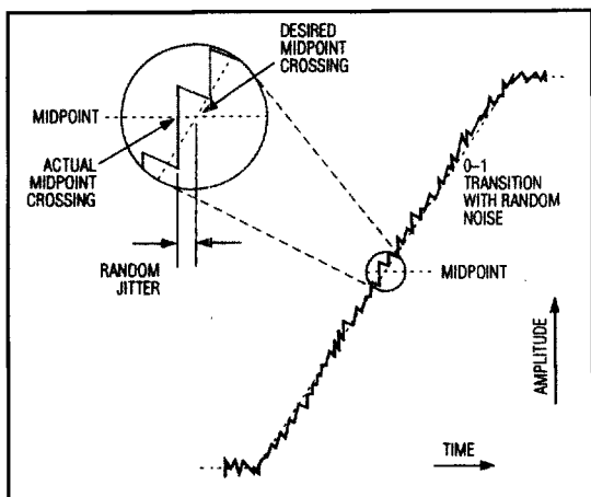
Figure 8. Random Jitter on Edge Transition
