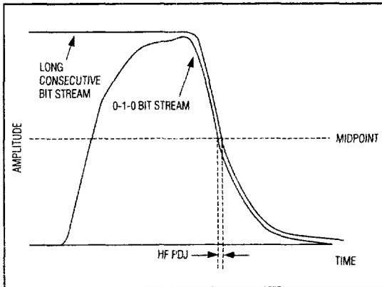
Figure 10. Pattern-Dependent Jitter Due to High-Frequency Roll-Off
