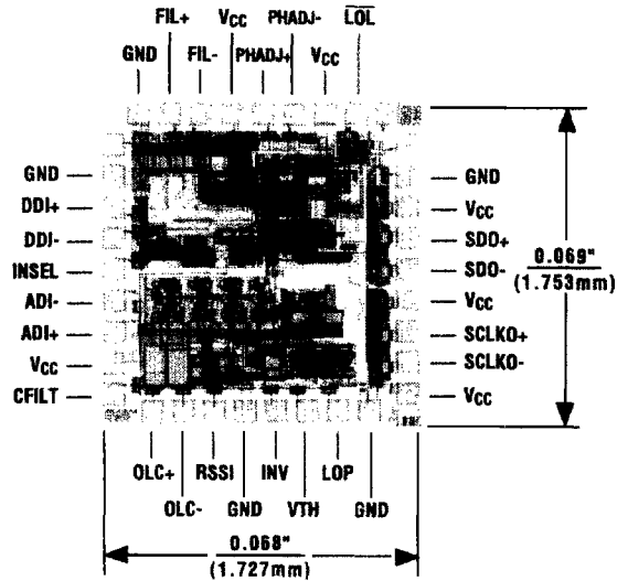
Chip Topography
