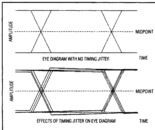
Figure 7. Eye Diagram With and Without Timing Jitter
