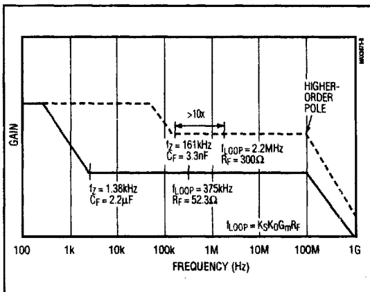
Figure 3. Loop-Filter Response
