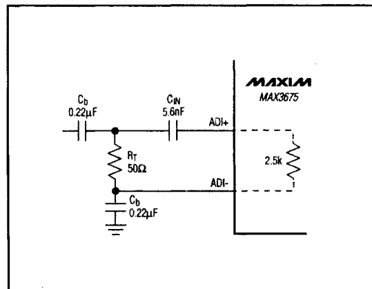
Figure 5. Single-Ended Input Termination
