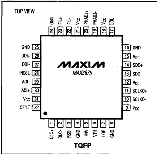
Pin Configuration
