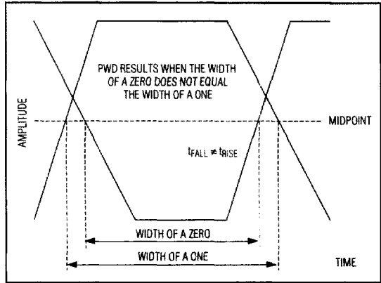
Figure 11. Pulse-Width Distortion
