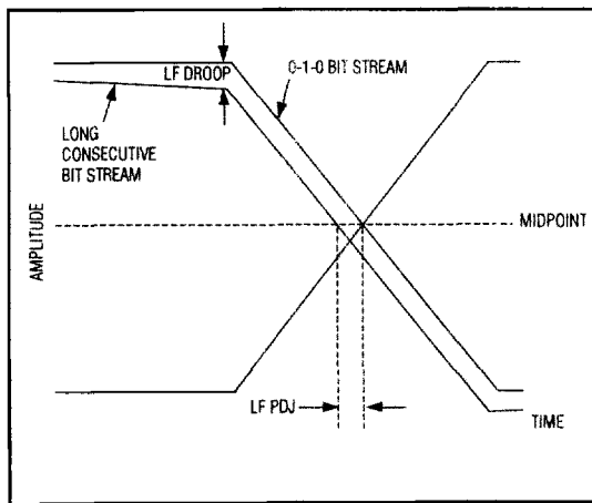
Figure 9. Pattern-Dependent Jitter Due to Low-Frequency Cutoff
