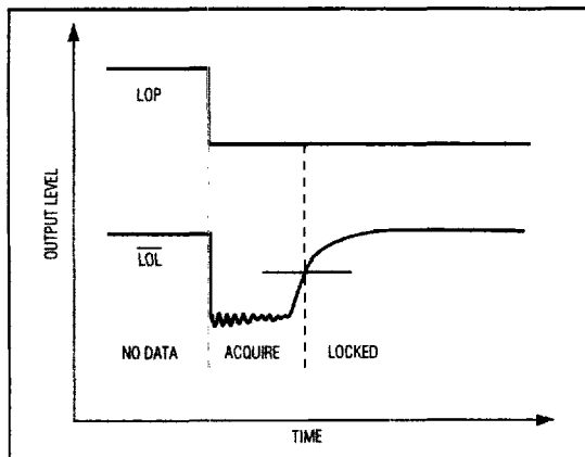
Figure 4. Loss-of-Lock Output
