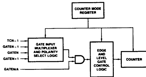
Figure 12. Gating Control
