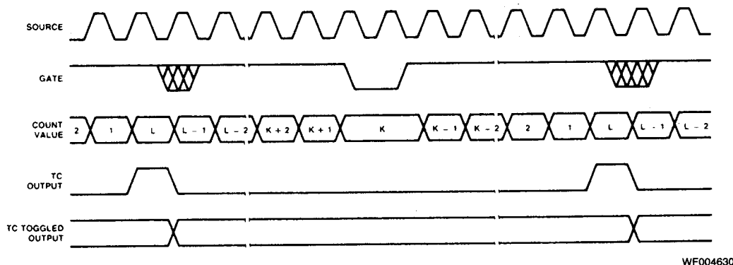
Figure 15e. Mode E Waveforms
