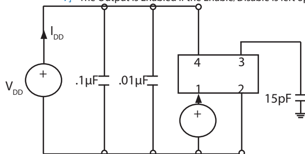
Fig 1: Test Circuit
