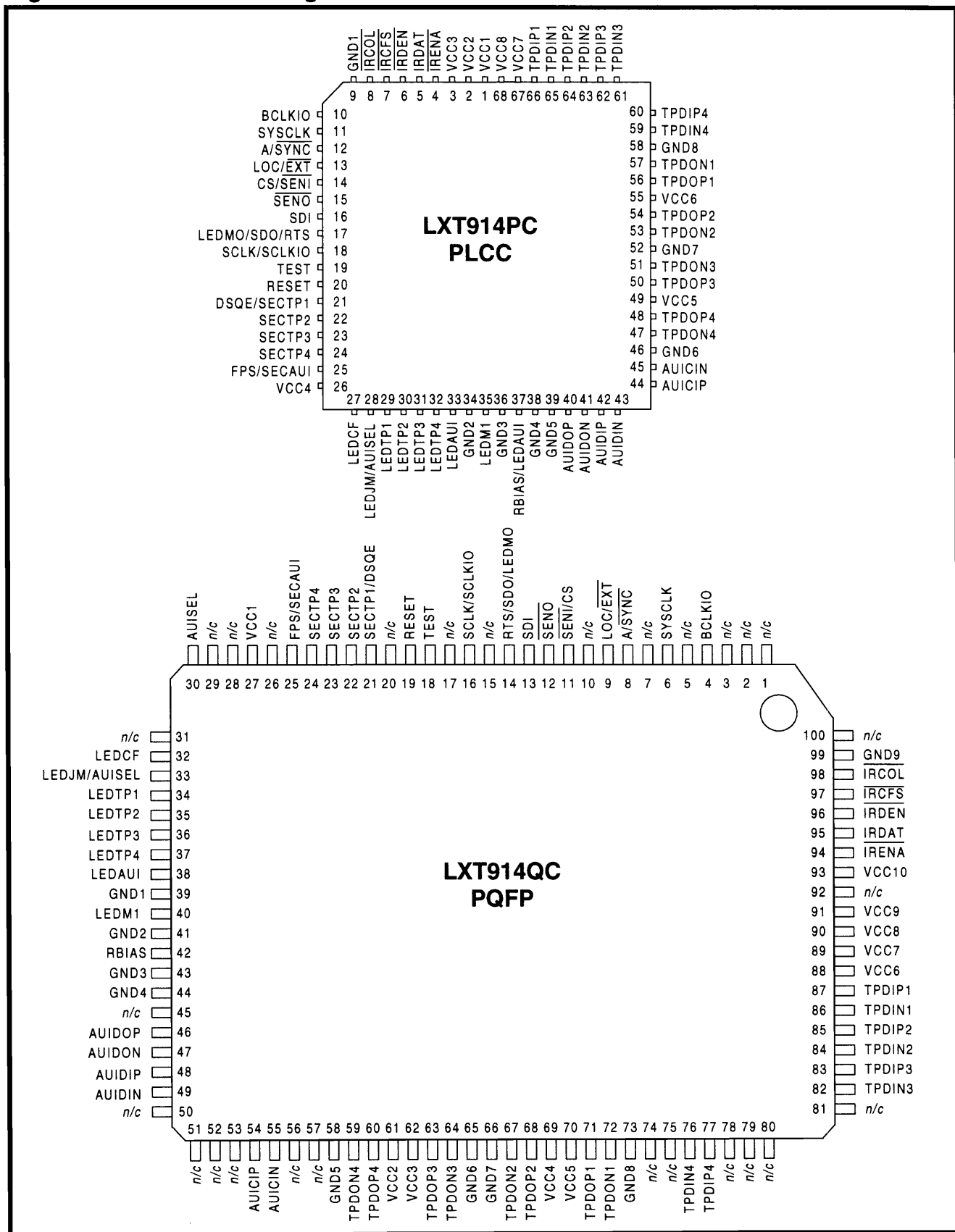
Figure 1: LXT914 Pin Assignments
