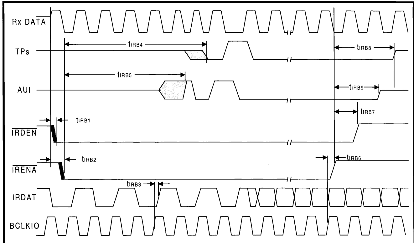
Figure 8: Inter-Repeater Bus Timing
