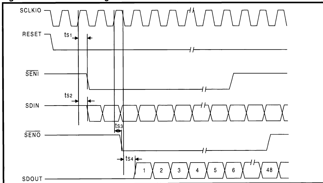
Figure 7: Serial Port Timing
