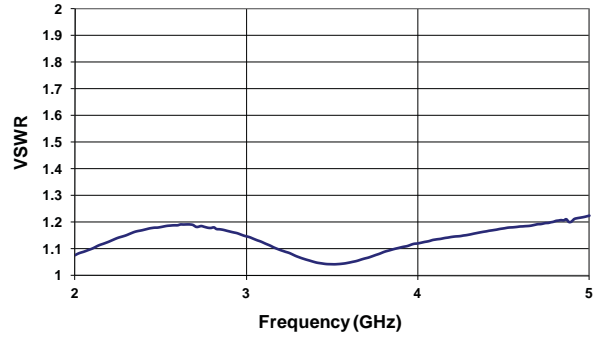
VSWR ( 2-5 GHz )
