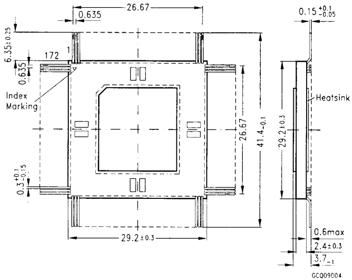
Figure 51 Ceramic-Package, C-QFP-172 (Ceramic Quad Flat Pack) "Top View"
