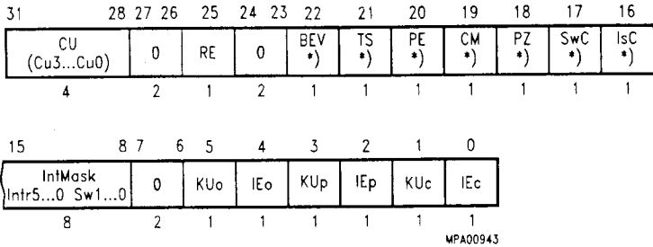
Figure 25 Status Register
