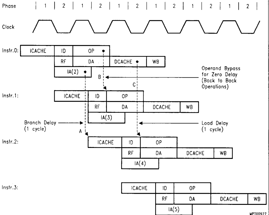
Figure 9 Instruction Pipeline Dependencies
