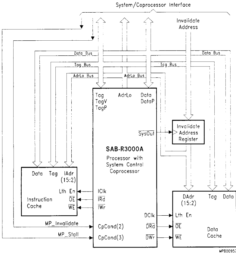
Figure 40 MP Interface Block Diagram
