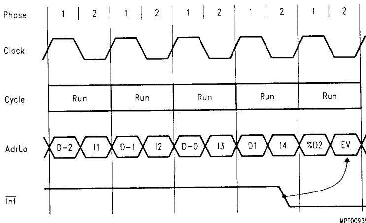
Figure 21 Interrupt Exception Latency
