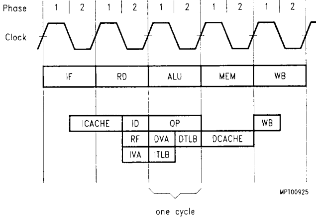
Figure 7 Execution Sequence of an Instruction
