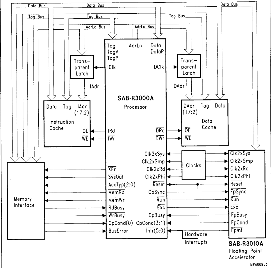
Figure 35 Solution for High-End-Computing Application
