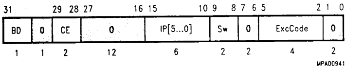
Figure 23 Cause Register
