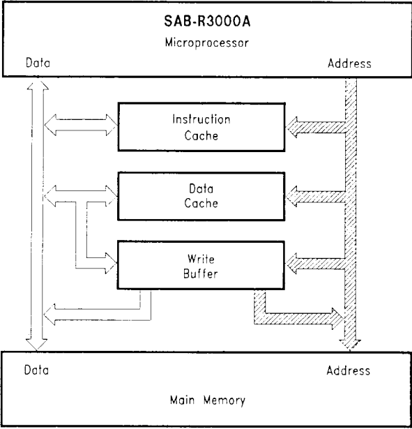
Figure 32 An SAB-R3000A System with a High-Performance Memory System
