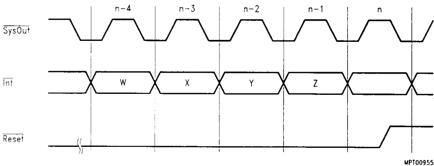
Figure 37 W, X, Y and Z Cycles on \overline{\text{Reset}} Deassertion
