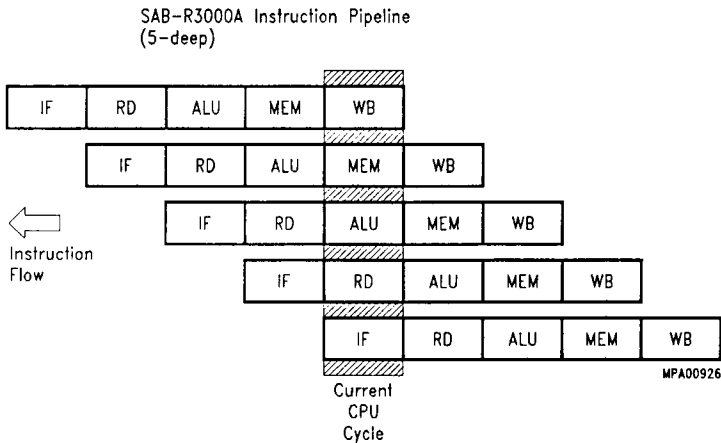
Figure 8 Overlapped execution of 5 instructions
