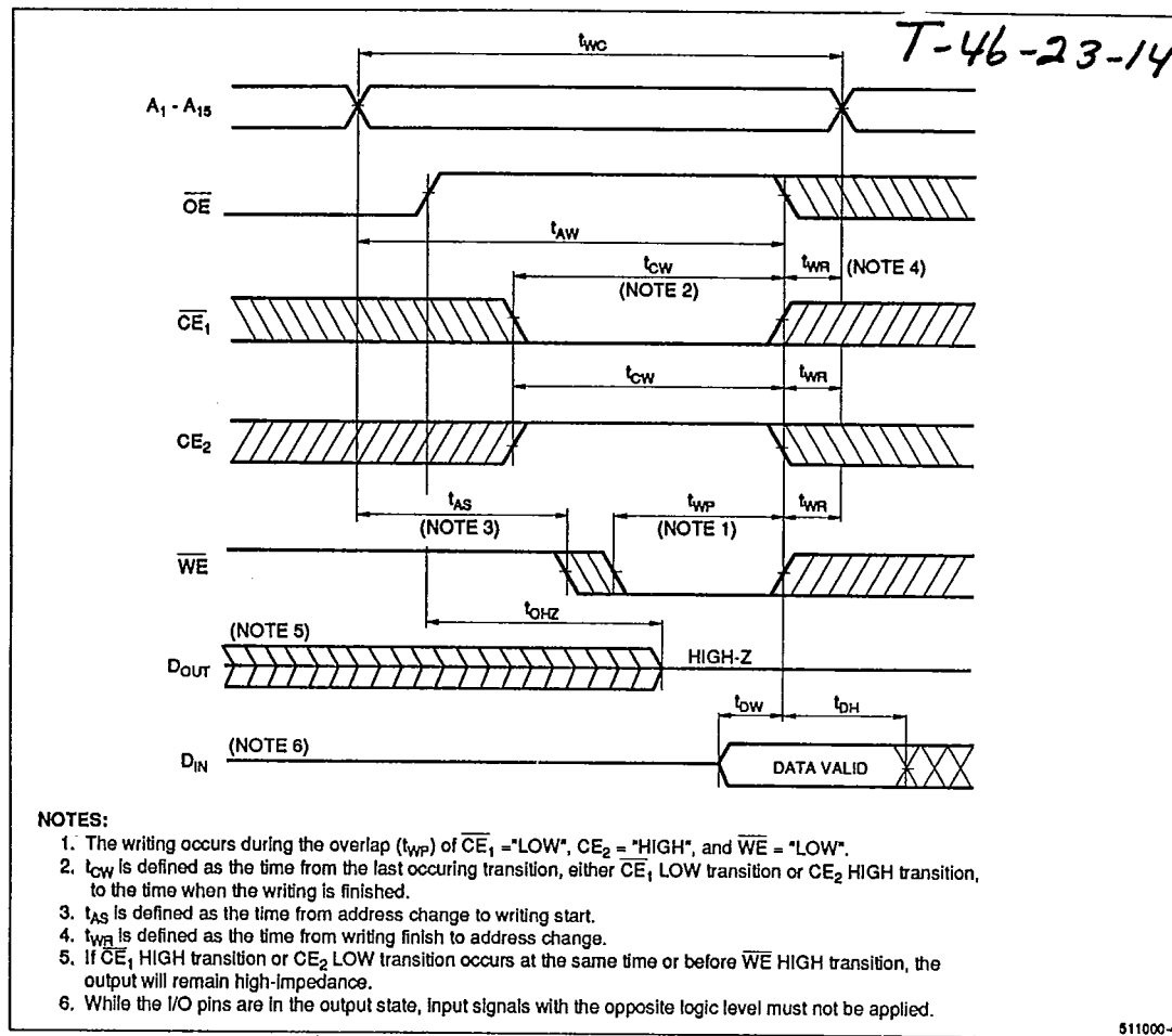
Figure 5. Write Cycle 1
