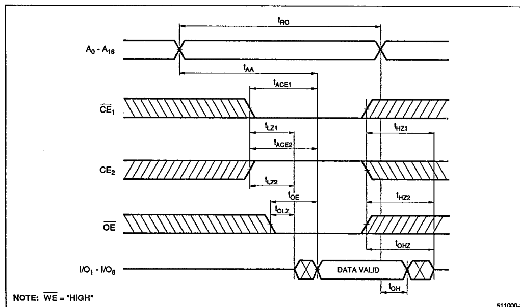
Figure 4. Read Cycle
