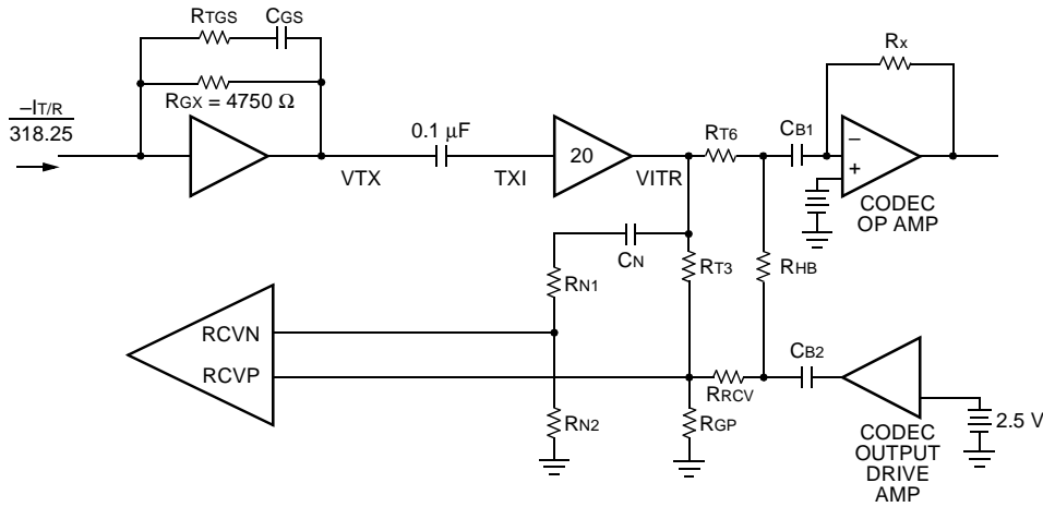
Figure 24. ac Interface Using First-Generation Codec (Including Blocking Capacitors) for Complex Termination Impedance
