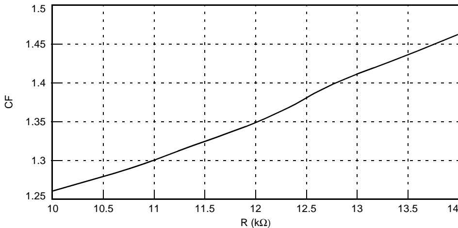
Figure 20. Crest Factor vs. R (kΩ)
