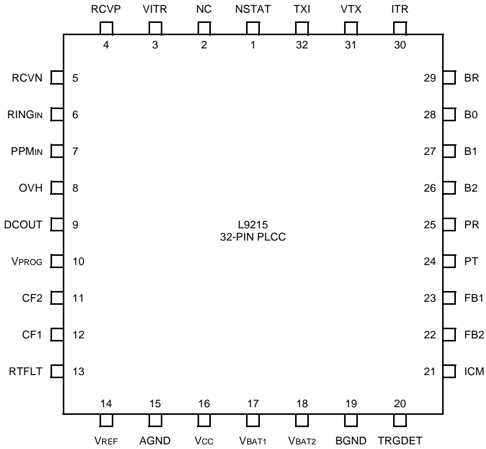
Figure 2. 32-Pin PLCC Diagram
