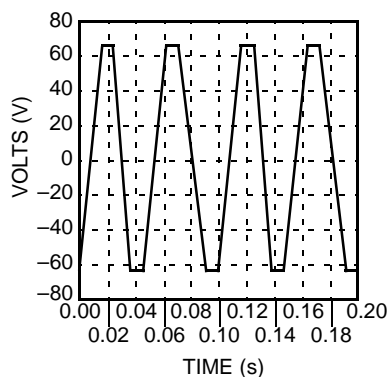
Figure 8. Ringing Waveform Crest Factor = 1.6
