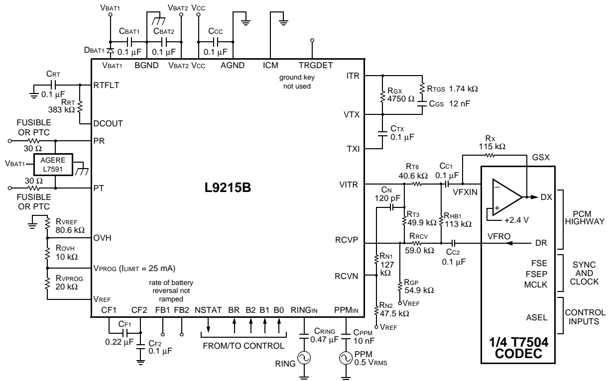
Figure 25. Agere T7504 First-Generation Codec Complex Termination; Meter Pulse Application
