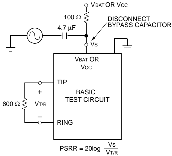
Figure 4. Metallic PSRR
