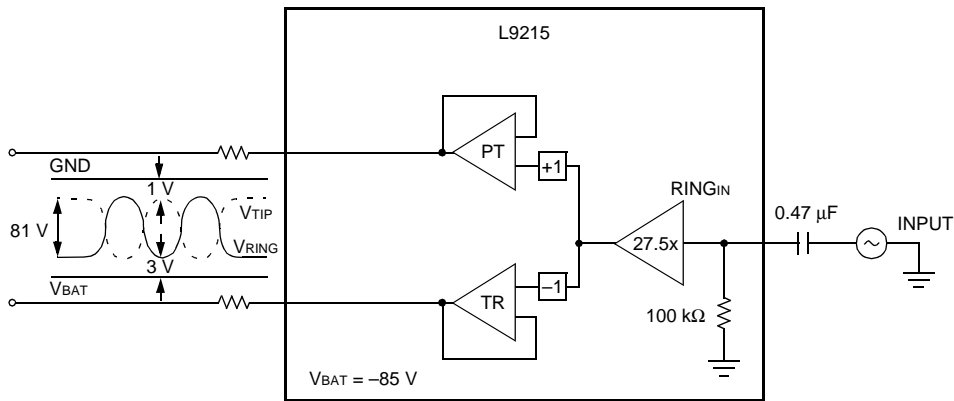
Figure 11. RINGIN Operation
