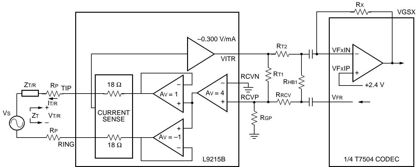
Figure 21. ac Equivalent Circuit
