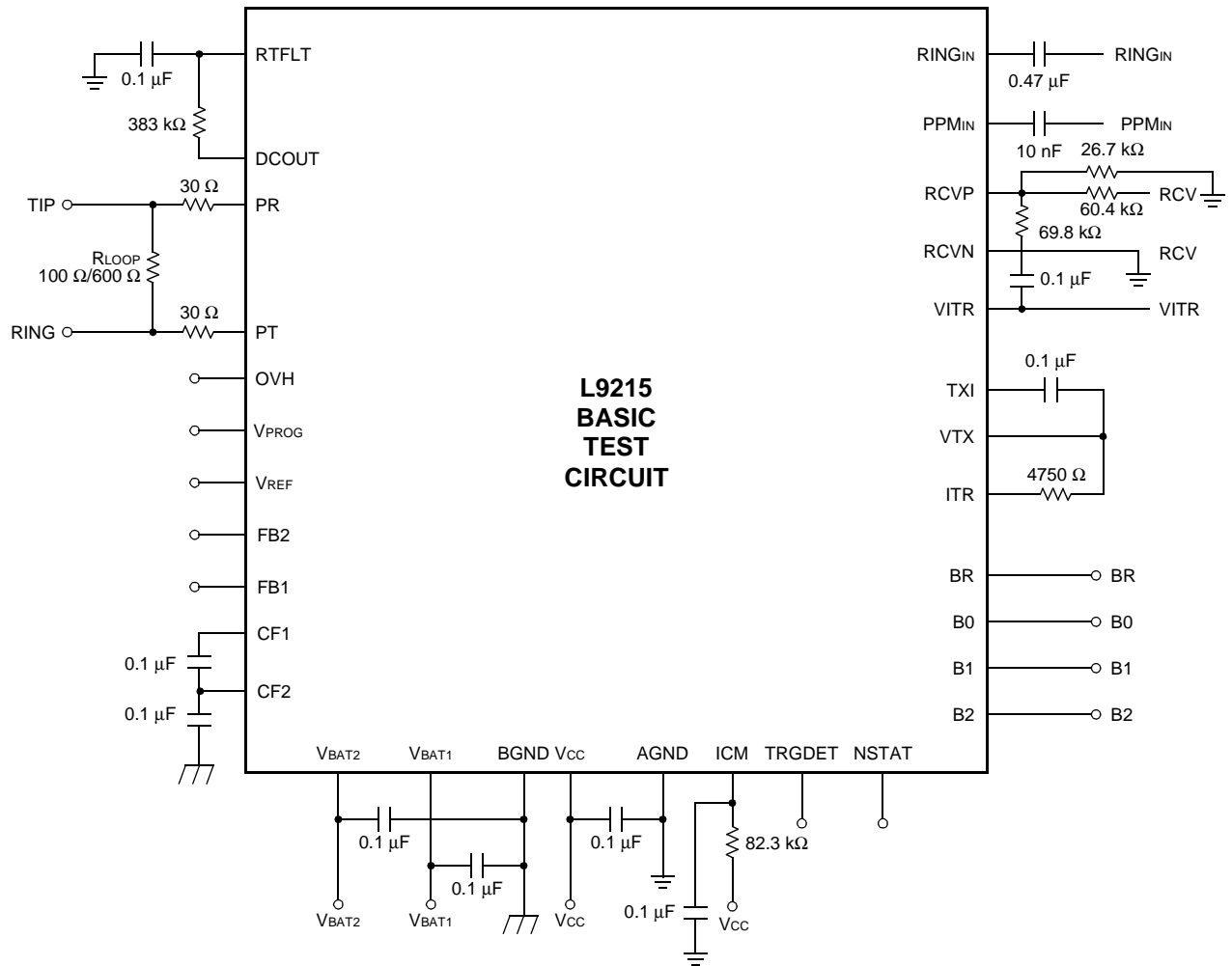
Figure 3. Basic Test Circuit
