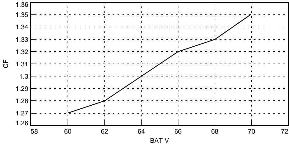
Figure 19. Crest Factor vs. Battery Voltage
