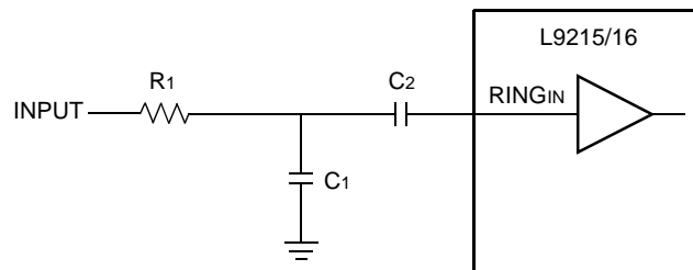
Figure 12. L9215/16 Ringing Input Circuit Selection Table for Square Wave and PWM Inputs
