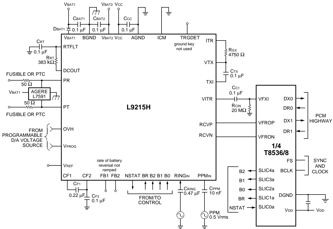
Figure 26. Third-Generation Codec ac Interface Network; Complex Termination
