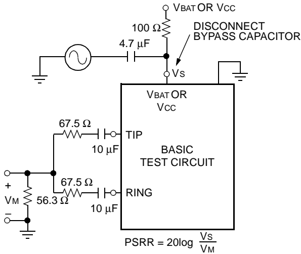
Figure 5. Longitudinal PSRR
