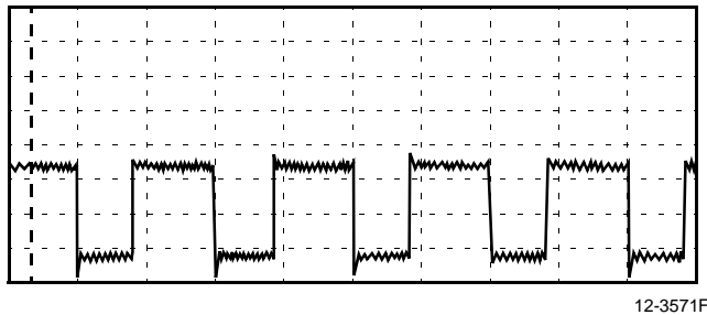
Figure 16. 3.3 V PWM Signal Amplitude
