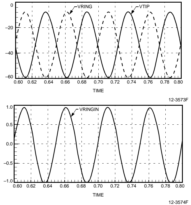
Figure 10. Ring Mode Typical Operation
