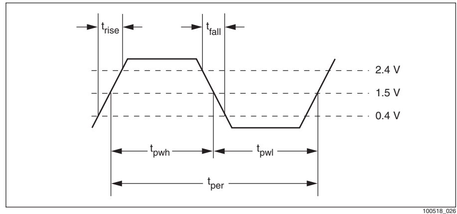
Figure 5-2. Output Waveform
