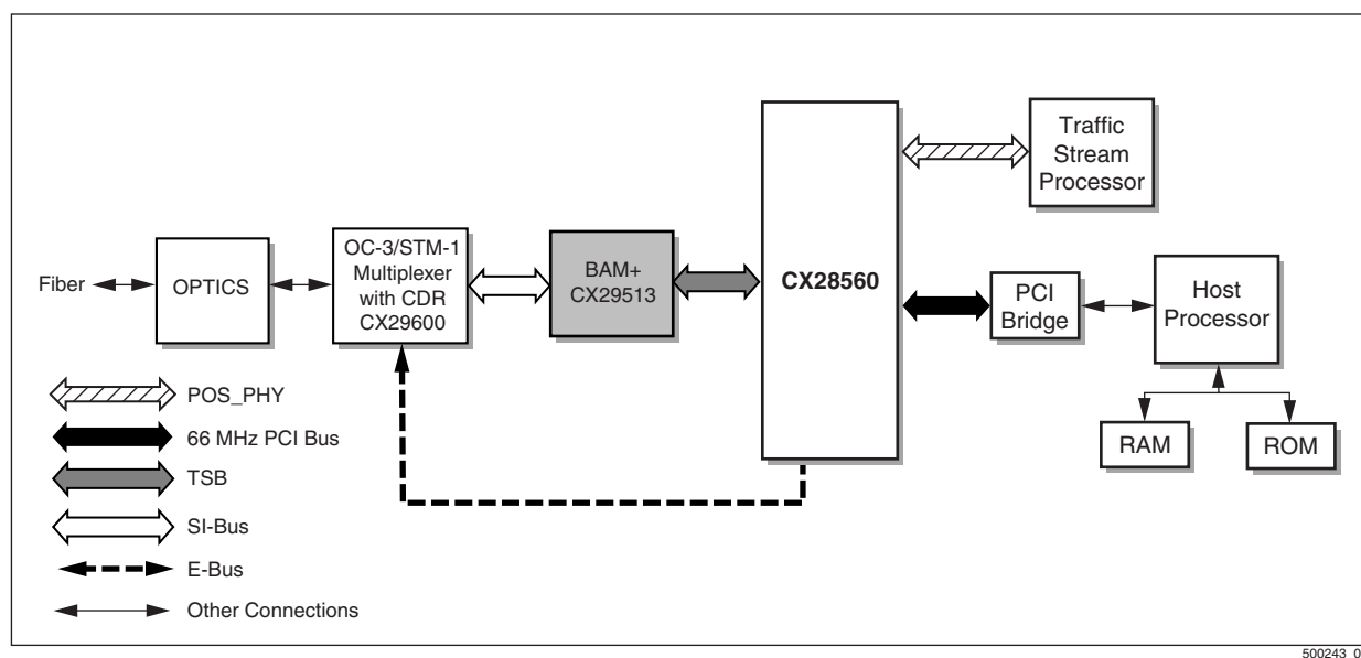
Figure 3-1. OC-3/STM-1 Full DS0/E0 Channelization Application
