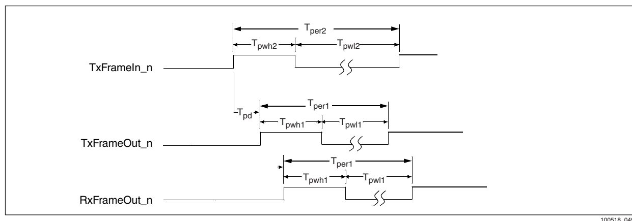
Figure 5-13. Frame Reference Timing Diagram
