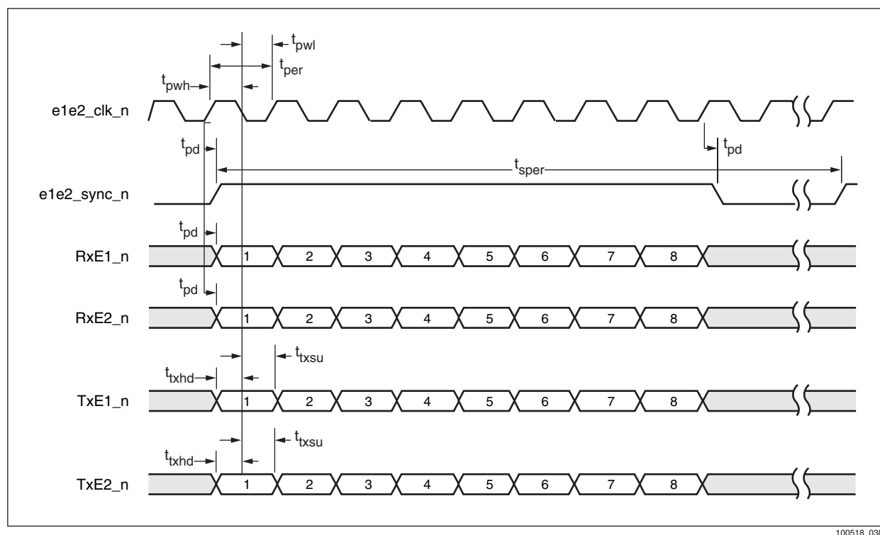
Figure 5-15. E1/E2 Timing Diagram
