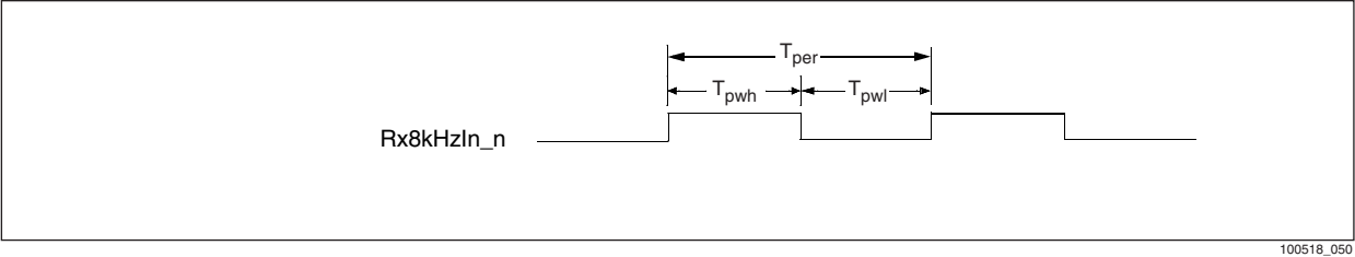
Figure 5-14. Rx8kHz Timing Diagram
