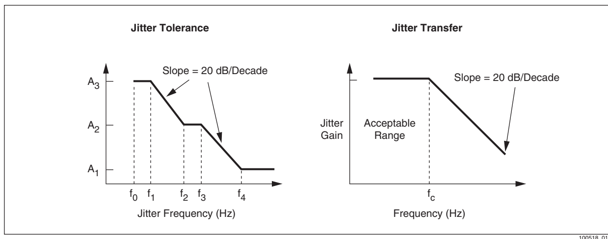
Figure 2-7. Bellcore GR-253-CORE Jitter Specifications
