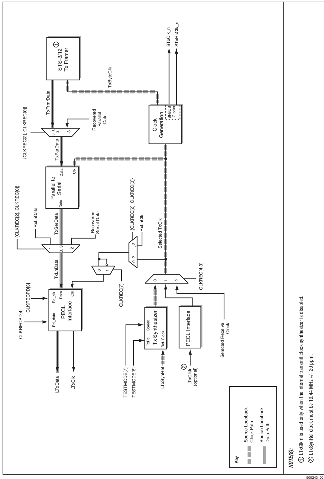
Figure 2-32. Source Loopback—Transmit
