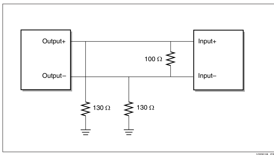
Figure 2-24. PECL Bias Network
