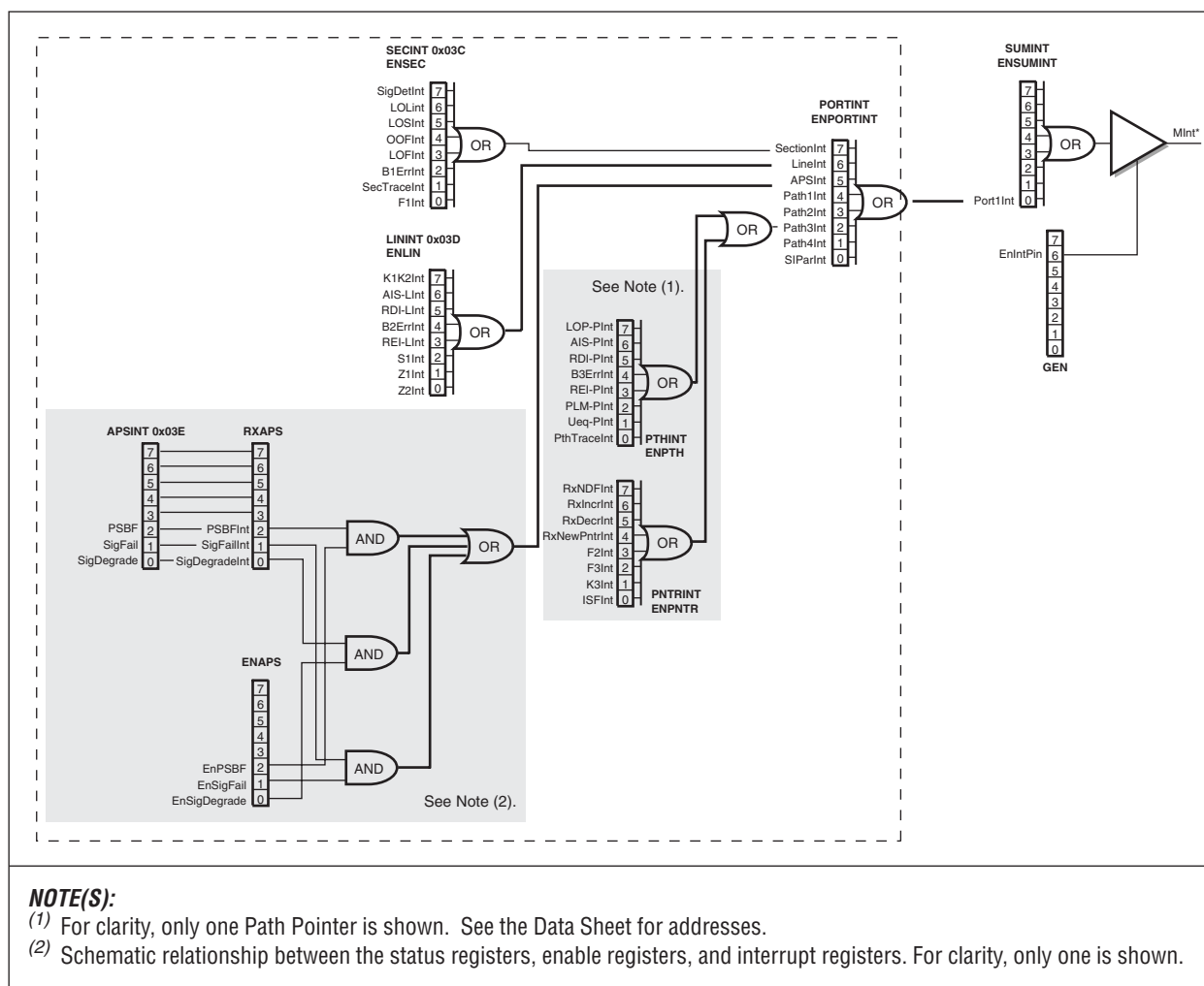
Figure 2-17. Interrupt Hierarchy
