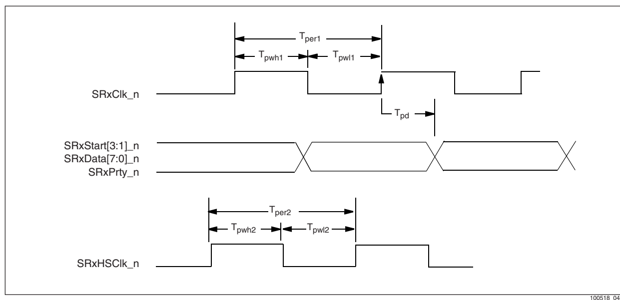
Figure 5-8. Receive Timing Parameters
