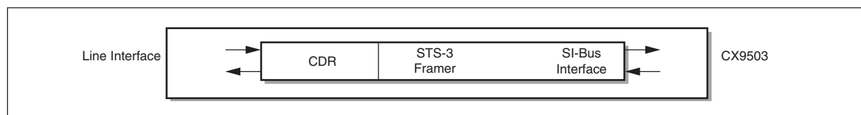
Figure 1-4. 4xSTS-3 Mode Data Flow Diagram
