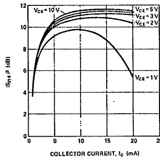
Figure 11. Typical |S_{21E}|^2 vs. Collector Current at 1000 MHz, for the HSMX-3635.
