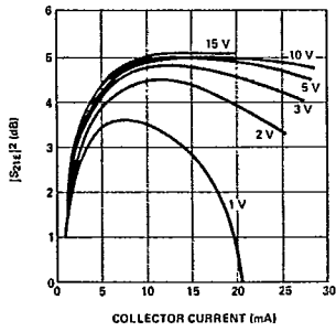
Figure 14. Typical |S_{21}|^2 vs. Collector Current at 4000 MHz, for the HXTR-3675.
