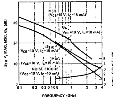
Figure 6. Typical |S_{21E}|^2 , MAG, MSG, G_A , Noise Figure, and G_A vs. Frequency, for the HSMX-3655.
