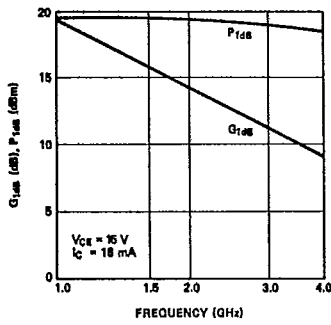
Figure 25. Typical Power Output at 1 dB Compression Gain vs. Frequency, for the HXTR-7111.
