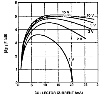
Figure 9. Typical |S_{21E}|^2 vs. Collector Current at 4000 MHz, for the HXTR-7111.
