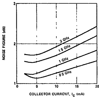
Figure 19. Typical Noise Figure vs. Collector Current, V_{CE} = 10 V, for the HSMX-3655.
