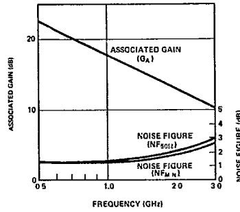
Figure 23. Typical Noise Figure and Associated Gain vs. Frequency at V_{CE} = 10\text{ V} , I_C = 10\text{ mA} , for the HXTR-3645.
