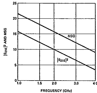
Figure 2. Typical |S 21E | 2 and Maximum Stable Gain (MSG) vs. Frequency at V CE = 10 V and I C = 10 mA, for the HXTR-7111.
