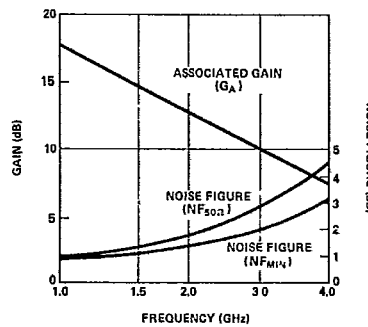
Figure 21. Typical Noise Figure and Associated Gain vs. Frequency at V_{CE} = 10 V, I_C = 10 mA, for the HXTR-7111.
