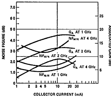
Figure 16. Typical NF_{MIN} and Associated Gain ( G_A ) vs. Collector Current at V_{CE} = 10 V, for the HXTR-7111.
