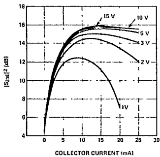
Figure 10. Typical |S_{21E}|^2 vs. Collector Current at 1000 MHz, for the HXTR-3615.
