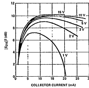
Figure 12. Typical |S_{21E}|^2 vs. Current at 2000 MHz, for the HXTR-3645.
