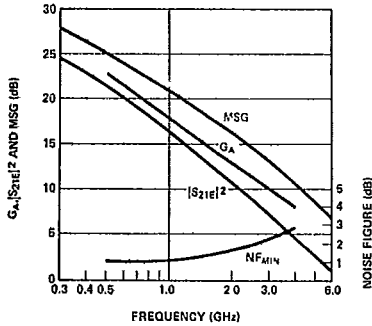
Figure 1. Typical NF min , GA, |S 21E | 2 and MSG vs. Frequency at V CE = 10 V, I C = 10 mA for the HXTR-7011.
