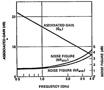
Figure 22. Typical NF_{MIN} and Associated Gain vs. Frequency at V_{CE} = 10\text{ V} , I_C = 10\text{ mA} , for the HXTR-3615.
