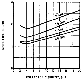
Figure 17. Typical Noise Figure vs. Collector Current, V_{CE} = 10 V, for the HSMX-3635.
