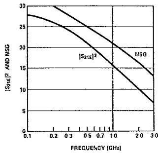
Figure 5. Typical |S_{21E}|^2 and Maximum Stable Gain (MSG) vs. Frequency at V_{CE} = 10 V and I_C = 10 mA, for the HXTR-3645.
