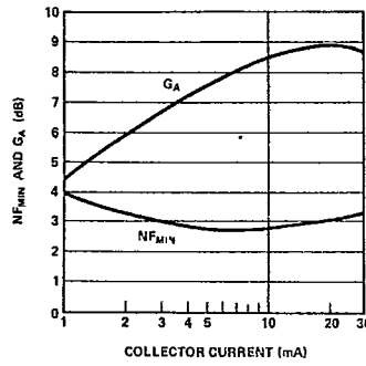
Figure 15. Typical NF_{MIN} and Associated Gain vs. I_C at 4 GHz for V_{CE} = 10 V, for the HXTR-7011.
