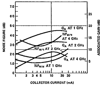
Figure 20. Typical NF_{MIN} and Associated Gain ( G_A ) vs. Collector Current at V_{CE} = 10 V, for the HXTR-3675.
