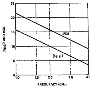
Figure 7. Typical |S_{21E}|^2 and Maximum Stable Gain (MSG) vs. Frequency at V_{CE} = 10 V and I_C = 10 mA, for the HXTR-3675.
