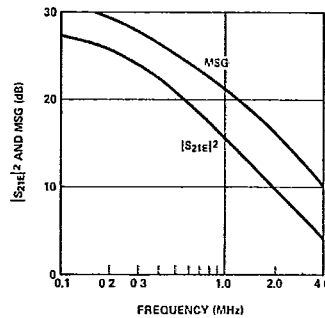
Figure 3. Typical |S 21E | 2 and Maximum Stable Gain (MSG) vs. Frequency at V CE = 10 V and I C = 10 mA, for the HXTR-7111.
