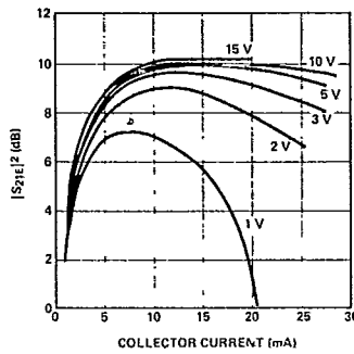
Figure 8. Typical |S_{21E}|^2 vs. Collector Current at 2000 GHz, for the HXTR-7011.
