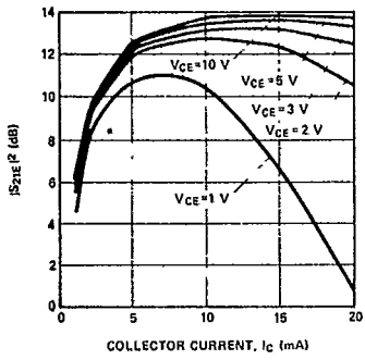
Figure 13. Typical |S_{21}|^2 vs. Collector Current at 1 GHz, for the HSMX-3655.
