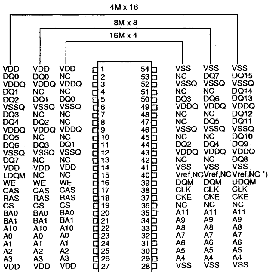
TSOPII-54 (10.16 mm x 22.22 mm, 0.8 mm pitch)
