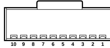
BOTTOM VIEW (HSDL-3612-008/-038)
