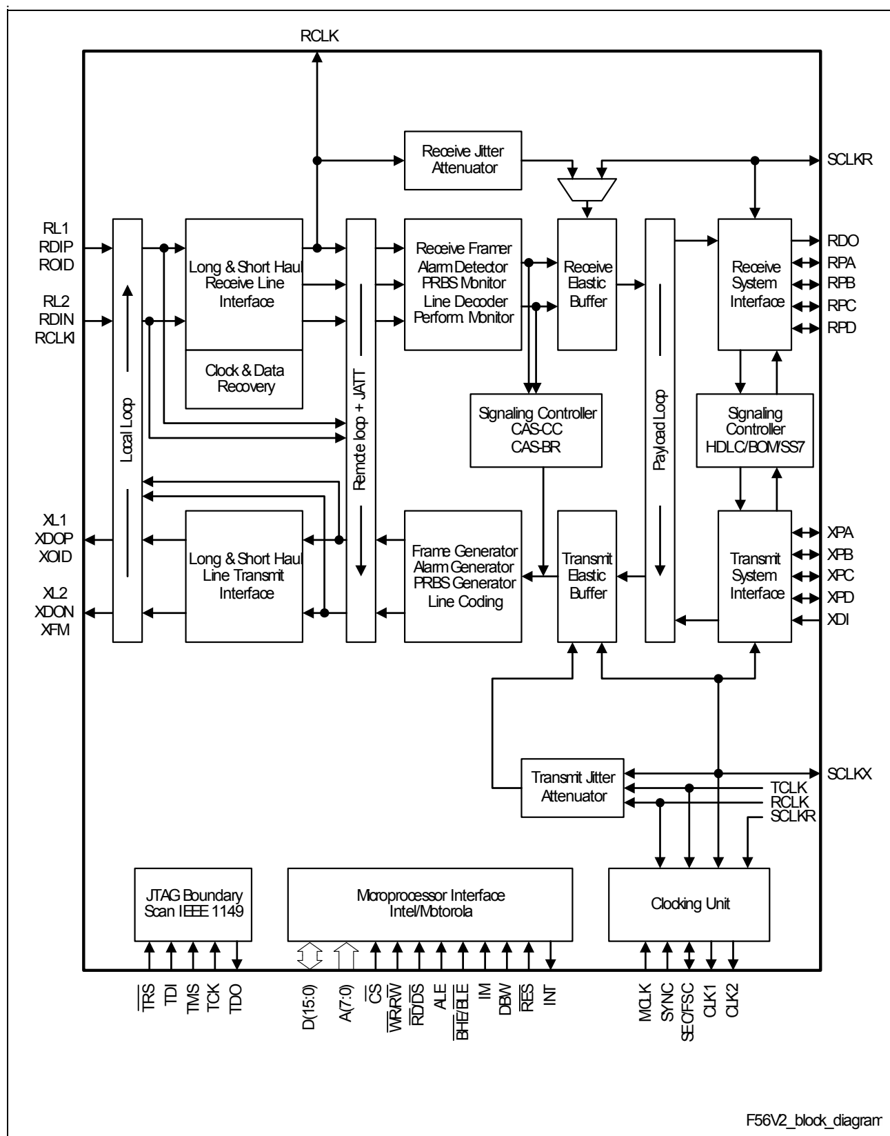
Figure 6 Block Diagram
