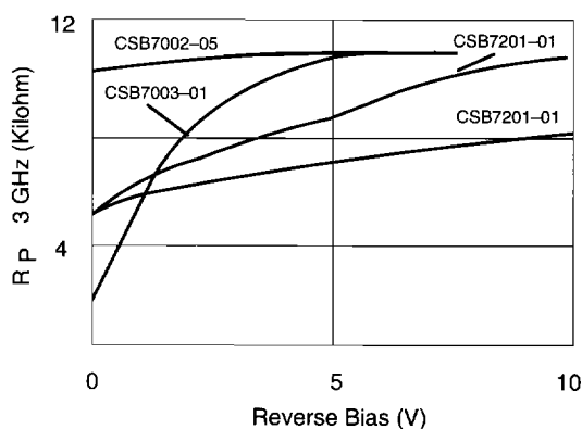
Figure 5. Parallel Resistance vs. Bias
