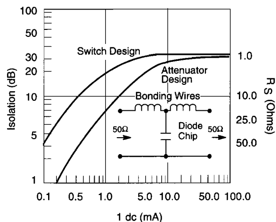
Figure 6. General Curves of Isolation and R_S vs. Bias for Attenuator and Switch Designs
