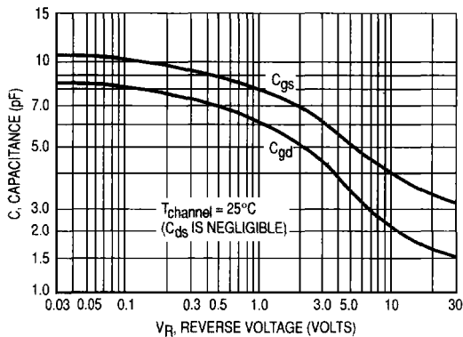
Figure 7. Typical Capacitance
