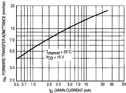
Figure 6. Typical Forward Transfer Admittance
