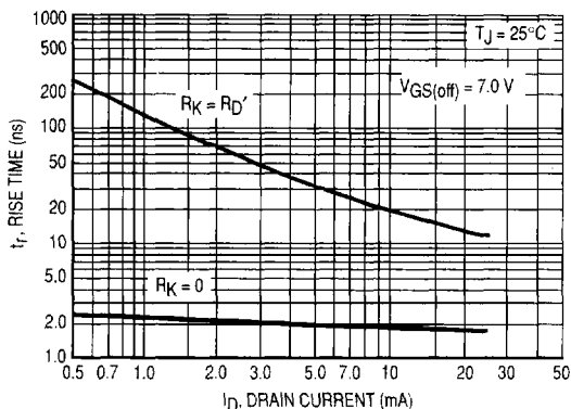
Figure 2. Rise Time
