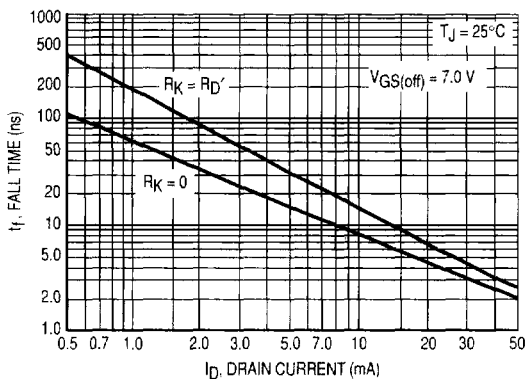
Figure 4. Fall Time
