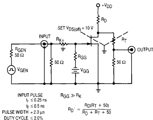
Figure 5. Switching Time Test Circuit
