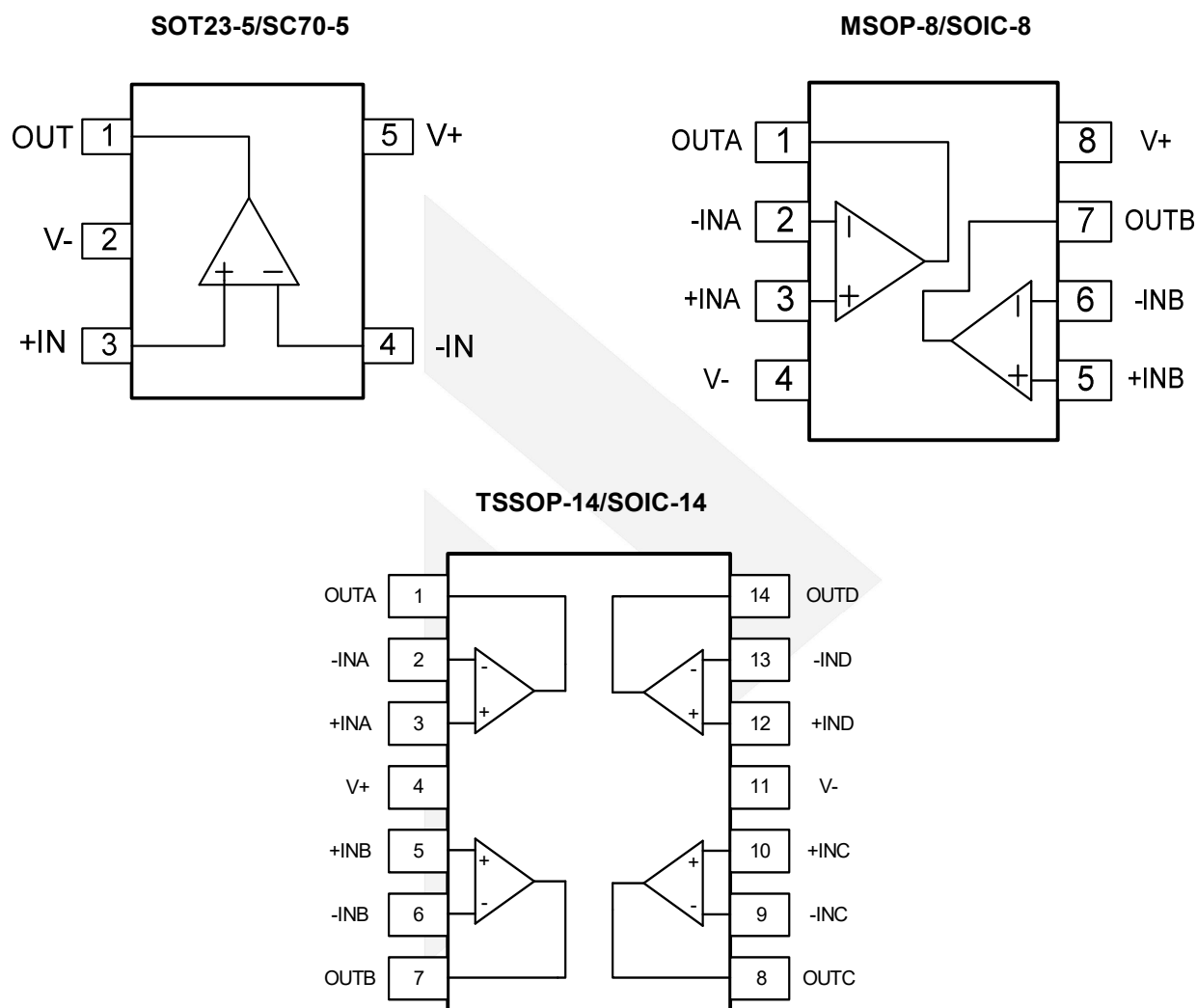
Figure 1 Pin Assignment (Top View)
