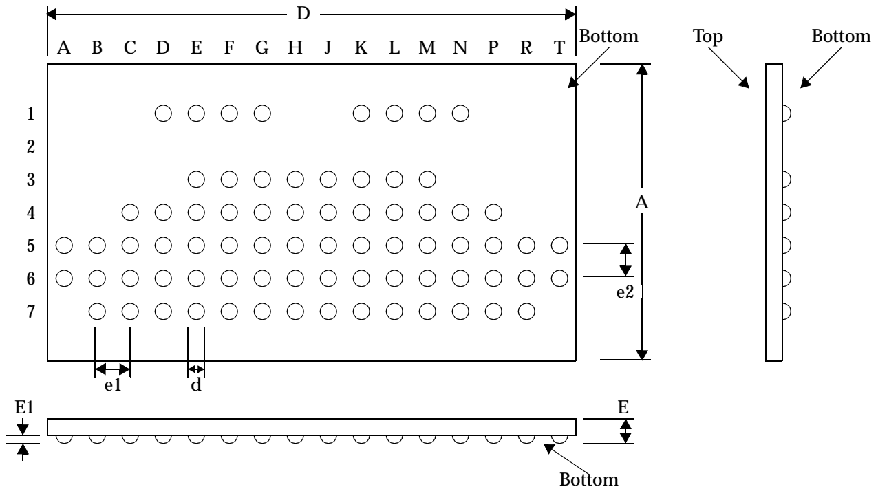
Figure 62: Edge-Bonded uBGA Package
