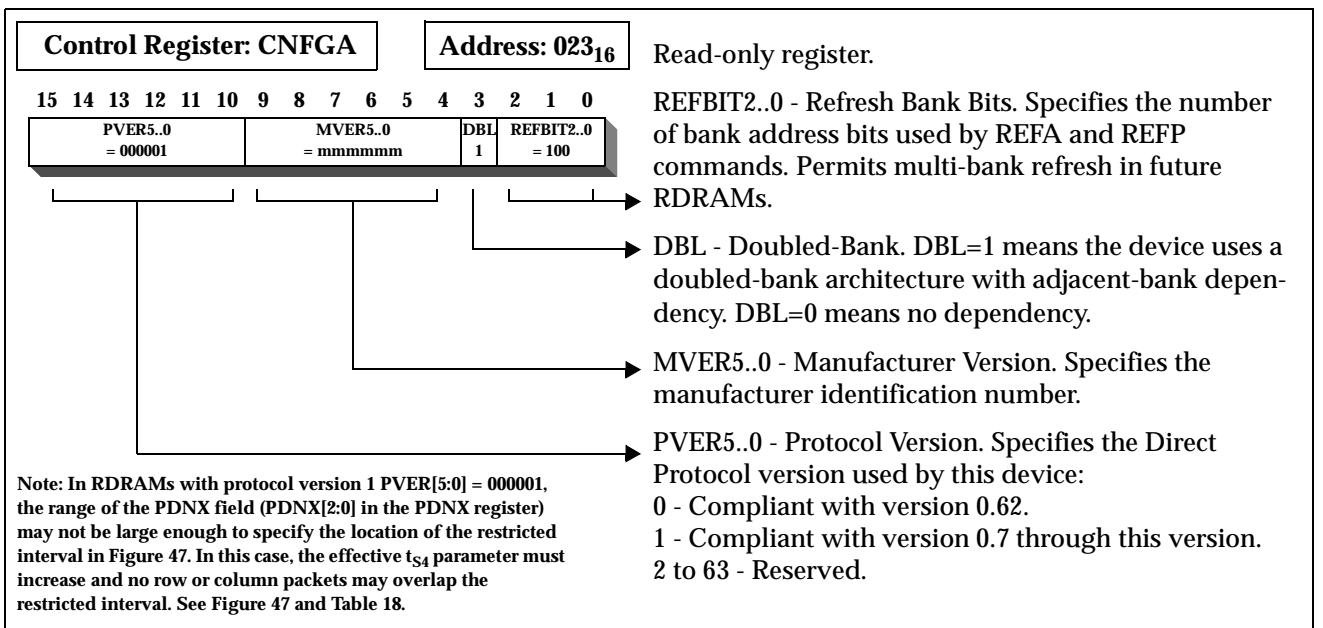
Figure 28: CNFGA Register
