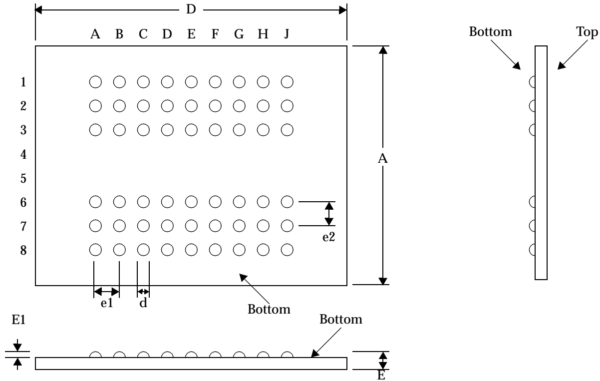
Figure 63: Center-Bonded uBGA Package
