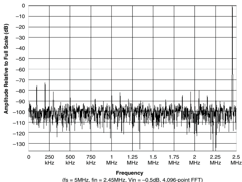
Figure 5. FFT Analysis of ADS-118
