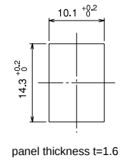
◆Mounting Hole Dimensions Diagram
