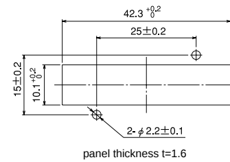
◆Mounting Hole Dimensions Diagram
