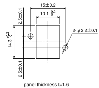
◆Mounting Hole Dimensions Diagram
