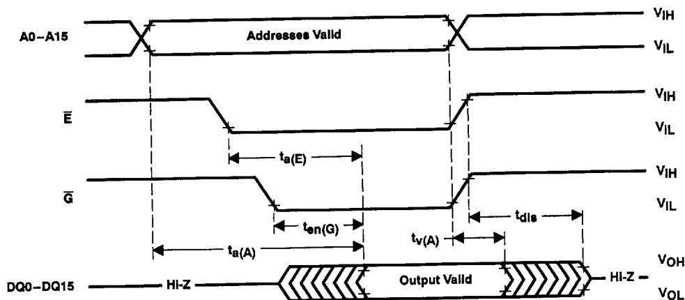
Figure 3. Read-Cycle Timing
