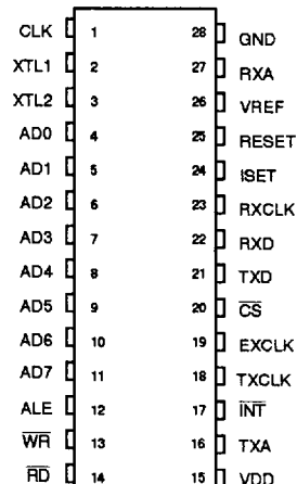
600-Mil 28-Pin DIP
