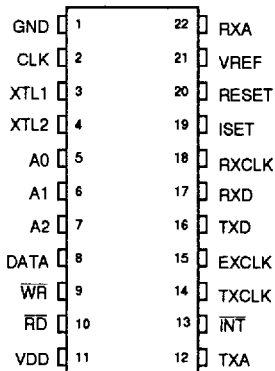
400-Mil 22-Pin DIP
