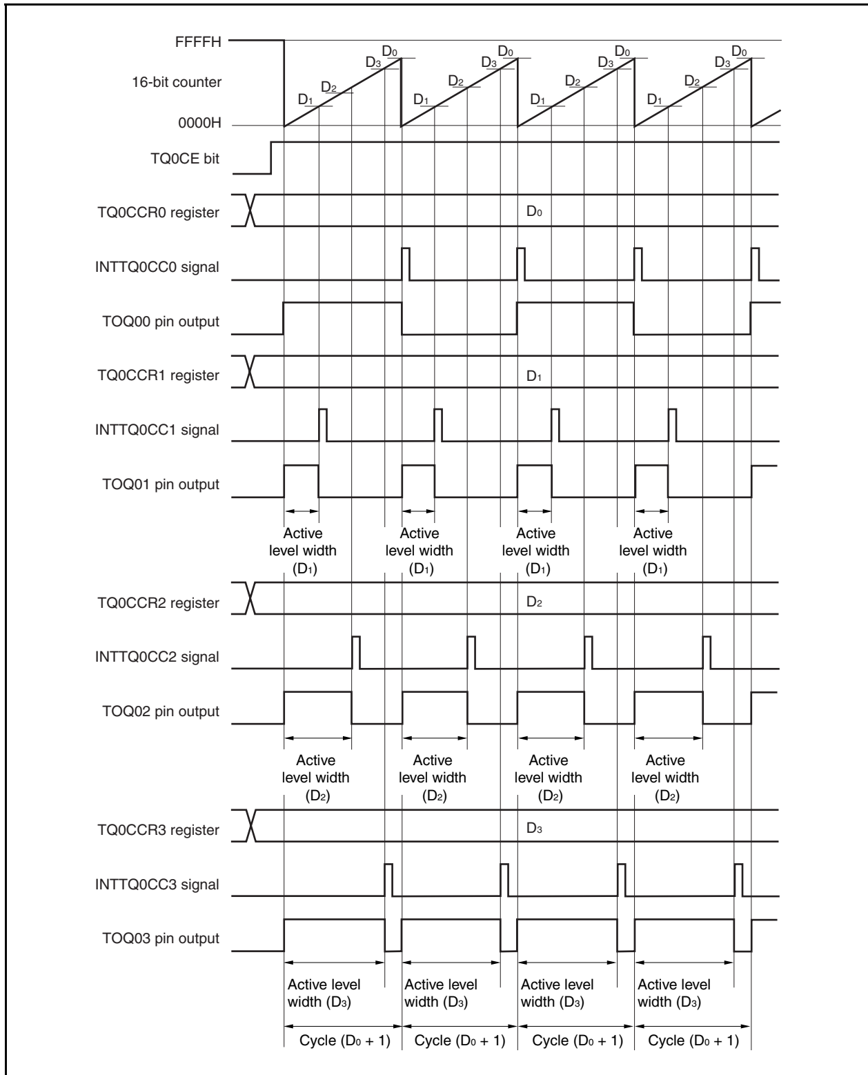
Figure 7-30. Basic Timing in PWM Output Mode
