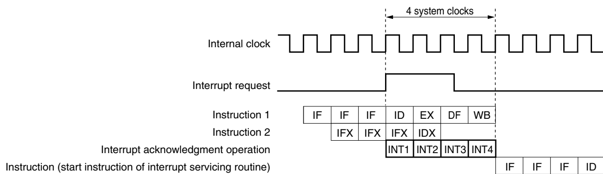
Figure 17-14. Pipeline Operation at Interrupt Request Acknowledgment (Outline)
