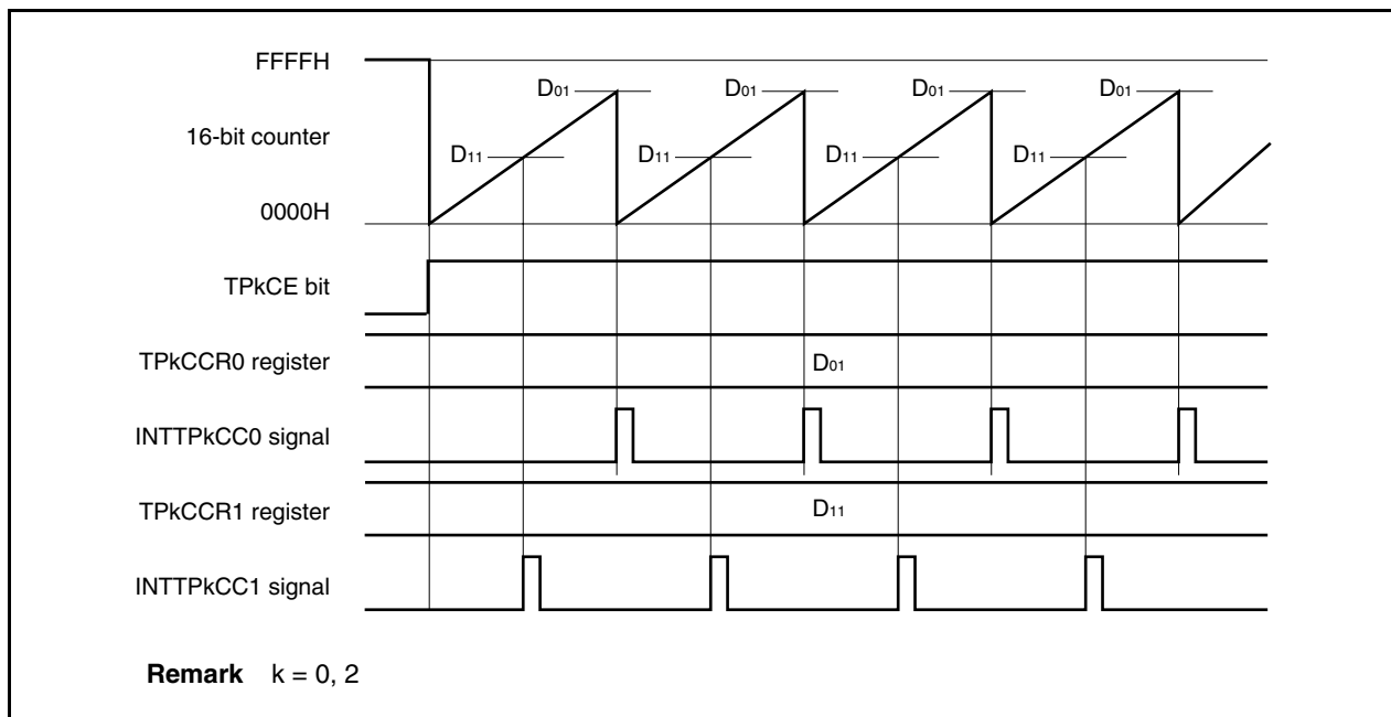
Figure 6-21. Timing Chart When D_{01} \geq D_{11}
