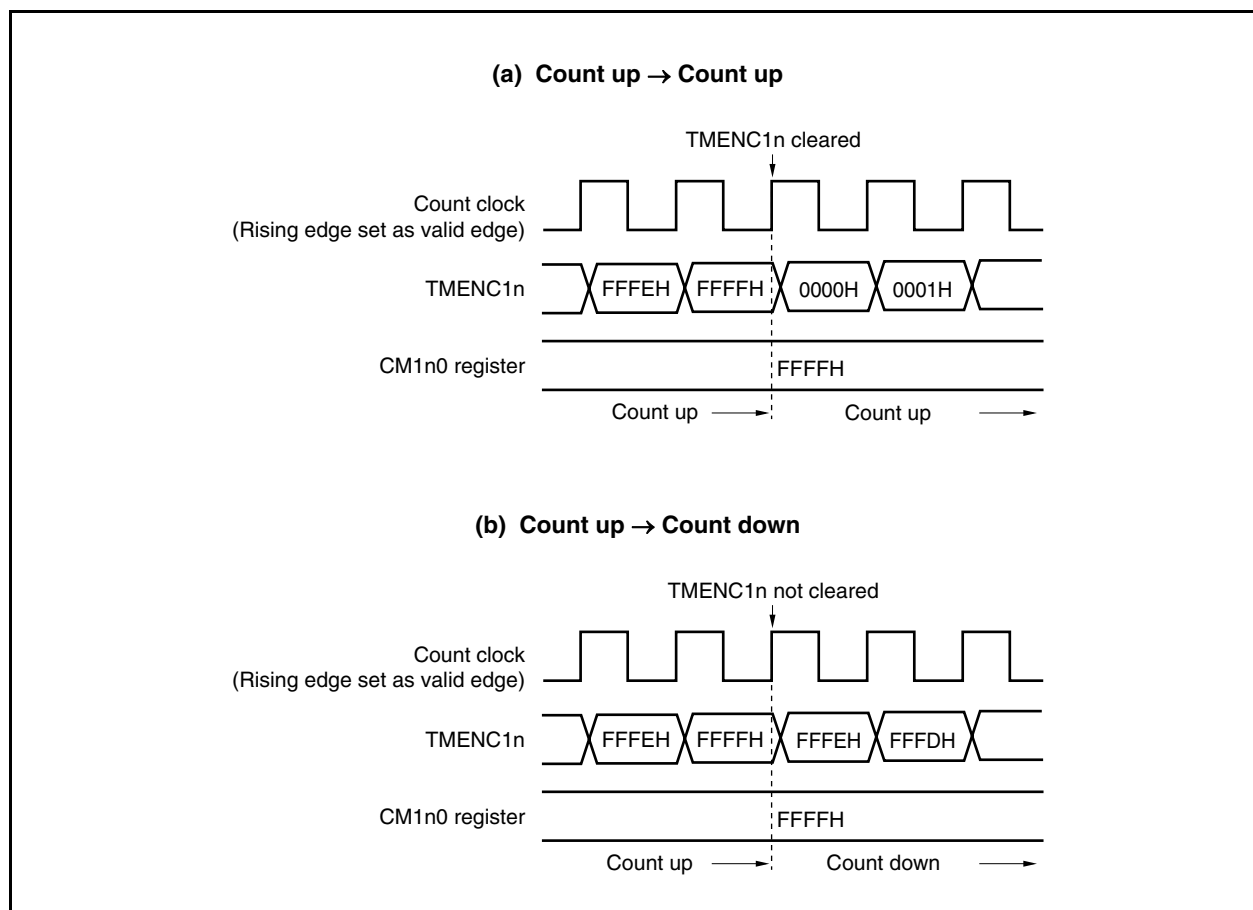
Figure 8-12. Clear Operation After Match of CM1n0 Register Set Value and TMENC1n Count Value
