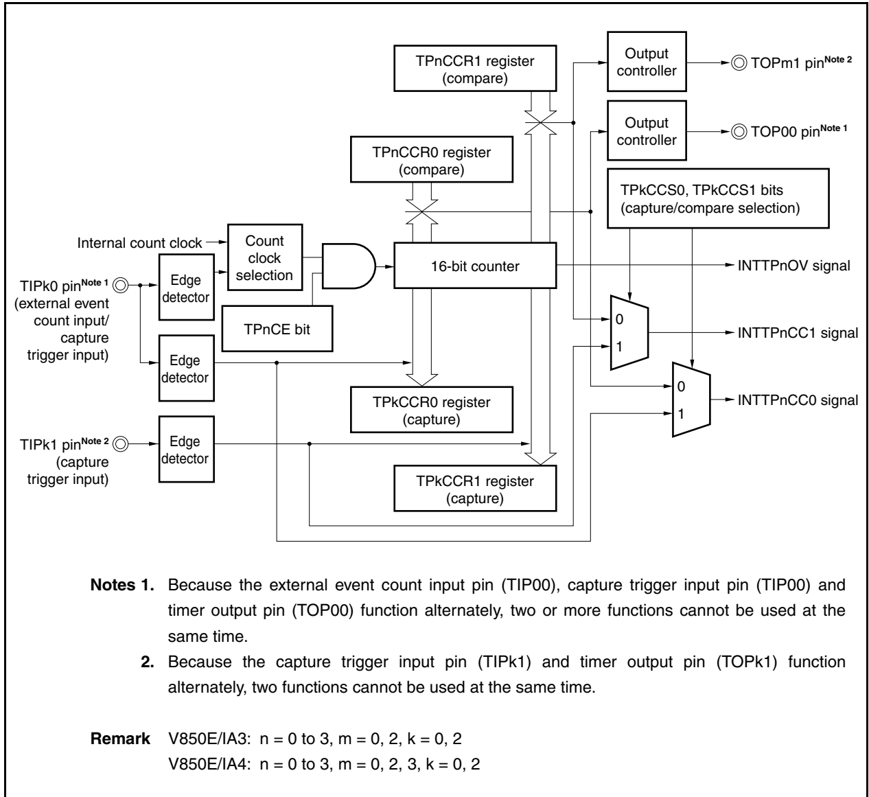
Figure 6-35. Configuration in Free-Running Timer Mode
