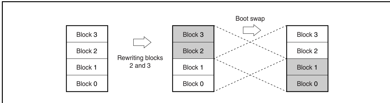
Figure 22-13. Rewriting Entire Memory Area (Boot Swap)
