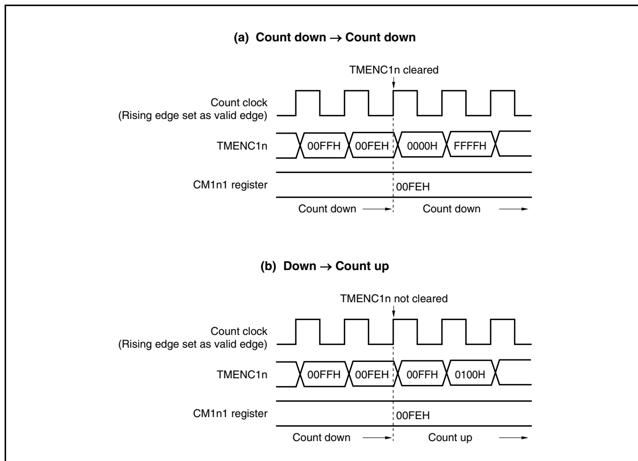
Figure 8-13. Clear Operation After Match of CM1n1 Register Set Value and TMENC1n Count Value
