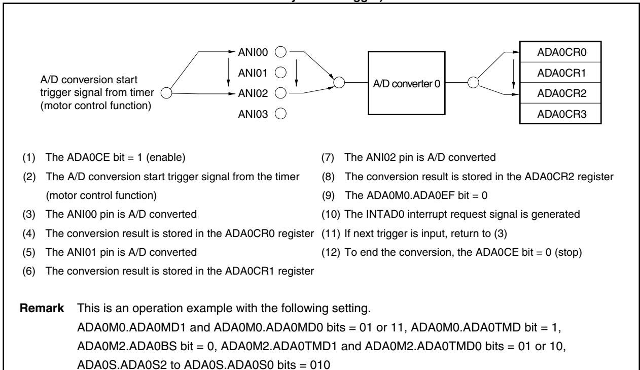
Figure 12-19. Example of Scan Mode Operation (Continuous Scan/ One-Shot Scan by Timer Trigger): V850E/IA4
