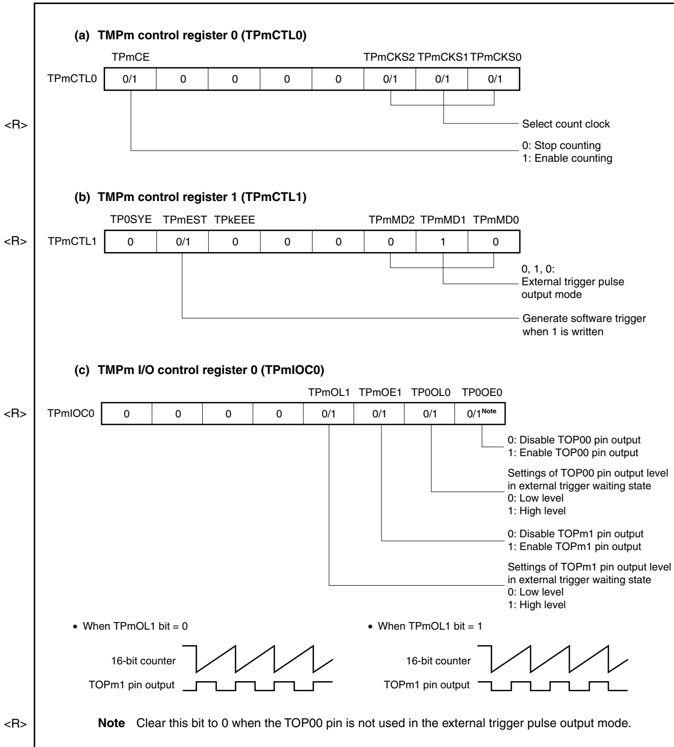
Figure 6-25. Setting of Registers in External Trigger Pulse Output Mode (1/2)
