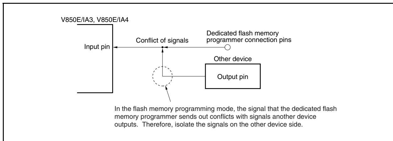
Figure 22-9. Conflict of Signals (Serial Interface Input Pin)
