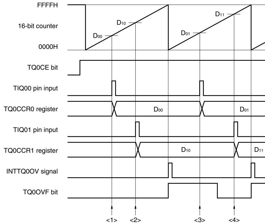
Example of incorrect processing when two or more capture registers are used
