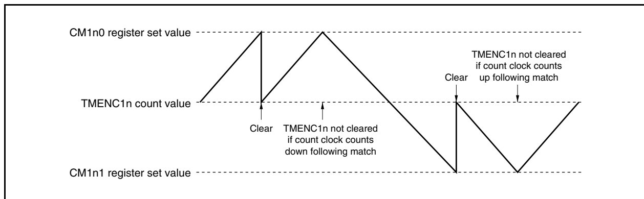
Figure 8-11. Example of TMENC1n Operation in UDC Mode
