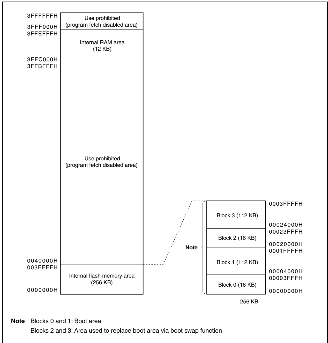
Figure 22-1. Flash Memory Mapping
