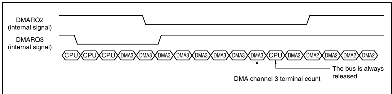
Figure 16-7. Block Transfer Example
