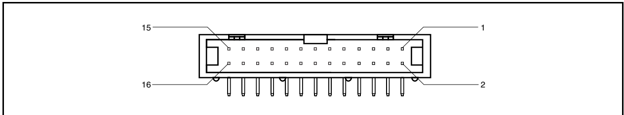
Figure 22-3. Target Connector Outline (Viewed from Connector Insertion Side)
