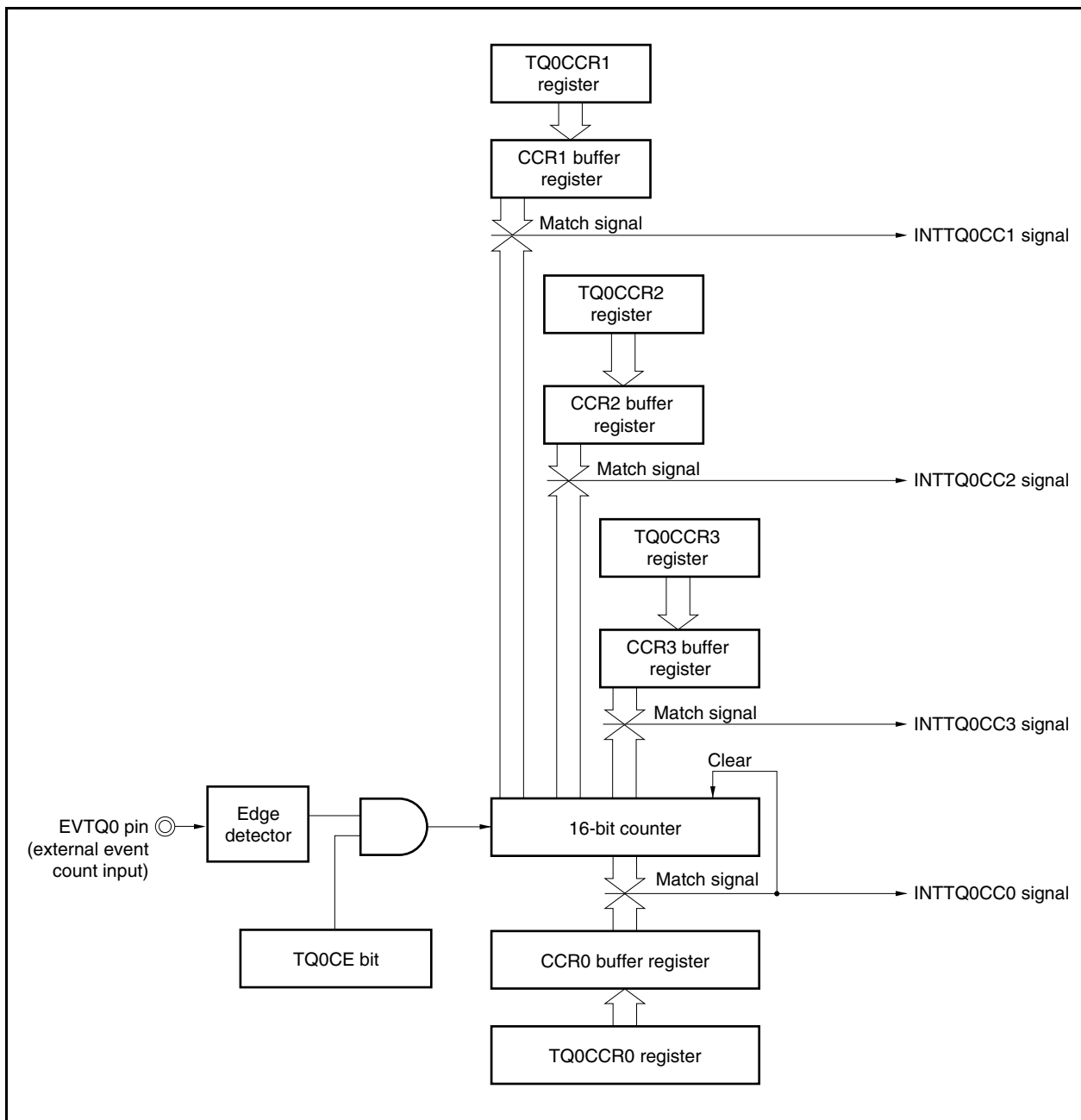
Figure 7-18. Configuration of TQ0CCR1 to TQ0CCR3 Registers
