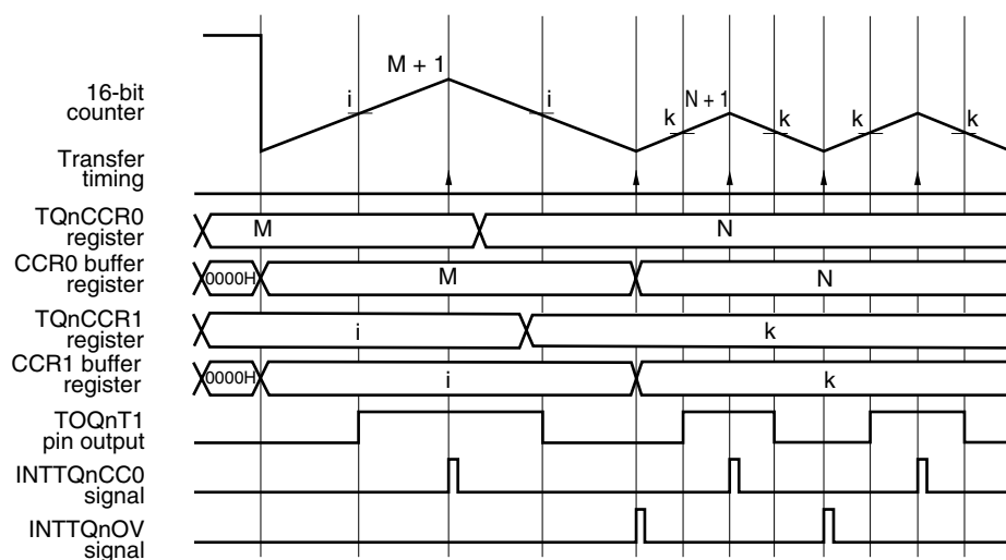
Figure 10-29. Example of Rewriting TQnCCR0 Register (During Counting Down)
