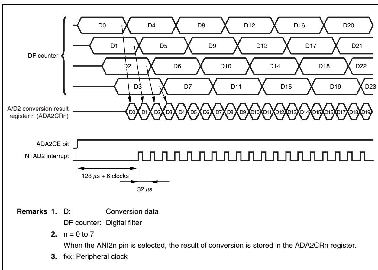
Figure 13-5. Example of Operation Timing in 1-Buffer Parallel Mode (with 8-Bit Resolution, f xx = 64 MHz)
