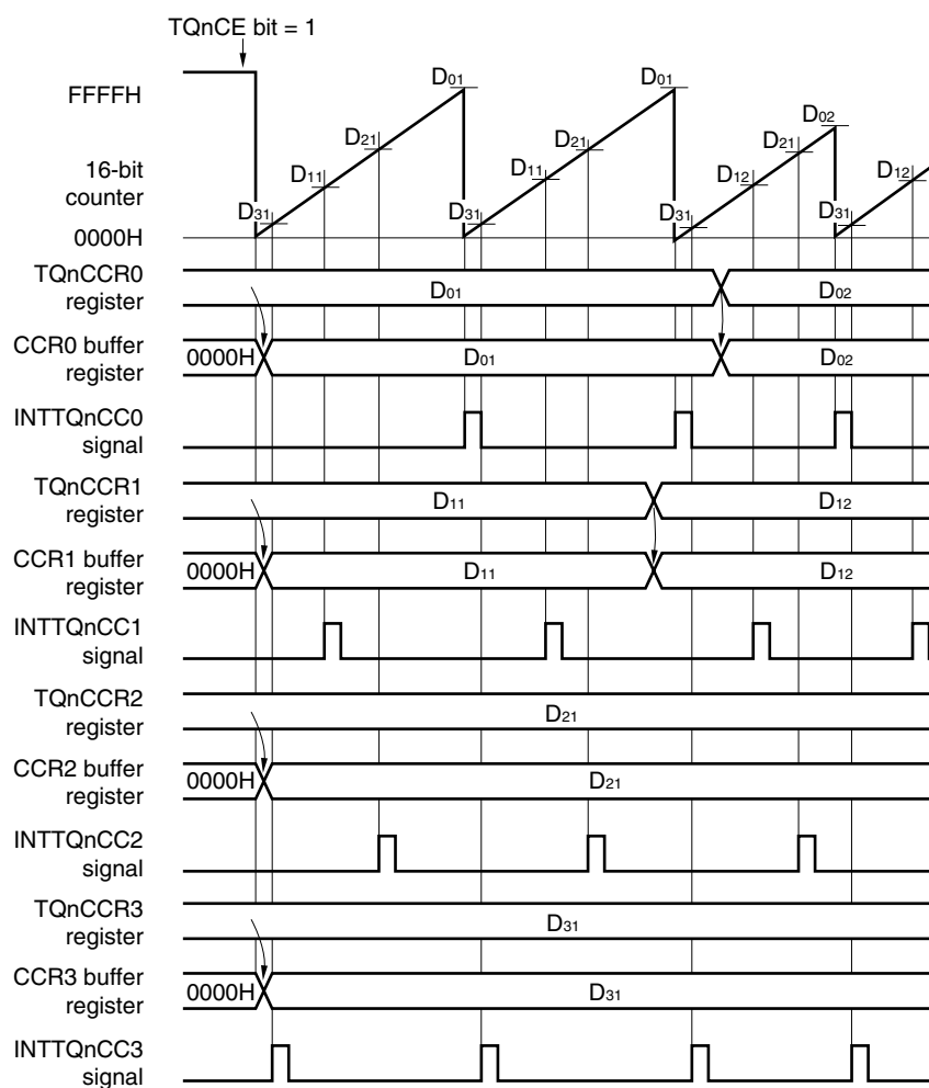
Figure 7-4. Timing of Anytime Write
