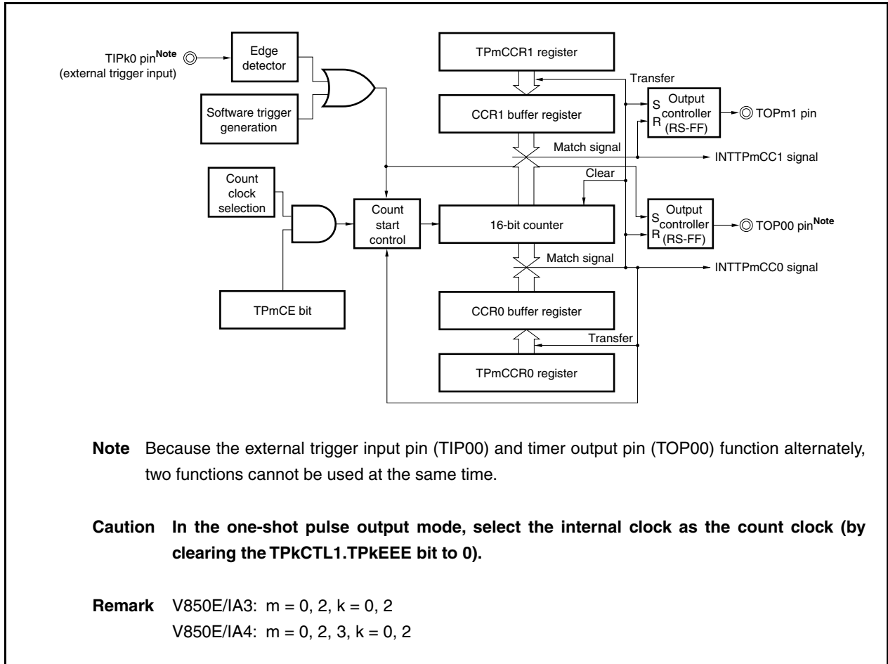
Figure 6-27. Configuration in One-Shot Pulse Output Mode
