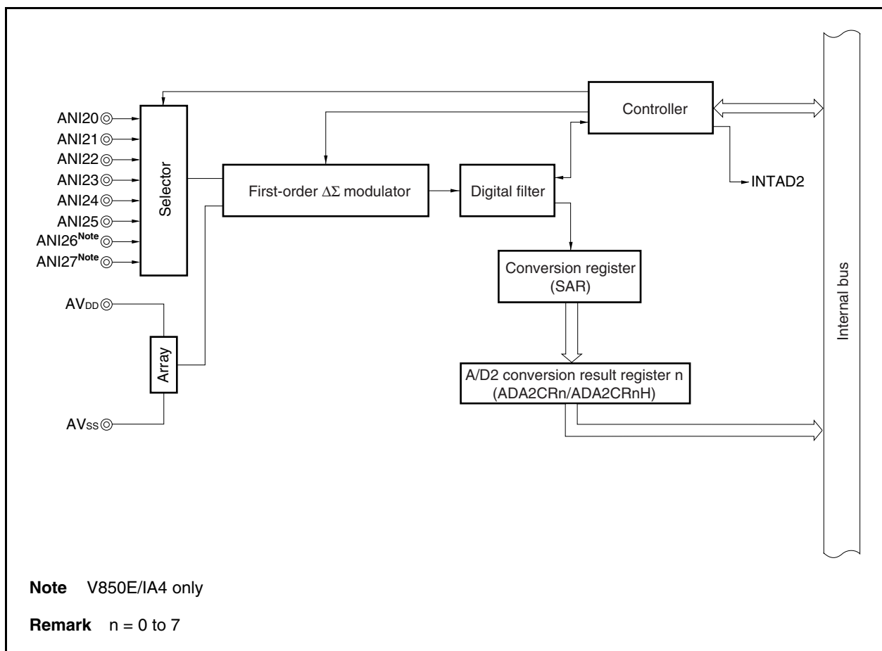
Figure 13-1. Block Diagram of A/D Converter 2
