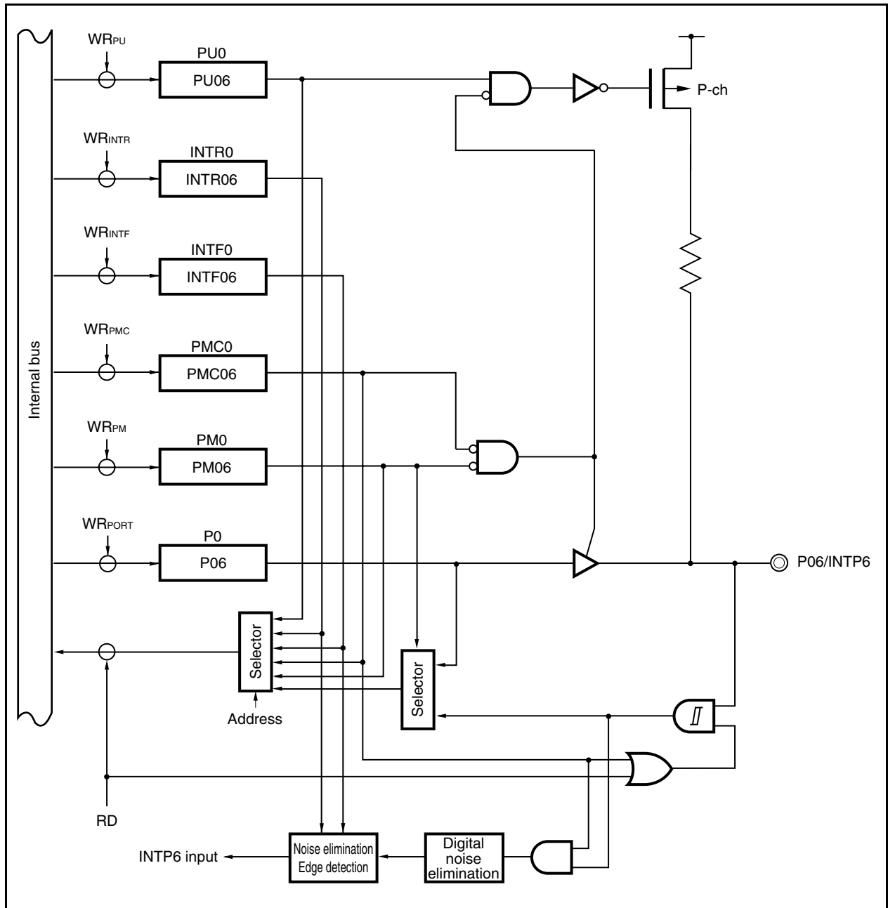
Figure 4-5. Block Diagram of P06 Pin
