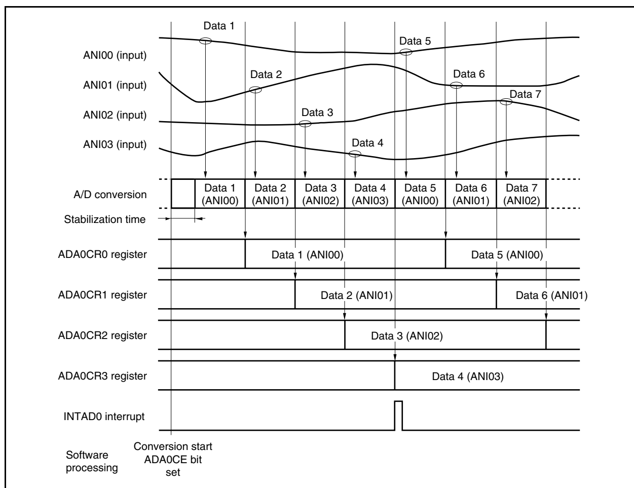
Figure 12-7. Continuous Scan Mode Operation Timing (When ADA0M0.ADA0MD1 and ADA0M0.ADA0MD0 Bits = 01, ADA0S.ADA0S2 to ADA0S.ADA0S0 Bits = 011): V850E/IA4
