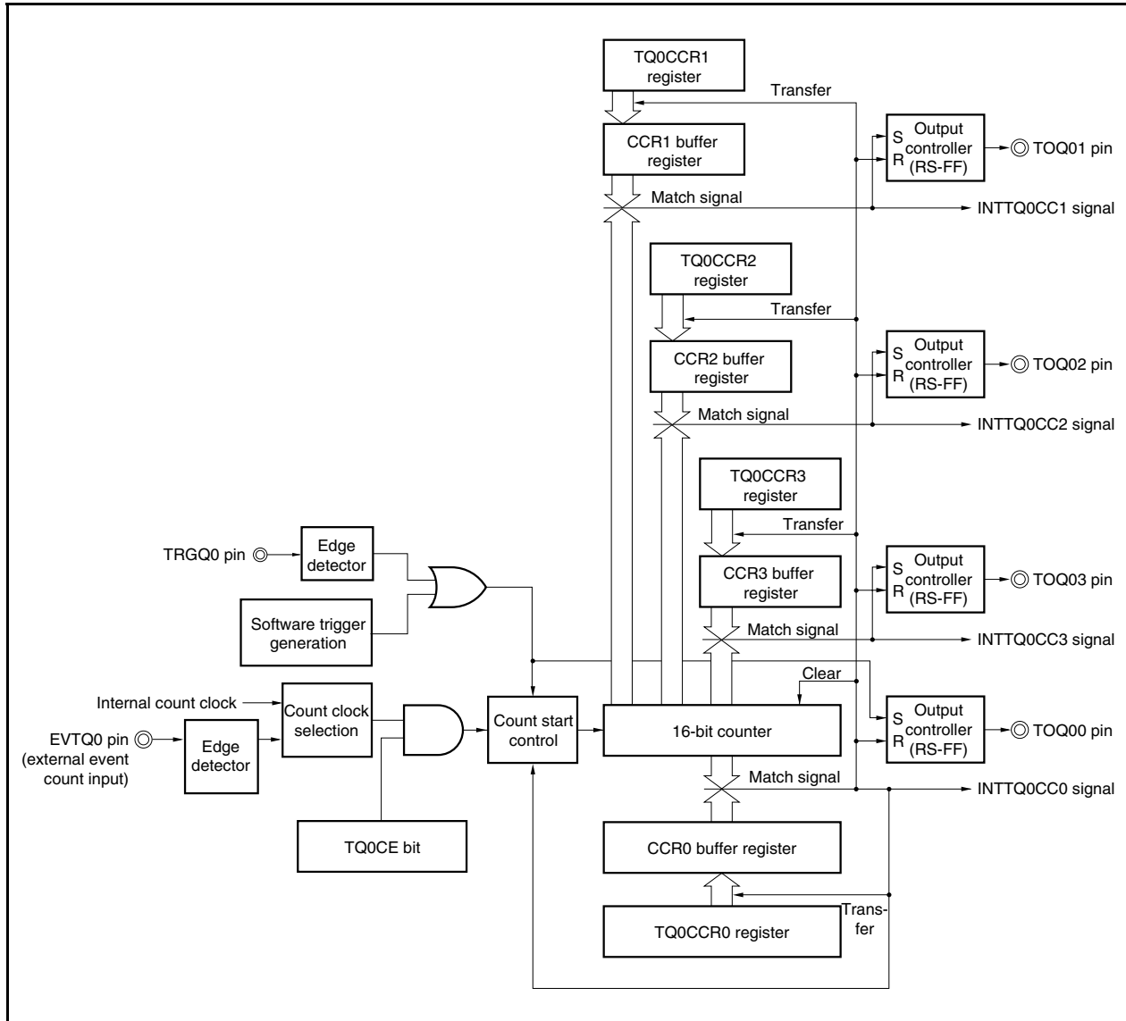
Figure 7-25. Configuration in One-Shot Pulse Output Mode
