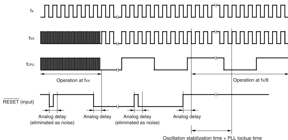
Figure 19-1. Reset Operation by \overline{\text{RESET}} Pin Input
