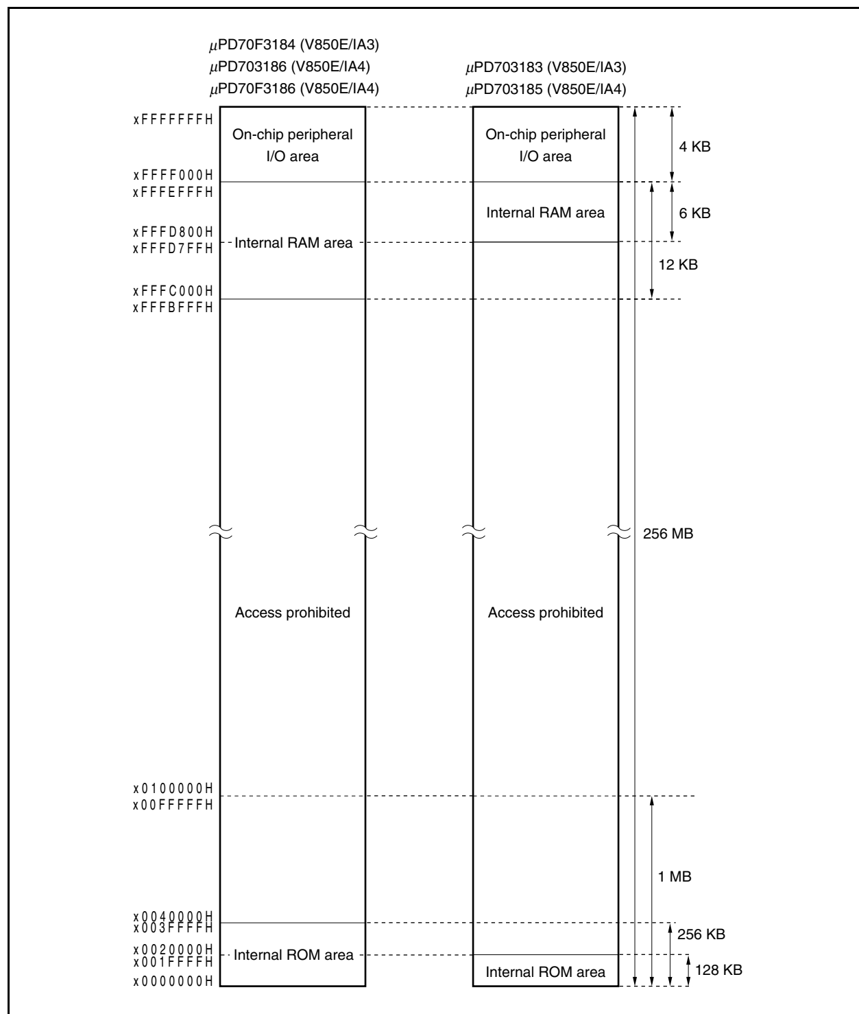
Figure 3-4. Memory Map
