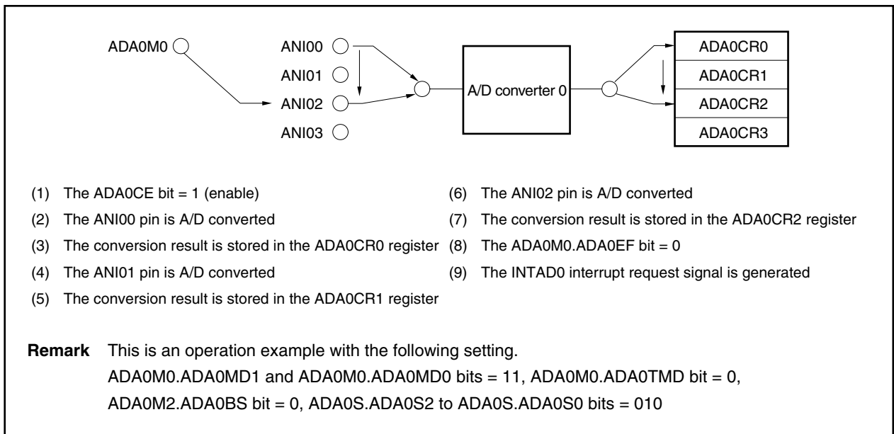
Figure 12-16. Example of One-Shot Scan Mode Operation (Software Trigger One-Shot Scan): V850E/IA4
