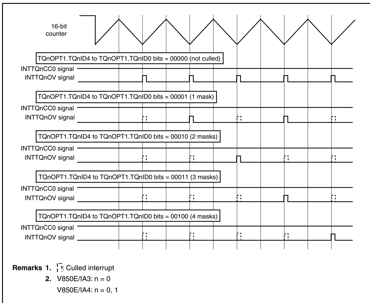
Figure 10-17. Interrupt Culling Operation When TQnOPT1.TQnICE Bit = 0, TQnOPT1.TQnIOE Bit = 1, TQnOPT2.TQnRDE Bit = 1 (Valley Interrupt Output)
