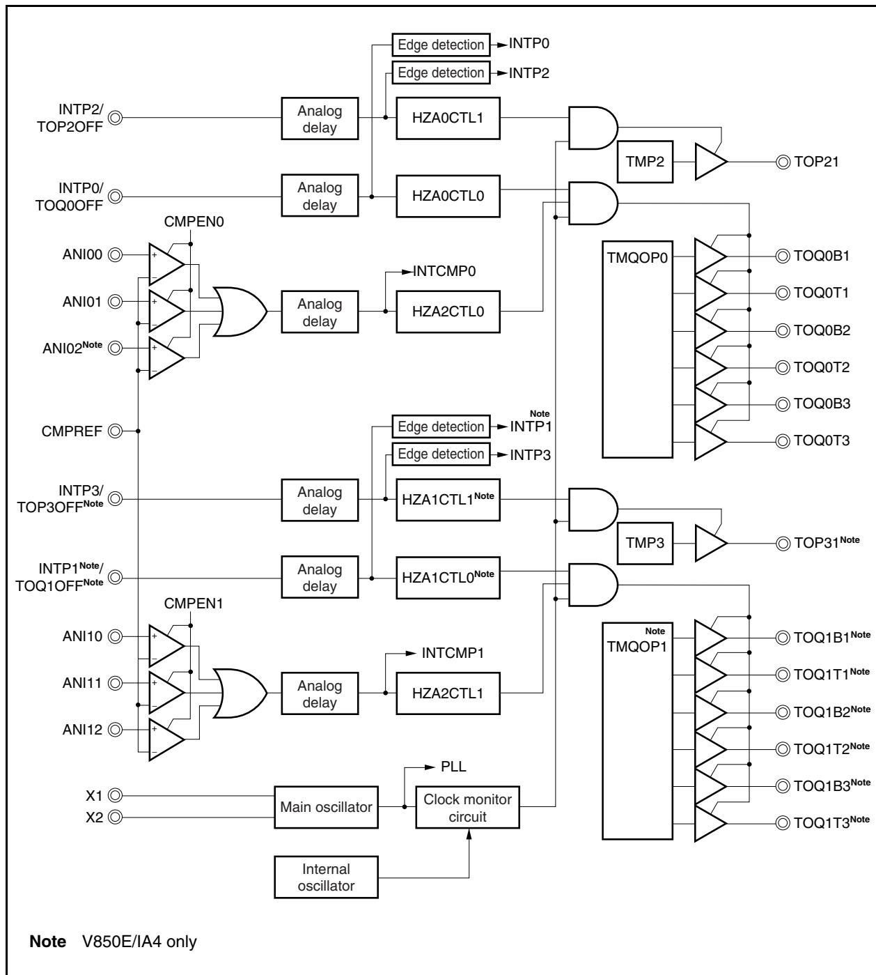
Figure 10-4. High-Impedance Output Controller Configuration
