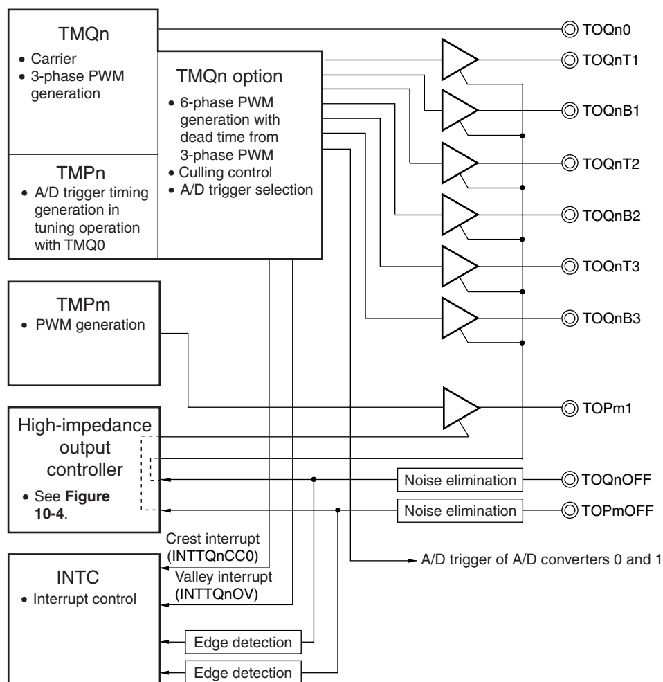
Figure 10-1. Block Diagram of Motor Control
