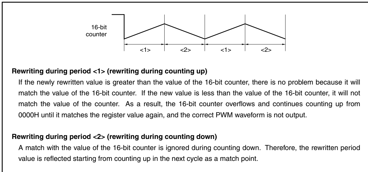
Figure 10-22. Example of Rewriting TQnCCR0 Register
