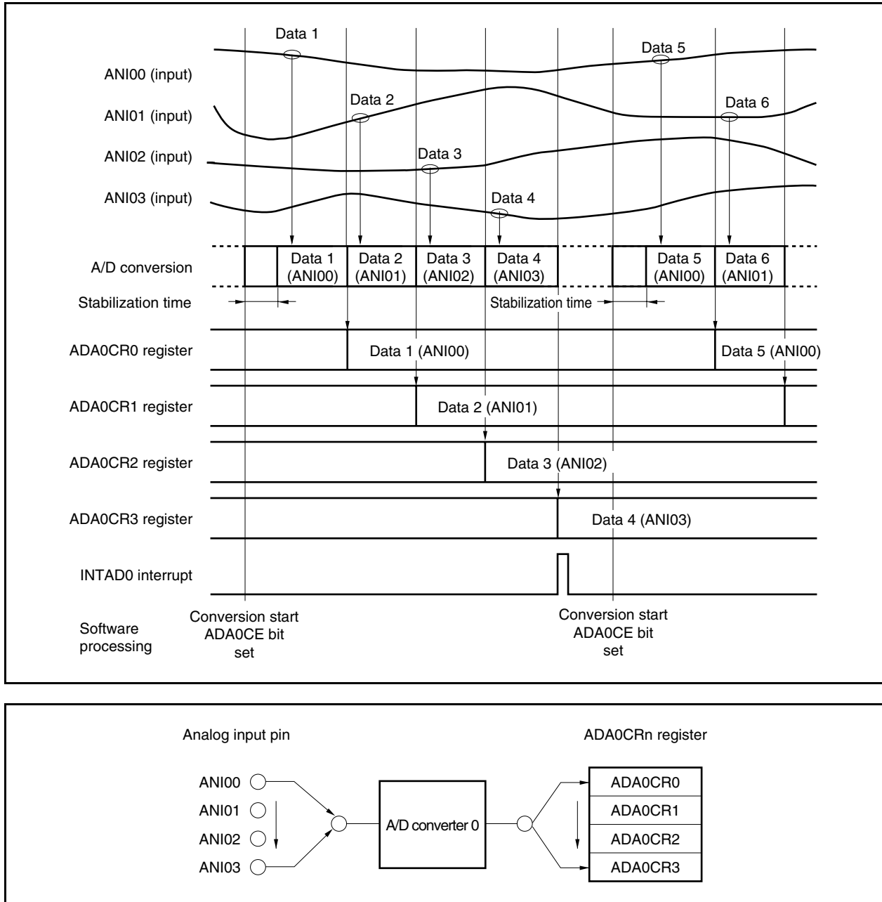
Figure 12-10. One-Shot Scan Mode Operation Timing (When ADA0M0.ADA0MD1 and ADA0M0.ADA0MD0 Bits = 11, ADA0S.ADA0S2 to ADA0S.ADA0S0 Bits = 011): V850E/IA4
