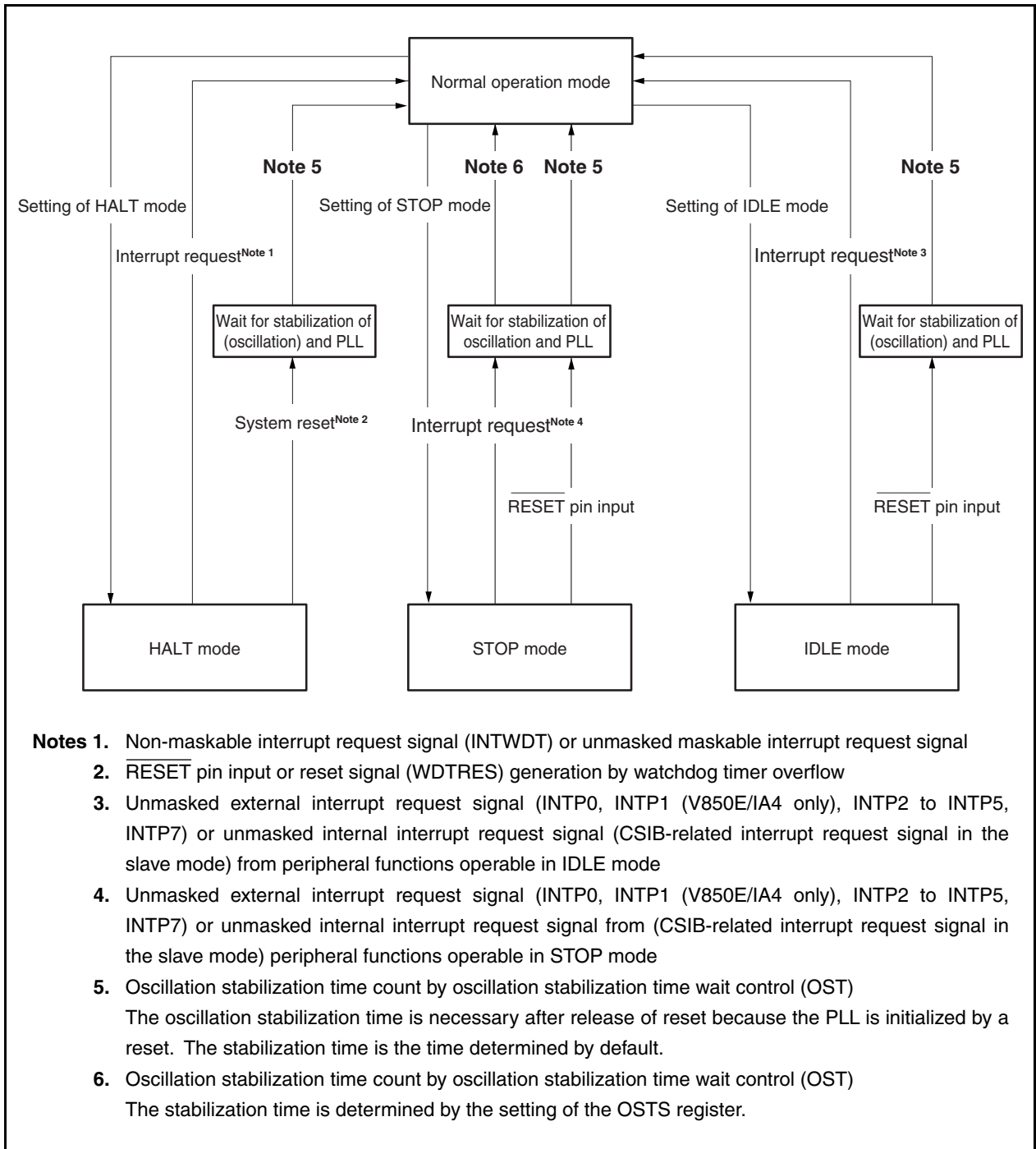
Figure 18-1. Status Transition
