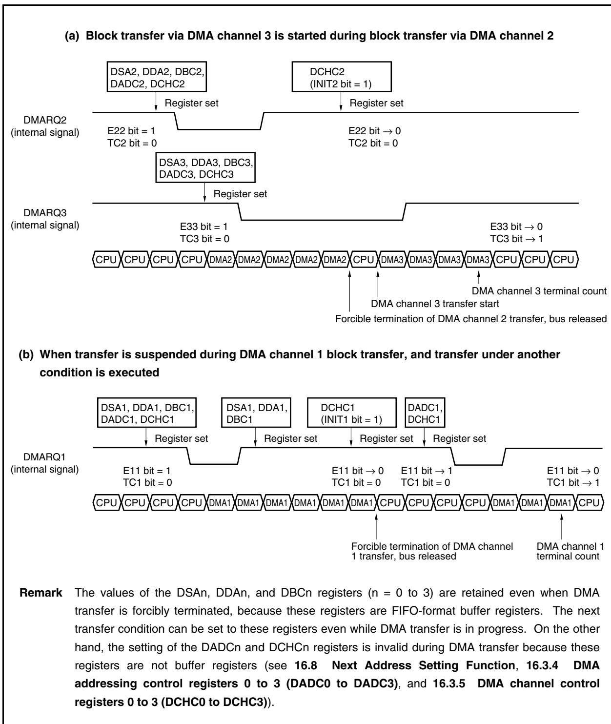
Figure 16-9. Example of Forcible Termination of DMA Transfer
