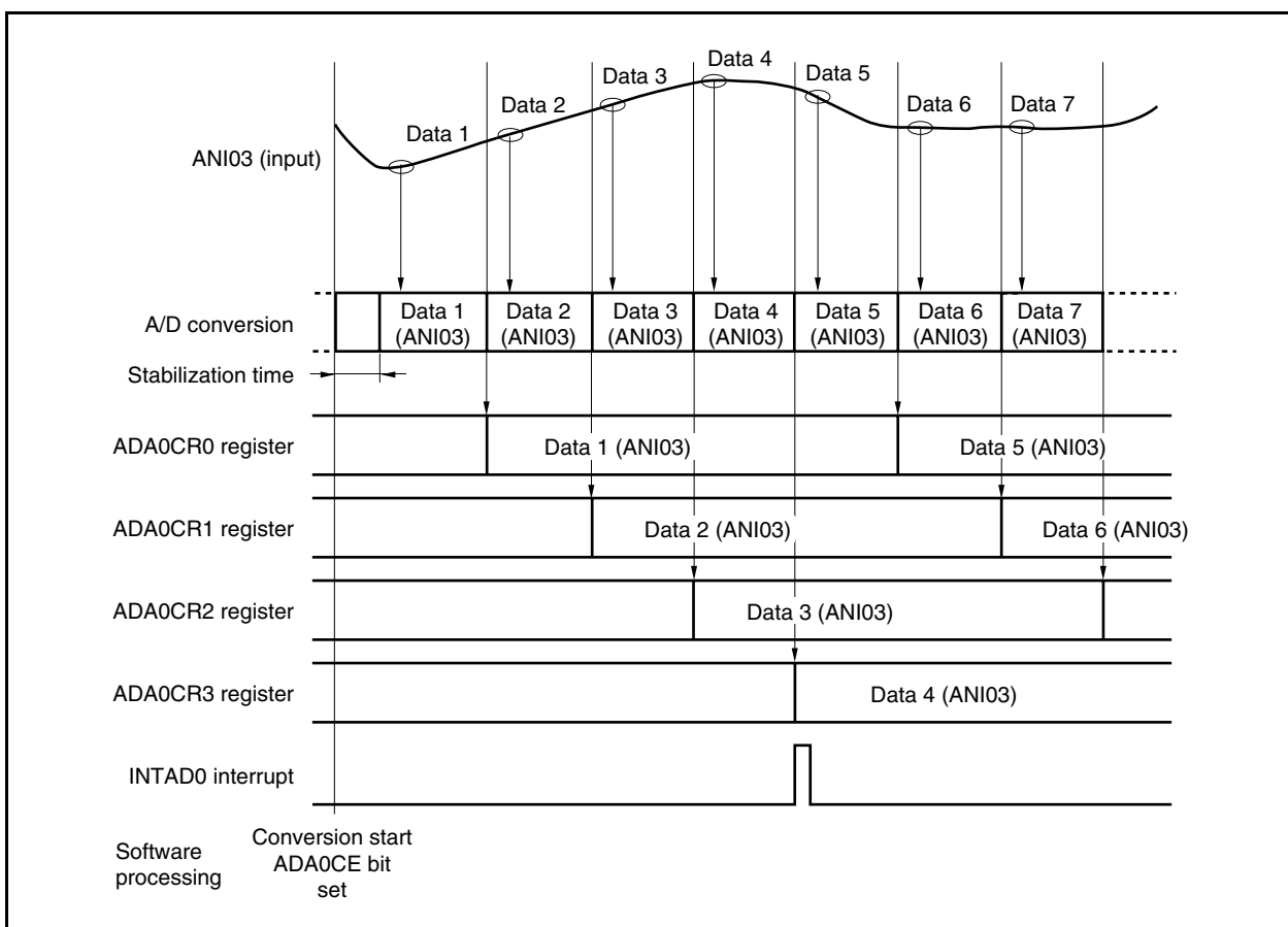
Figure 12-6. Continuous Select 4-Buffer Mode Operation Timing (When ADA0M0.ADA0MD1 and ADA0M0.ADA0MD0 Bits = 00, ADA0M2.ADA0BS Bit = 1, ADA0S.ADA0S2 to ADA0S.ADA0S0 Bits = 011): V850E/IA4
