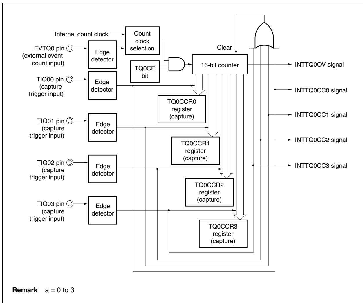
Figure 7-39. Configuration in Pulse Width Measurement Mode
