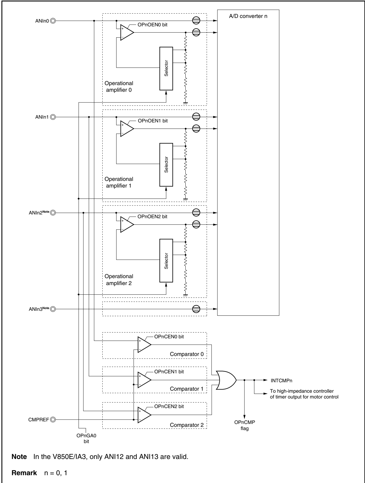
Figure 12-2. Block Diagram of Operational Amplifier for Input Level Amplification and Overvoltage Detection Comparator
