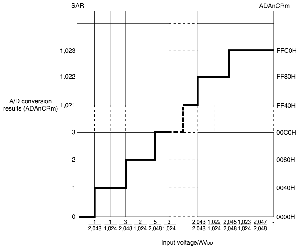
Figure 12-4. Relationship Between Analog Input Voltage and A/D Conversion Results
