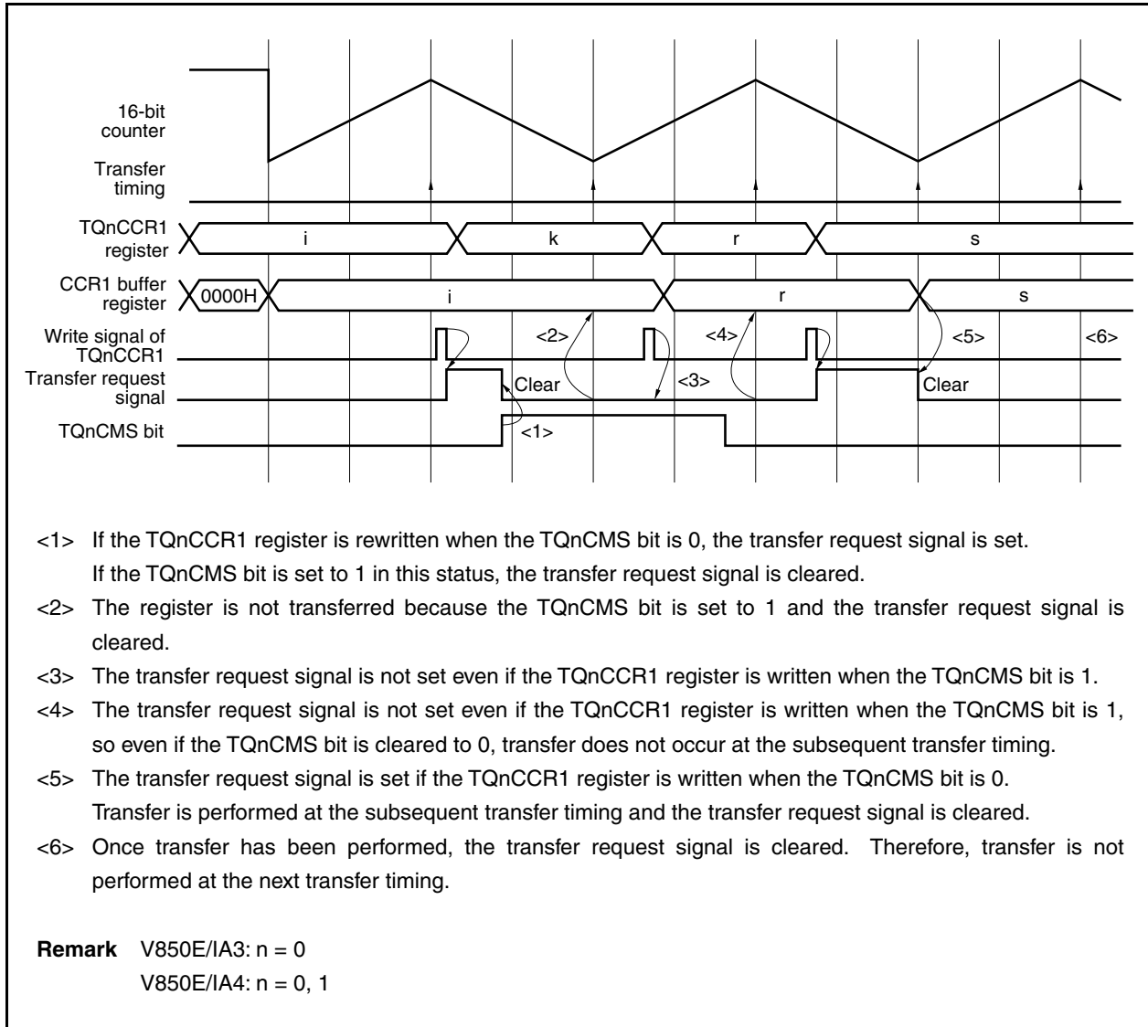
Figure 10-36. Rewriting TQnCMS Bit
