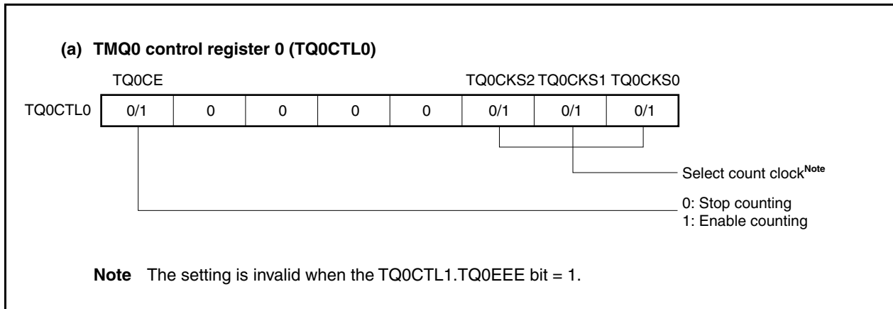
Figure 7-23. Setting of Registers in External Trigger Pulse Output Mode (1/3)
