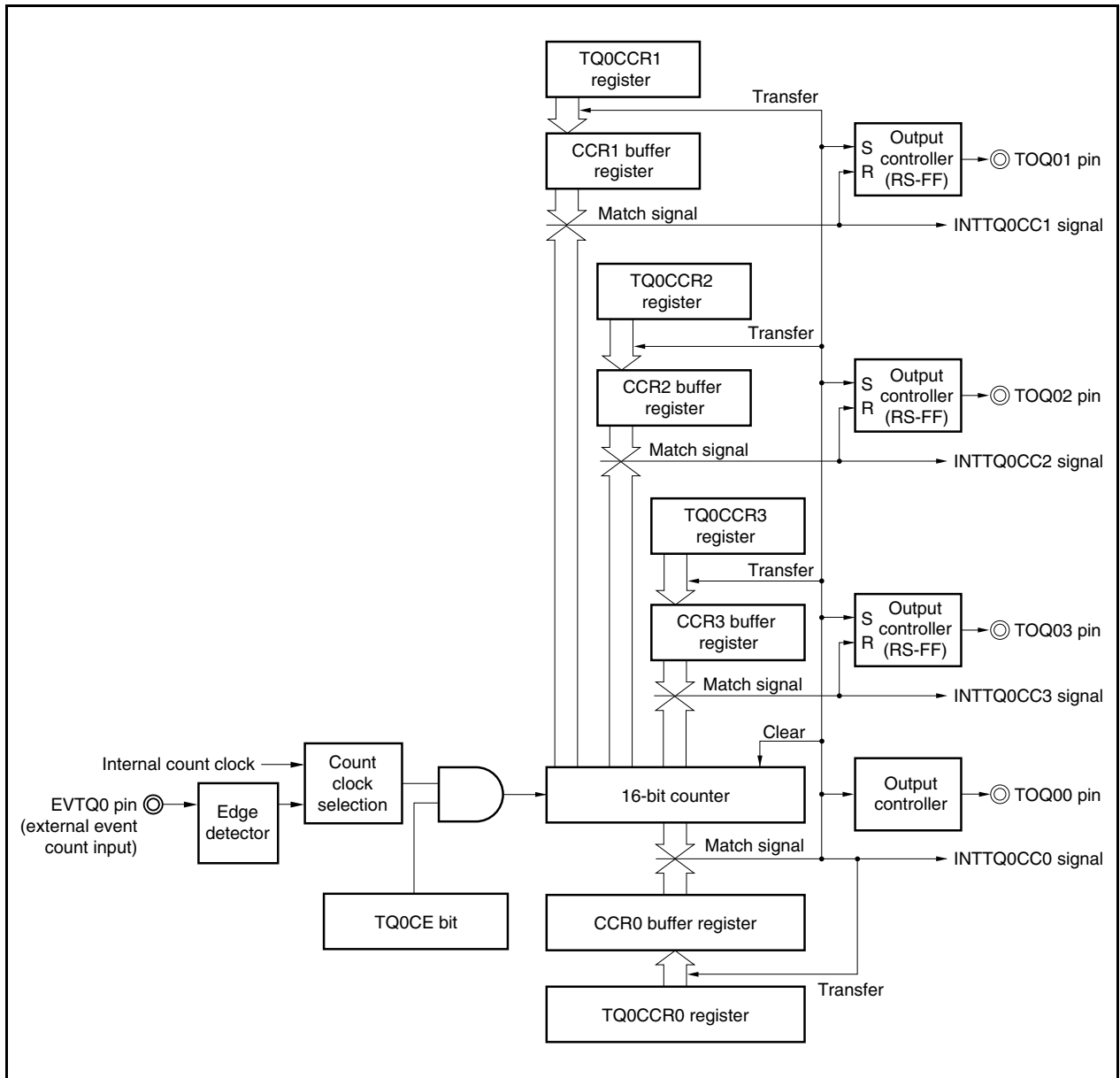
Figure 7-29. Configuration in PWM Output Mode
