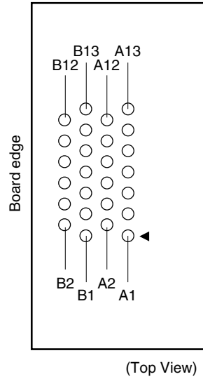
Figure 21-2. Pin Configuration of Emulator Connector (on Target System Side)
