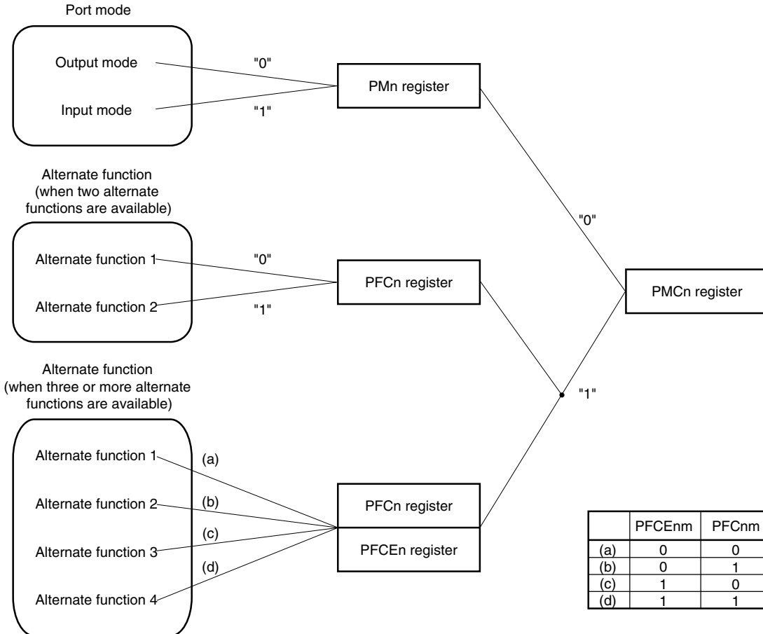
Figure 4-3. Register Settings and Pin Functions
