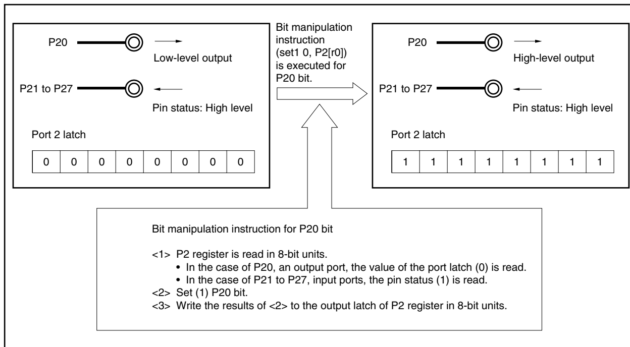
Figure 4-27. Bit Manipulation Instruction (P20 Pin)
