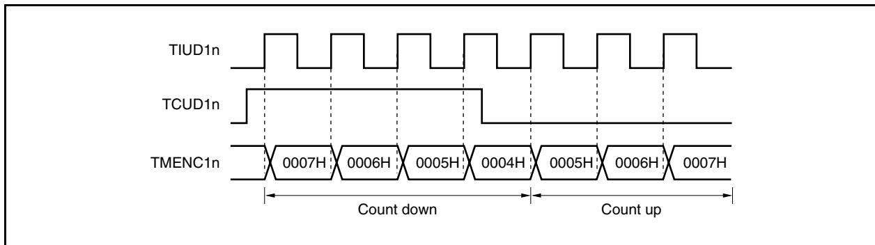
Figure 8-5. Mode 1 (When Rising Edge Is Specified as Valid Edge of TIUD1n Pin): In Case of Simultaneous TIUD1n, TCUD1n Pin Edge Timing
