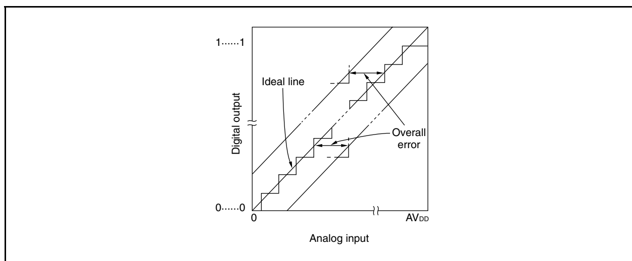
Figure 12-25. Overall Error
