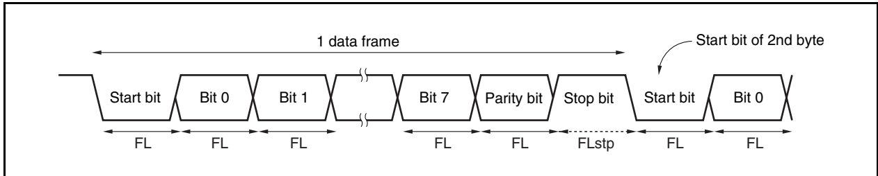
Figure 14-12. Transfer Rate During Continuous Transmission
