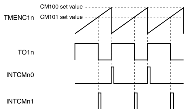
Figure 8-3. PWM Signal Output Example (When ALVT10n Bit = 0 Is Set)
