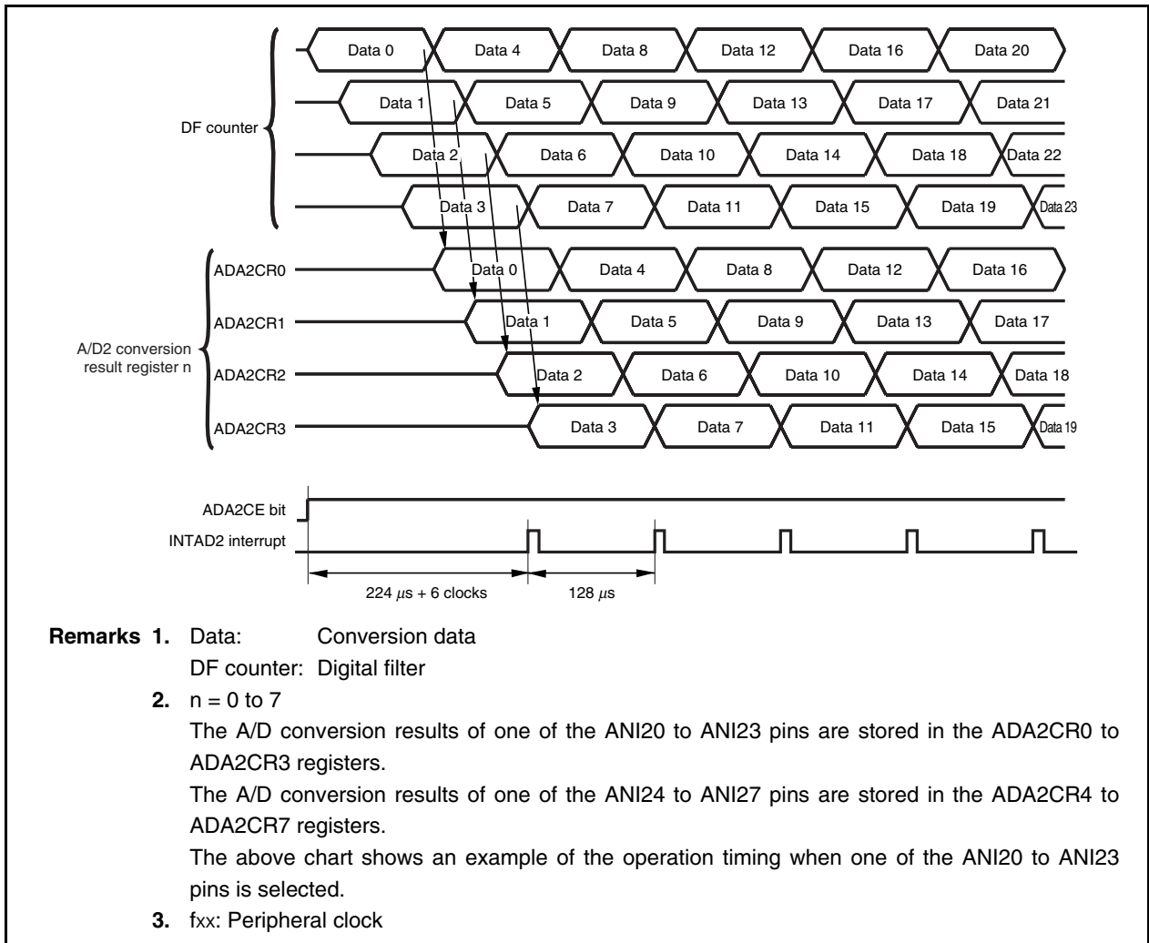
Figure 13-7. Example of Operation Timing in 4-Buffer Parallel Mode (with 8-Bit Resolution, fxx = 64 MHz)
