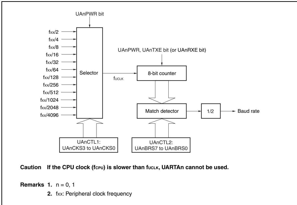
Figure 14-10. Configuration of Baud Rate Generator
