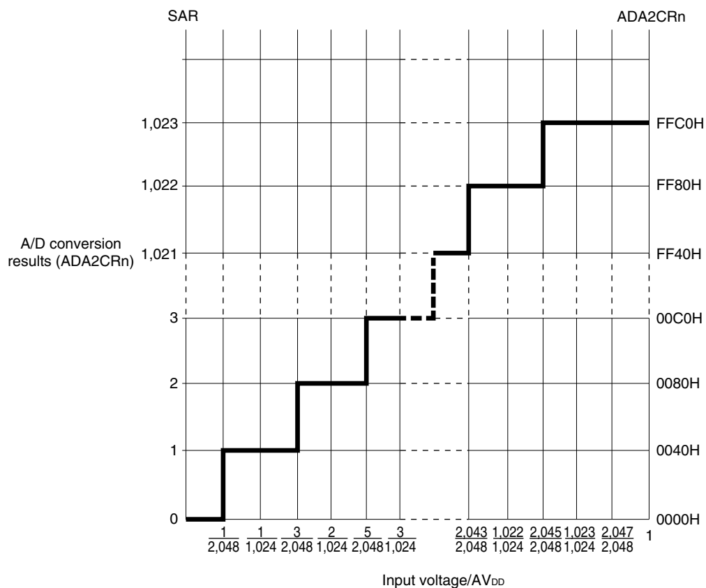
Figure 13-3. Relationship Between Analog Input Voltage and A/D Conversion Results (When 10-Bit Resolution Setting)
