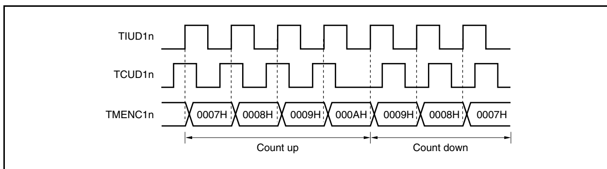
Figure 8-7. Mode 3 (When Rising Edge Is Specified as Valid Edge of TIUD1n Pin)
