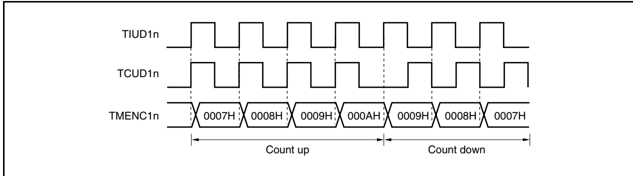
Figure 8-8. Mode 3 (When Rising Edge Is Specified as Valid Edge of TIUD1n Pin): In Case of Simultaneous TIUD1n, TCUD1n Pin Edge Timing
