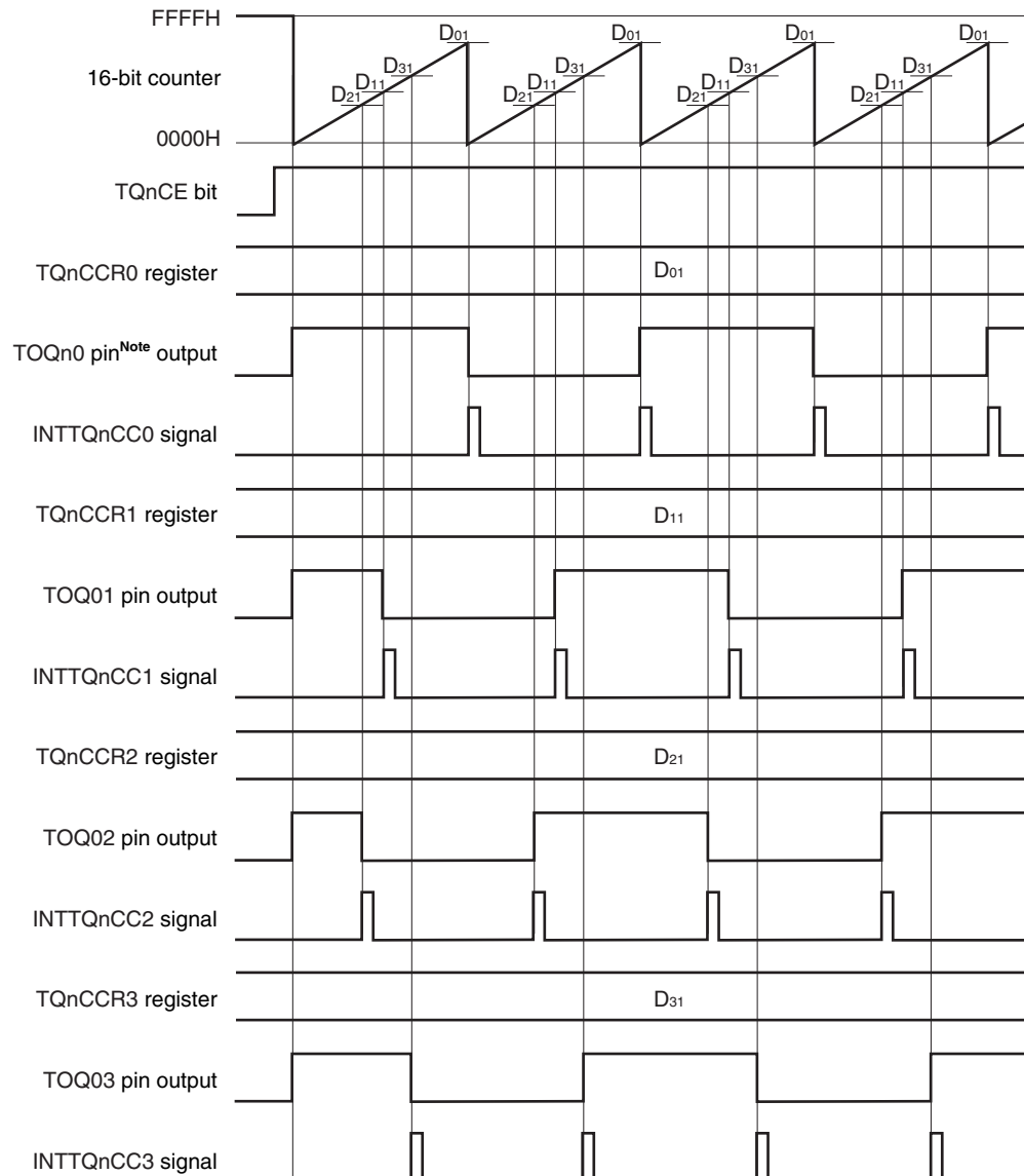
Figure 7-12. Timing Chart When D_{01} \geq D_{b1}
