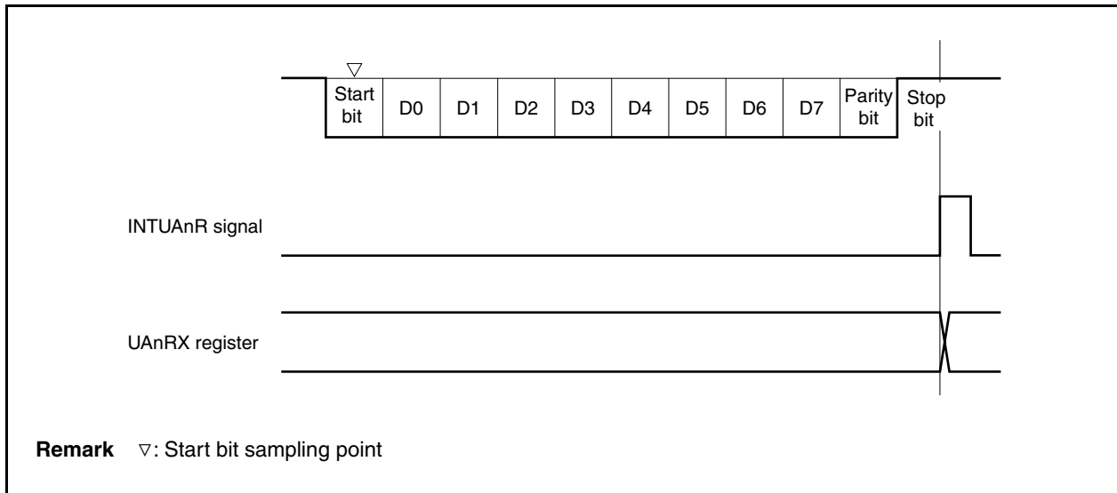
Figure 14-7. UART Reception
