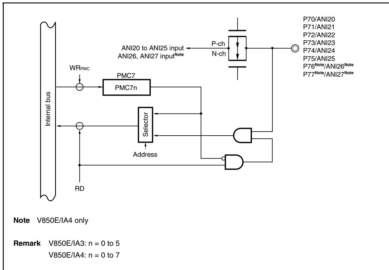
Figure 4-24. Block Diagram of P70 to P77 Pins
