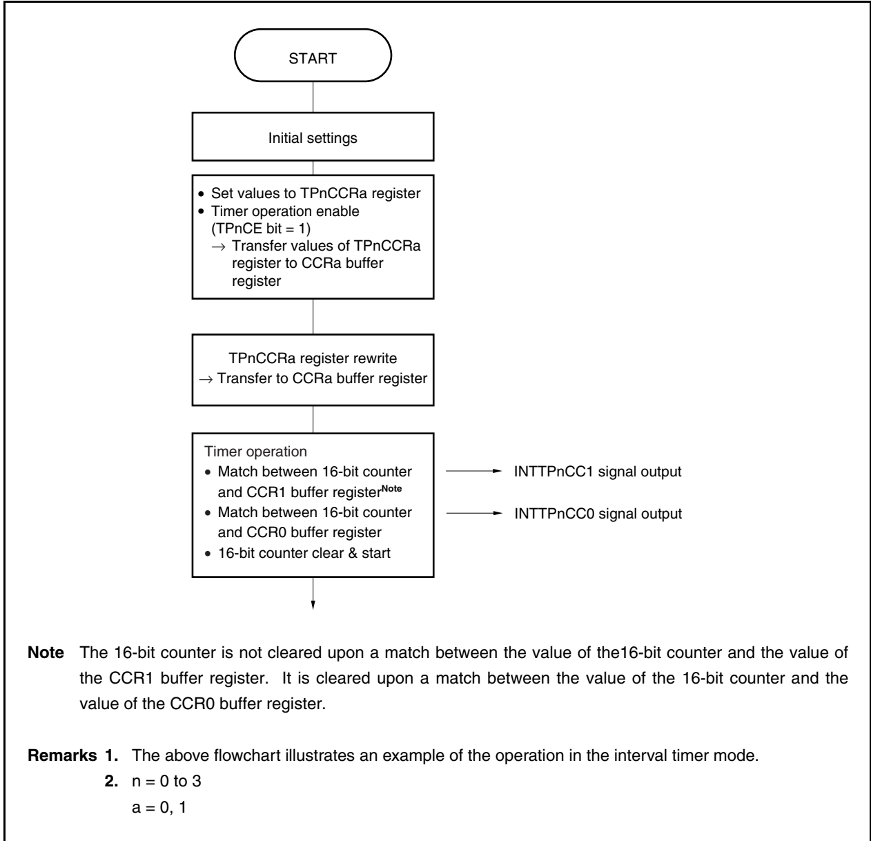
Figure 6-5. Flowchart of Basic Operation for Anytime Write
