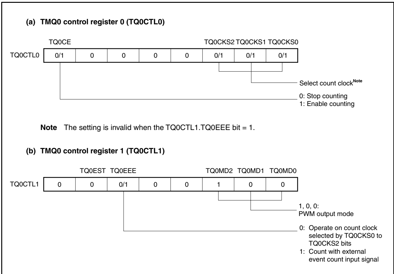
Figure 7-31. Register Setting in PWM Output Mode (1/3)
