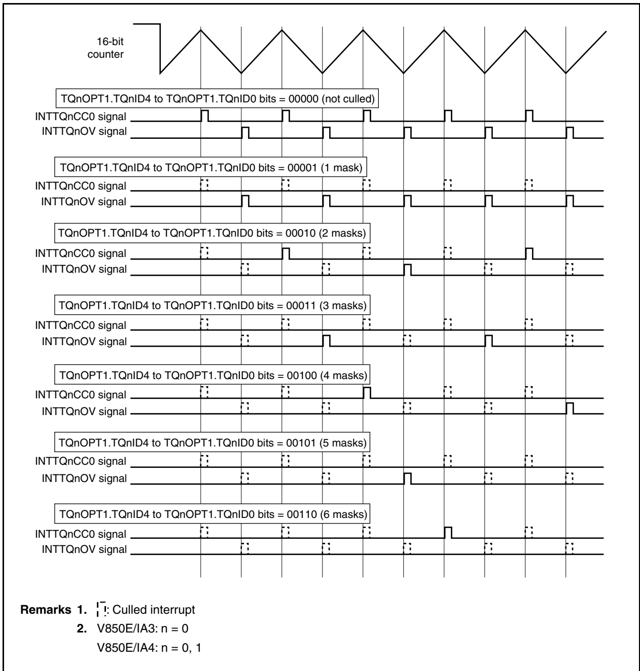
Figure 10-15. Interrupt Culling Operation When TQnOPT1.TQnICE Bit = 1, TQnOPT1.TQnIOE Bit = 1, TQnOPT2.TQnRDE Bit = 1 (Crest/Valley Interrupt Output)
