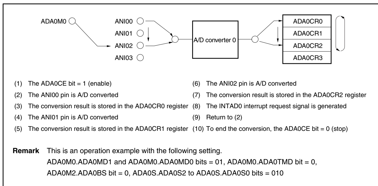
Figure 12-13. Example of Continuous Scan Mode Operation (Software Trigger Continuous Scan): V850E/IA4
