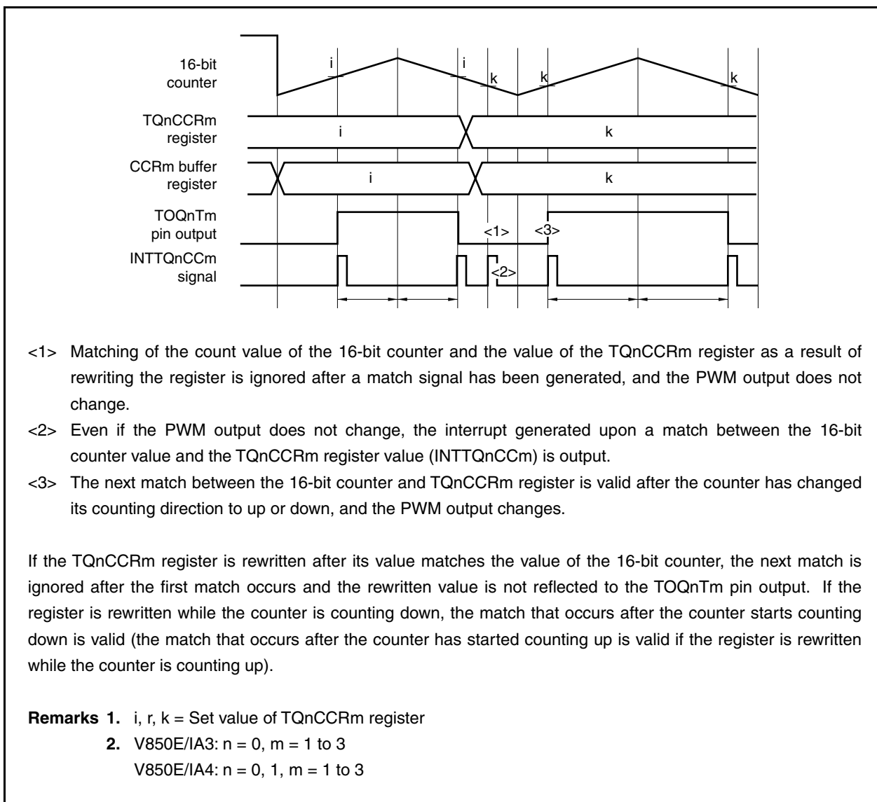
Figure 10-25. Example of Rewriting TQnCCR1 to TQnCCR3 Registers (Rewriting After Match Occurs)
