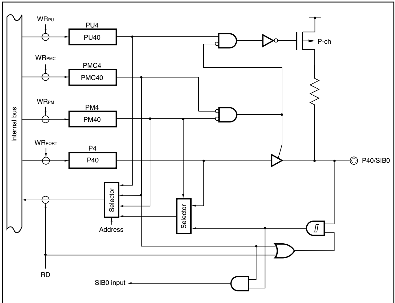
Figure 4-18. Block Diagram of P40 Pin
