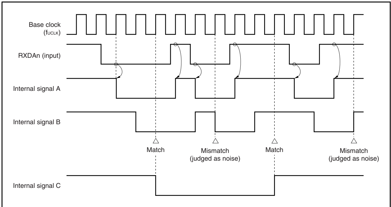
Figure 14-9. Timing of RXDAn Signal Judged as Noise
