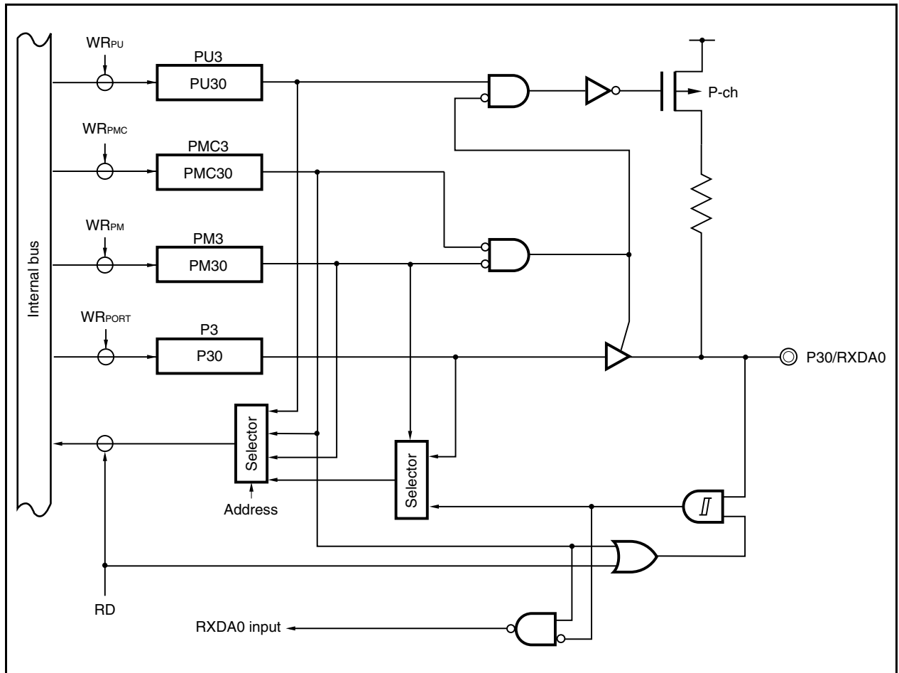
Figure 4-11. Block Diagram of P30 Pin
