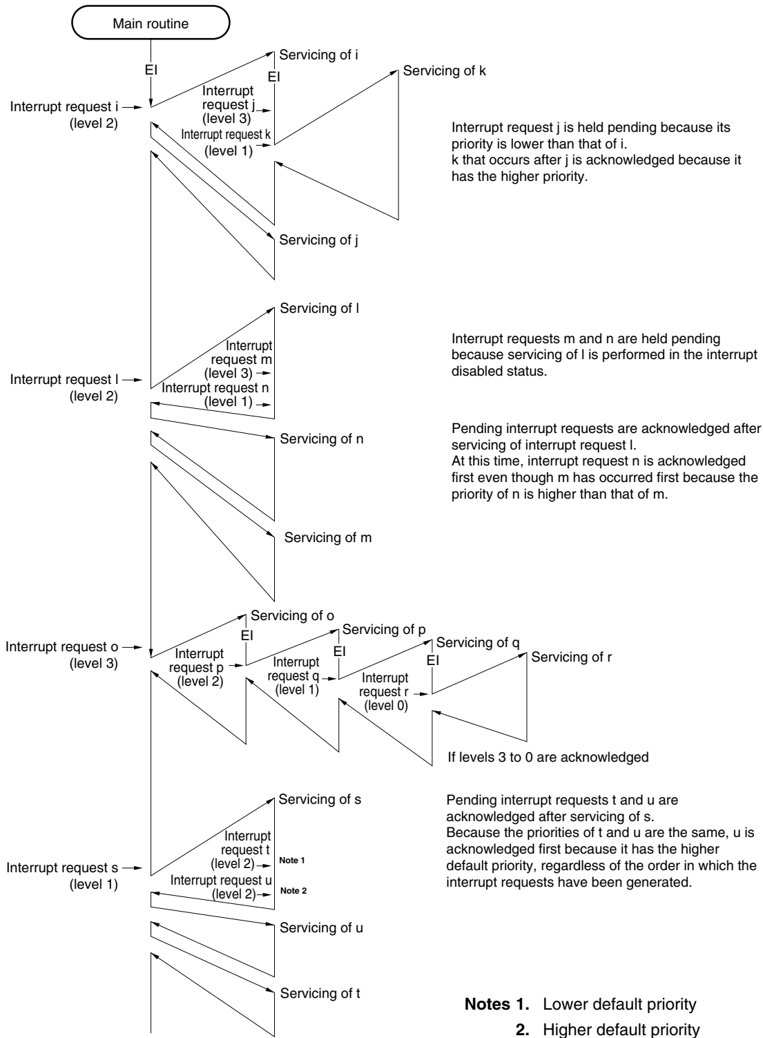
Figure 17-6. Example of Processing in Which Another Interrupt Request Signal Is Issued While an Interrupt Is Being Serviced (2/2)
