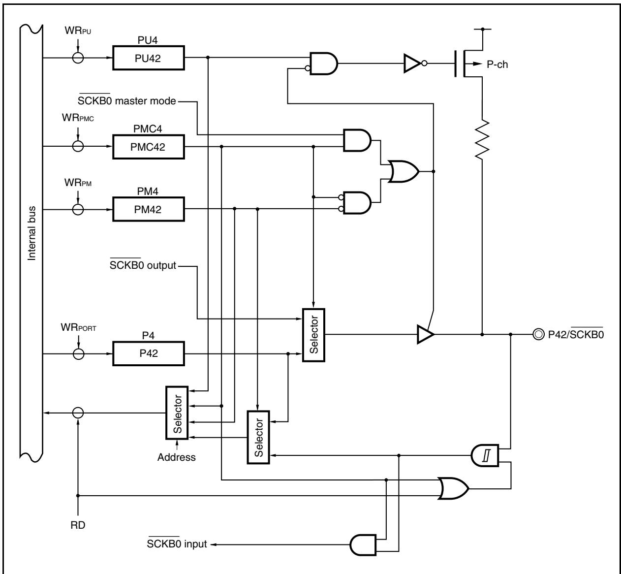
Figure 4-20. Block Diagram of P42 Pin
