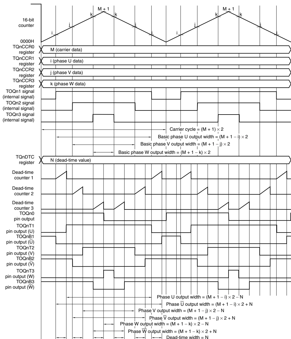
Figure 10-6. Timing Chart of 6-Phase PWM Output Mode
