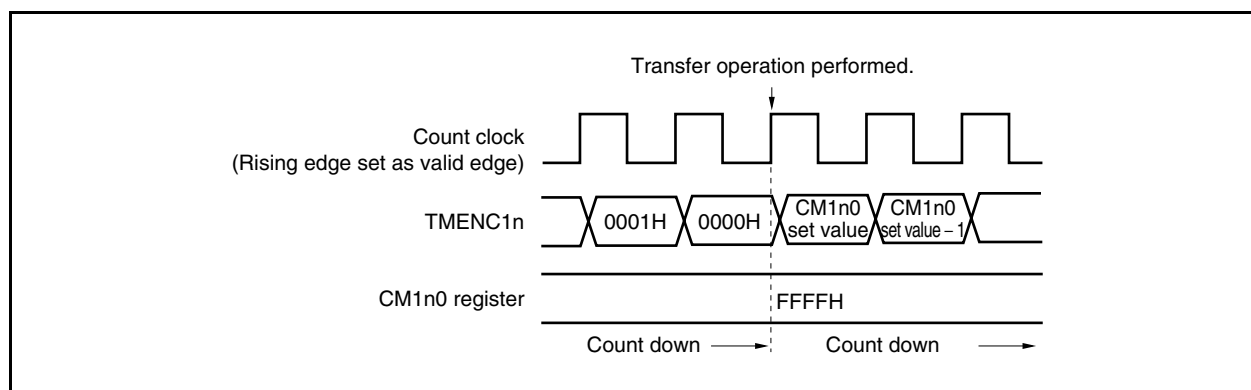
Figure 8-14. Internal Operation During Transfer Operation
