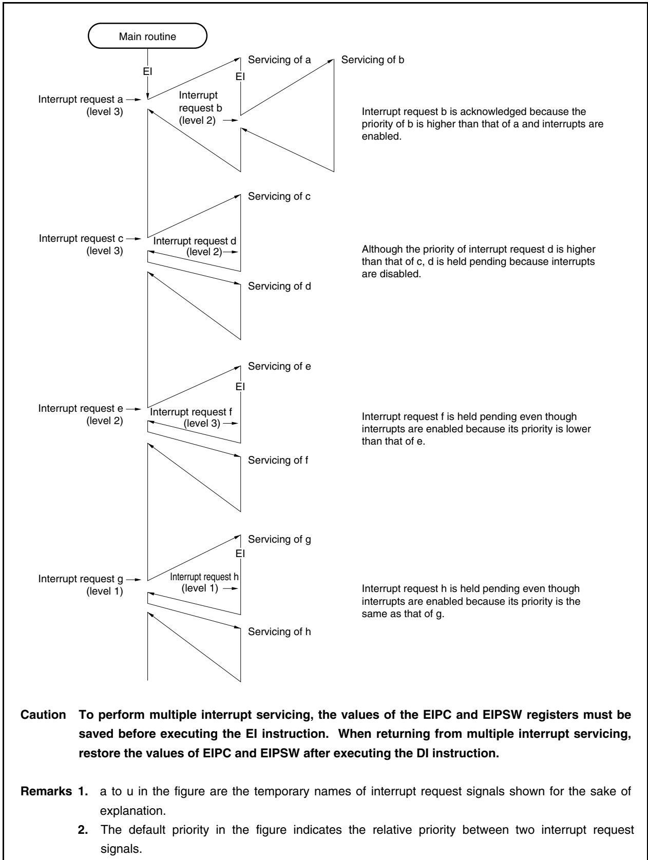
Figure 17-6. Example of Processing in Which Another Interrupt Request Signal Is Issued While an Interrupt Is Being Serviced (1/2)
