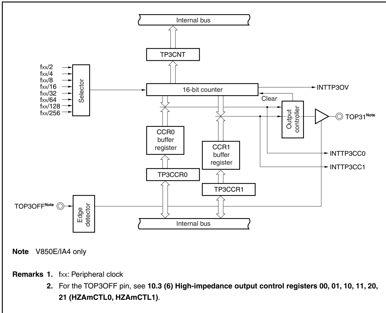
Figure 6-4. TMP3 Block Diagram
