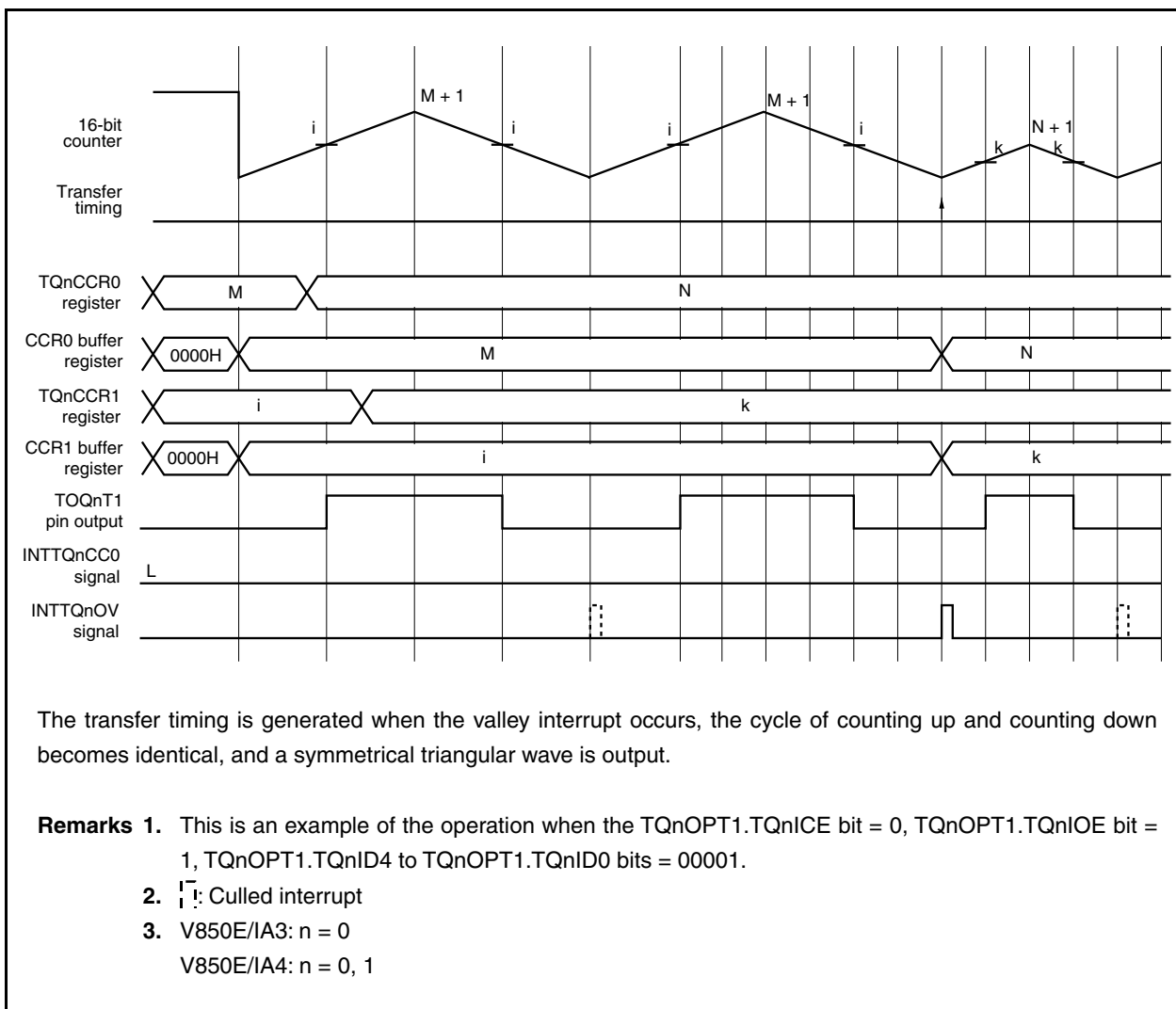
Figure 10-33. Rewriting TQnCCR0 Register (When Valley Interrupt Is Set)
