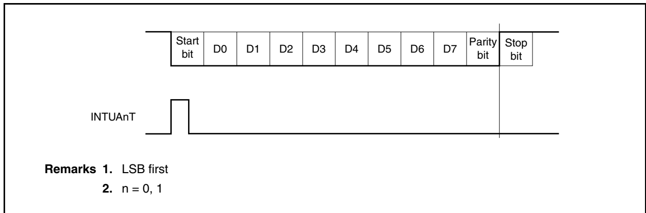
Figure 14-4. UART Transmission
