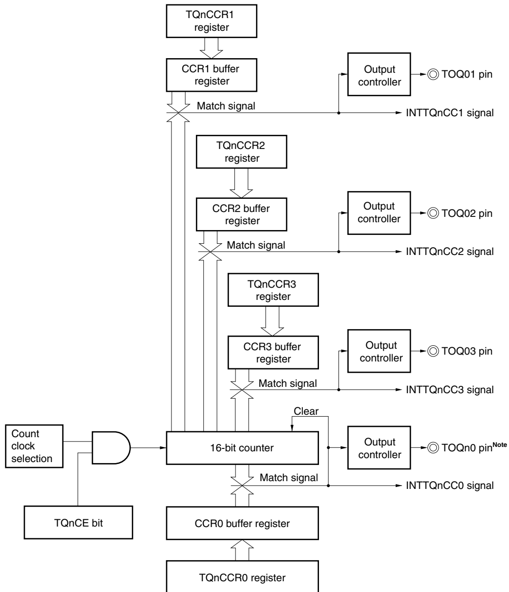
Figure 7-11. Configuration of TQnCCR1 to TQnCCR3 Registers
