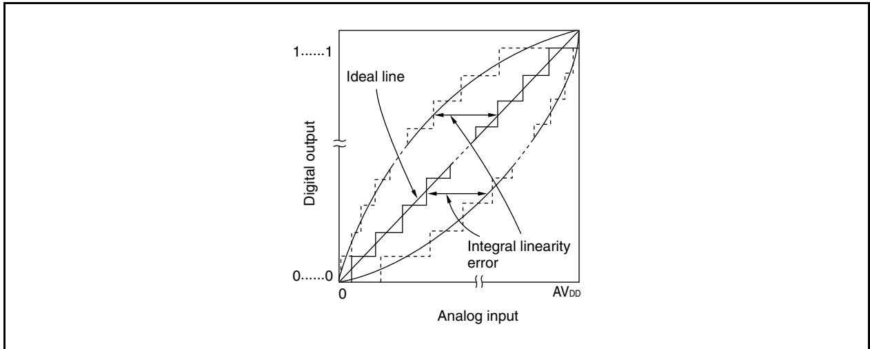
Figure 12-30. Integral Linearity Error
