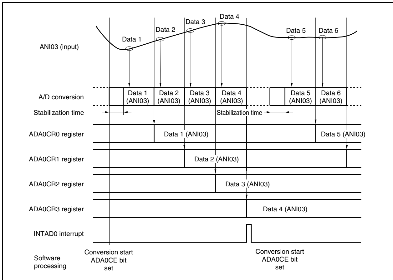
Figure 12-9. One-Shot Select 4-Buffer Mode Operation Timing (When ADA0M0.ADA0MD1 and ADA0M0.ADA0MD0 Bit = 10, A0M2.ADA0BS Bit = 1, ADA0S.ADA0S2 to ADA0S.ADA0S0 Bits = 011): V850E/IA4
