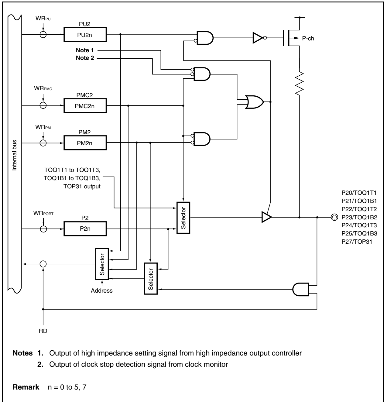
Figure 4-9. Block Diagram of P20 to P25, and P27 Pins
