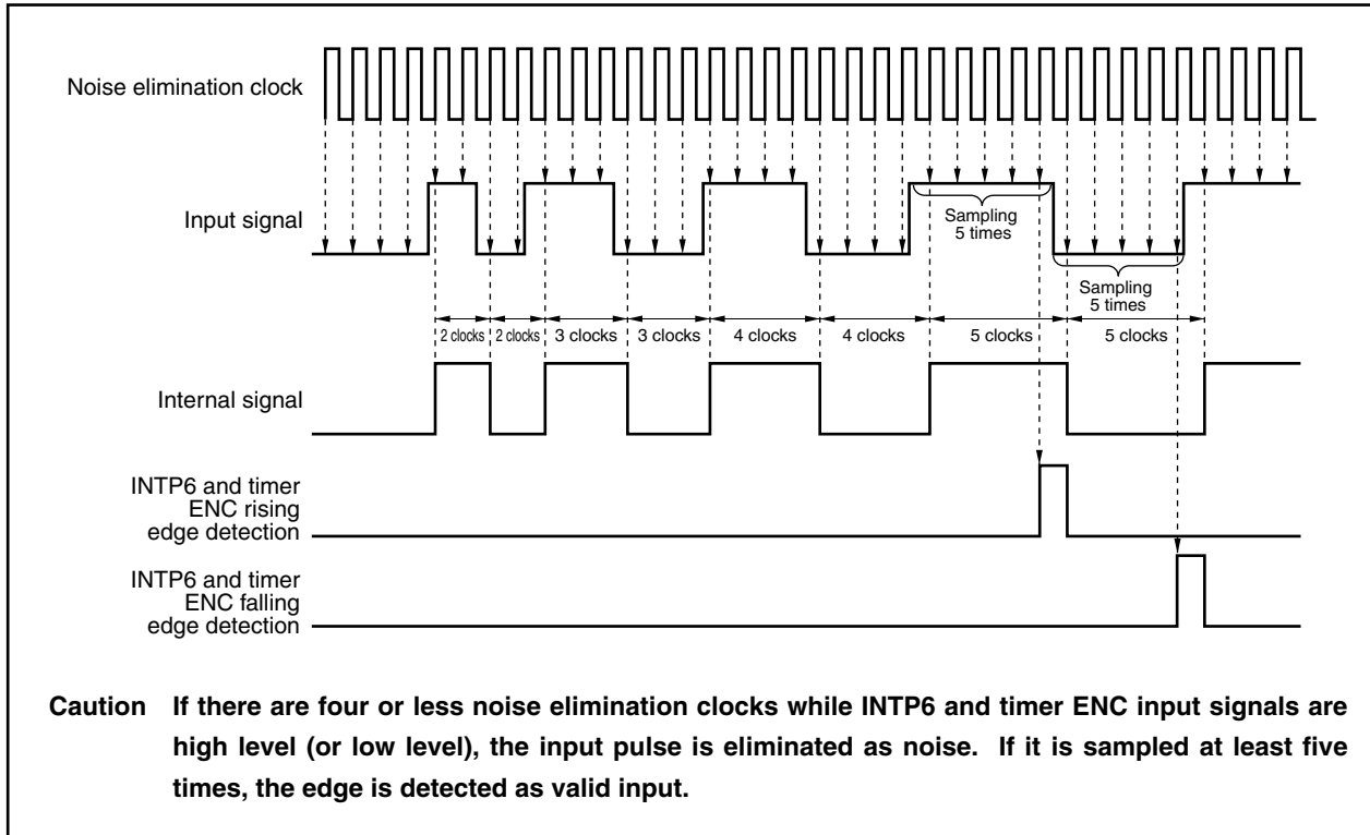
Figure 4-26. Example of Noise Elimination Timing
