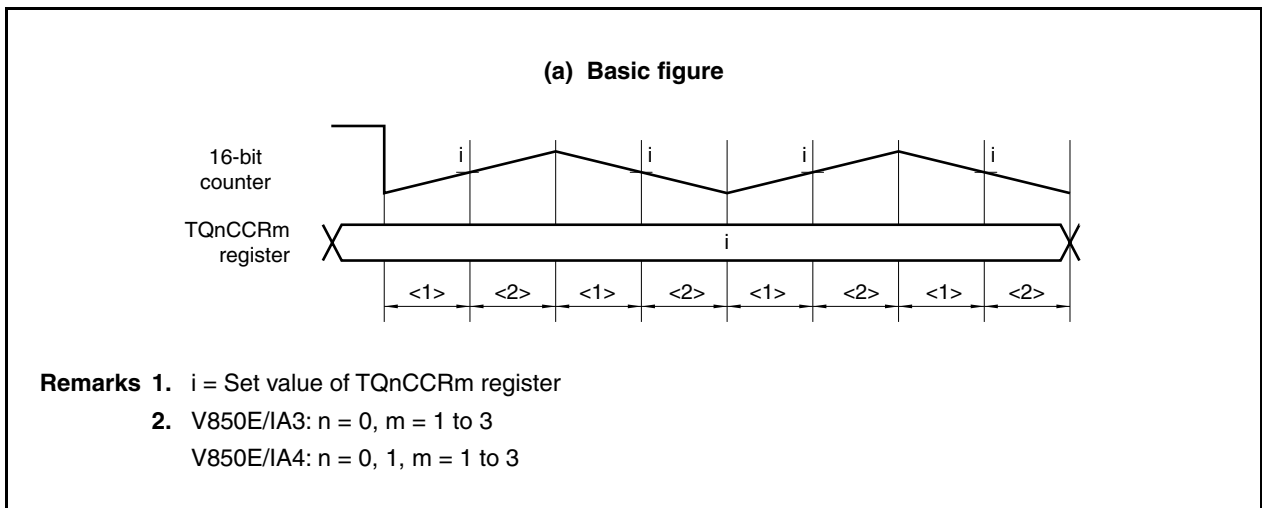
Figure 10-23. Basic Operation of 16-Bit Counter and TQnCCRm Register
