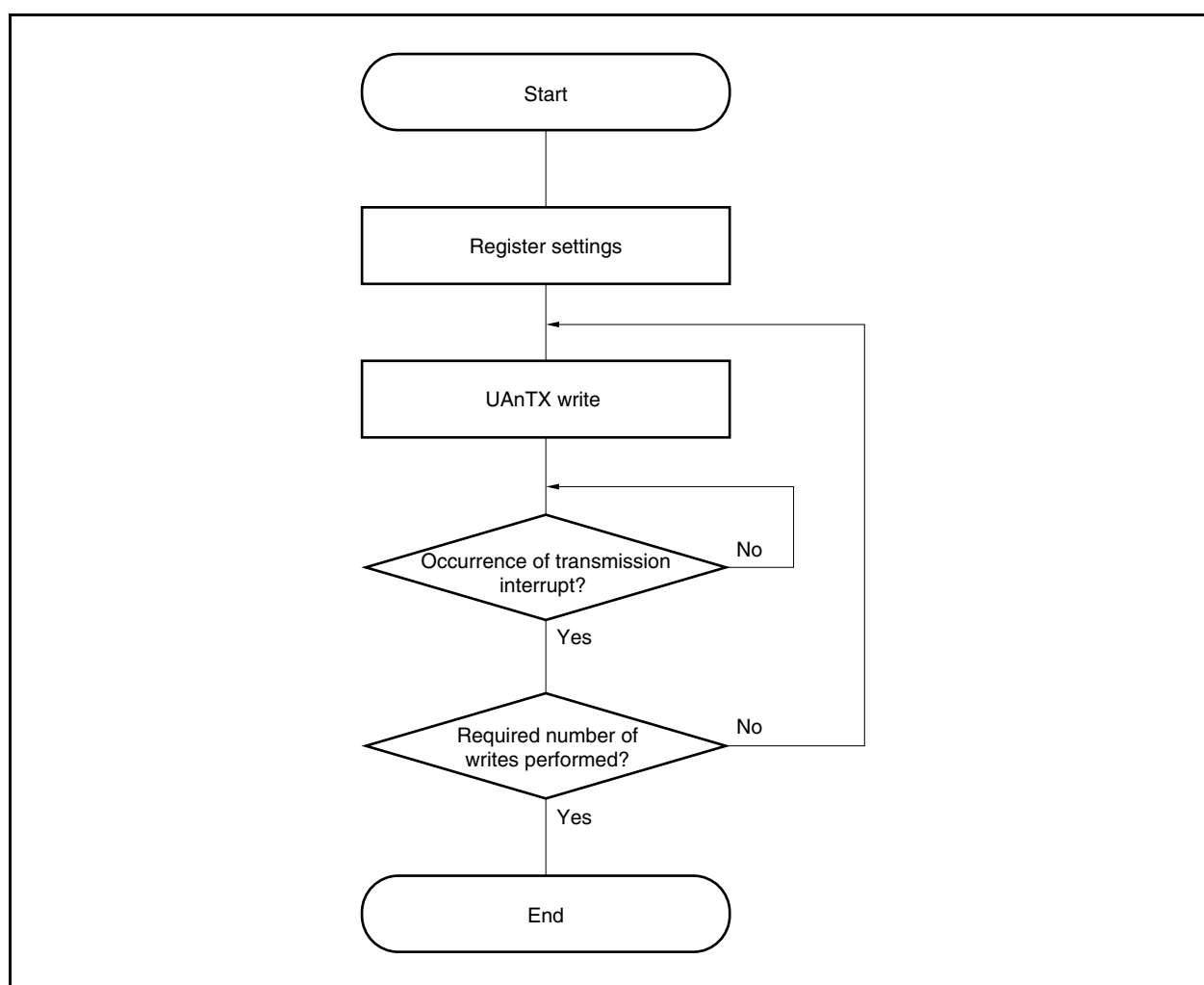
Figure 14-5. Continuous Transmission Processing Flow
