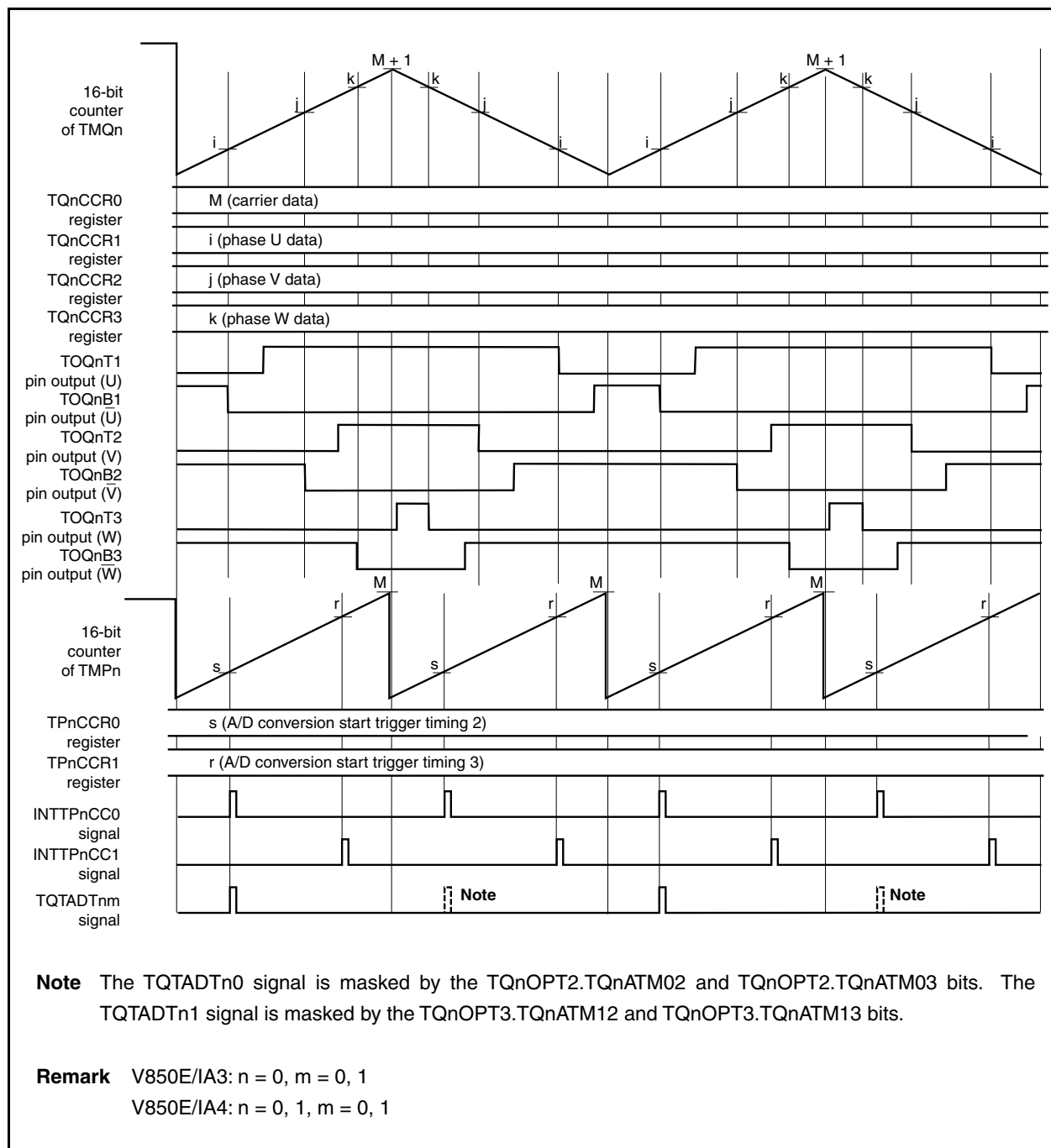
Figure 10-37. TMPn During Tuning Operation
