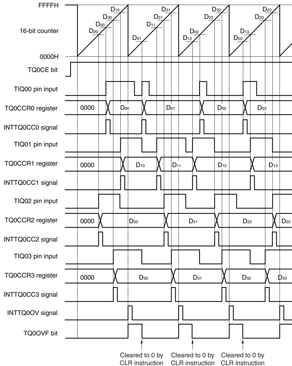
Figure 7-35. Basic Timing in Free-Running Timer Mode (Capture Function)
