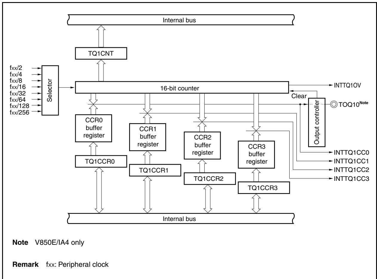
Figure 7-2. TMQ1 Block Diagram
