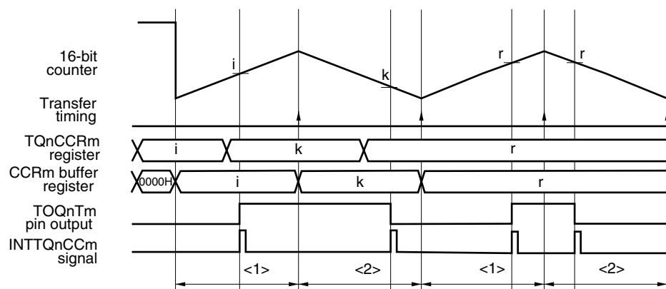
Figure 10-30. Example of Rewriting TQnCCRm Register
