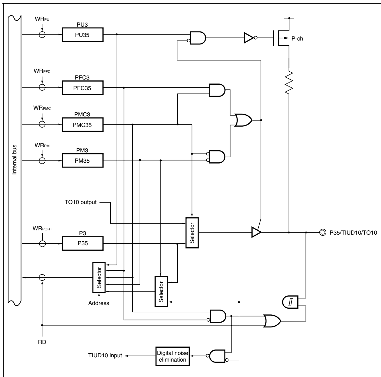
Figure 4-16. Block Diagram of P35 Pin
