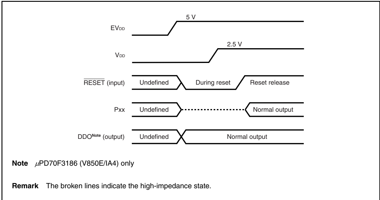
Figure 19-2. Timing and Pin Status at Power-On
