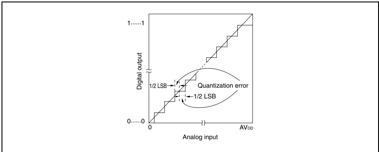
Figure 12-26. Quantization Error
