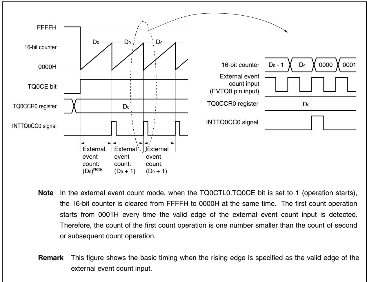
Figure 7-15. Basic Timing in External Event Count Mode
