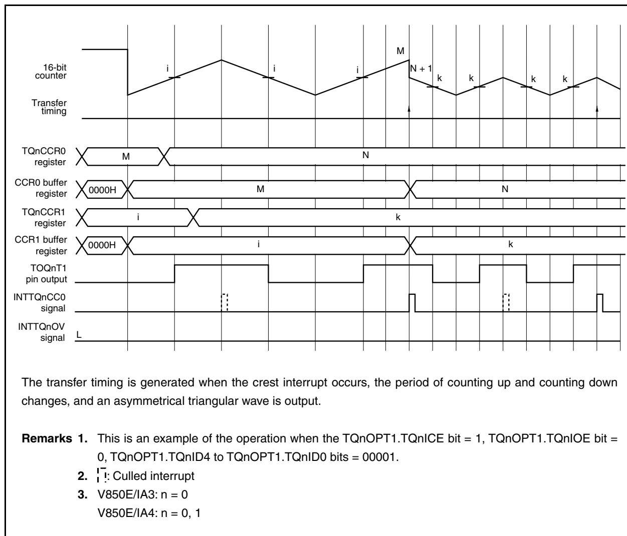
Figure 10-32. Rewriting TQnCCR0 Register (When Crest Interrupt Is Set)
