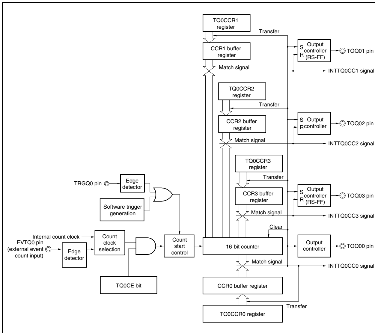
Figure 7-21. Configuration in External Trigger Pulse Output Mode
