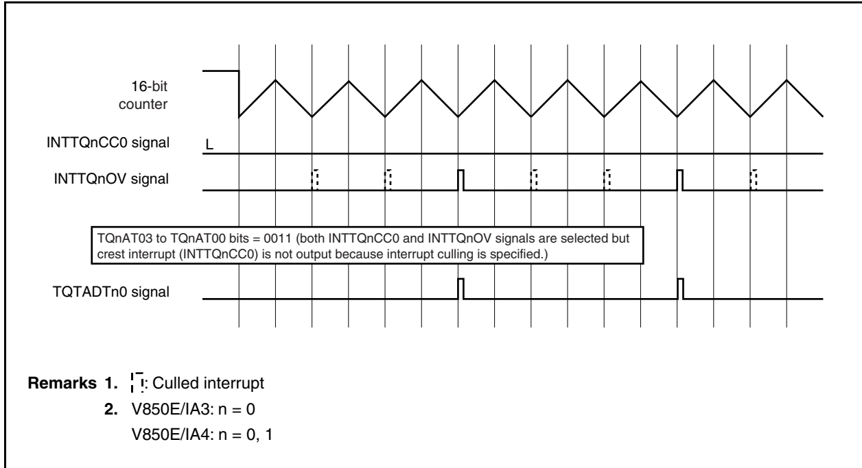
Figure 10-40. Example of A/D Conversion Start Trigger (TQTADTn0) Signal Output (TQnOPT1.TQnICE Bit = 0, TQnOPT1.TQnIOE Bit = 1, TQnOPT1.TQnID4 to TQnOPT1.TQnID0 Bits = 00010: With Interrupt Culling) (2)
