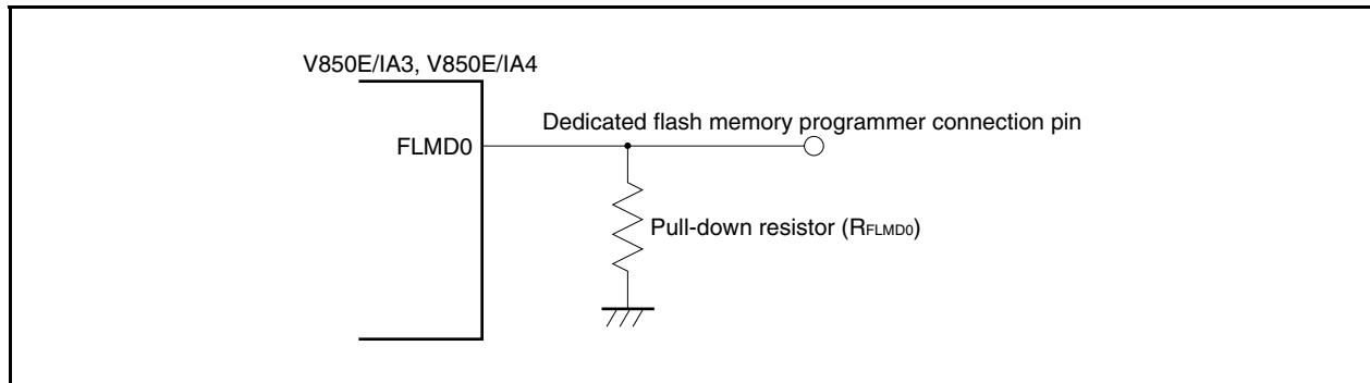
Figure 22-7. FLMD0 Pin Connection Example
