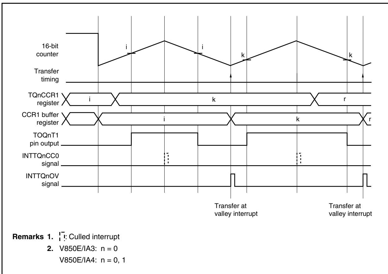
Figure 10-35. Rewriting TQnCCR1 Register
