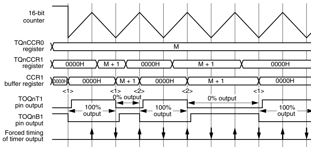
<R> Figure 10-11. PWM Output Waveform from 0% to 100% and from 100% to 0% (With Dead Time)
