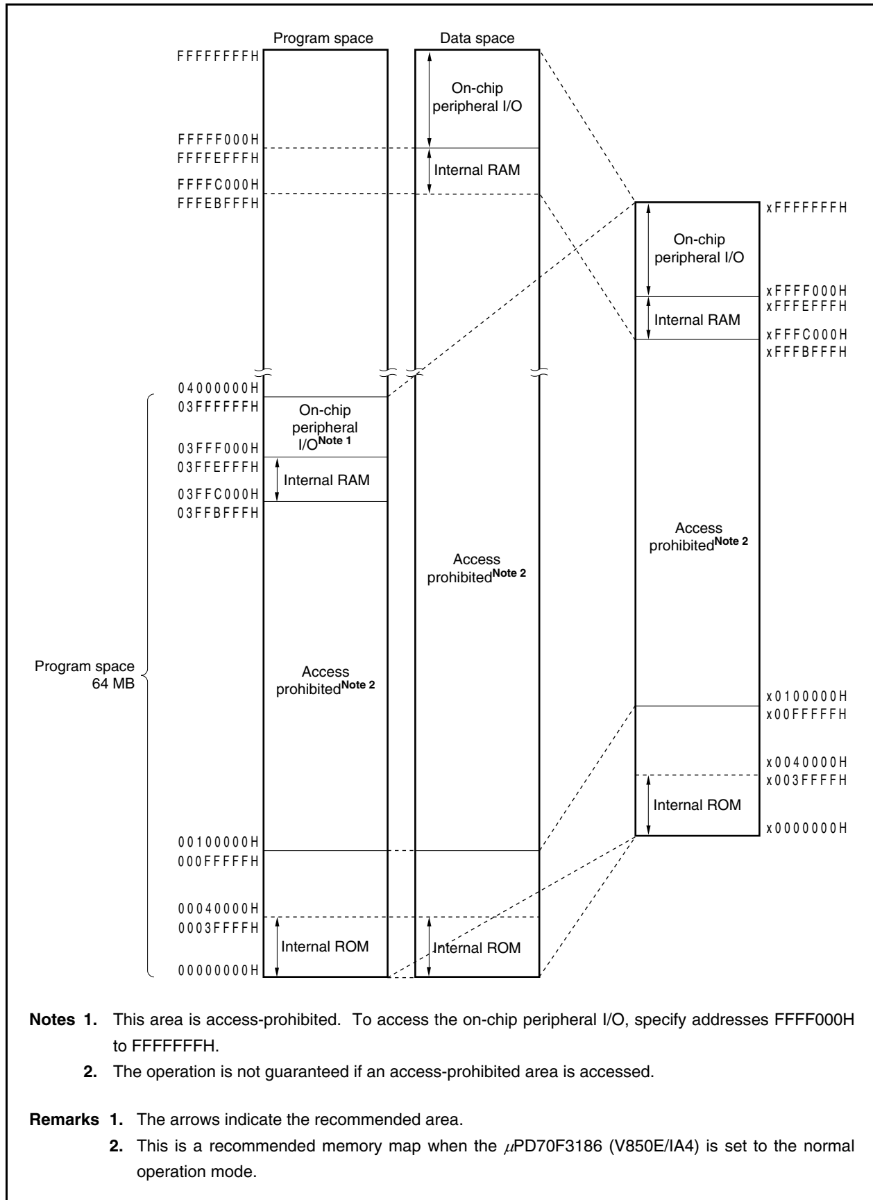
Figure 3-10. Recommended Memory Map
