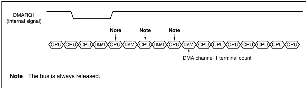
Figure 16-6. Single-Step Transfer Example 2
