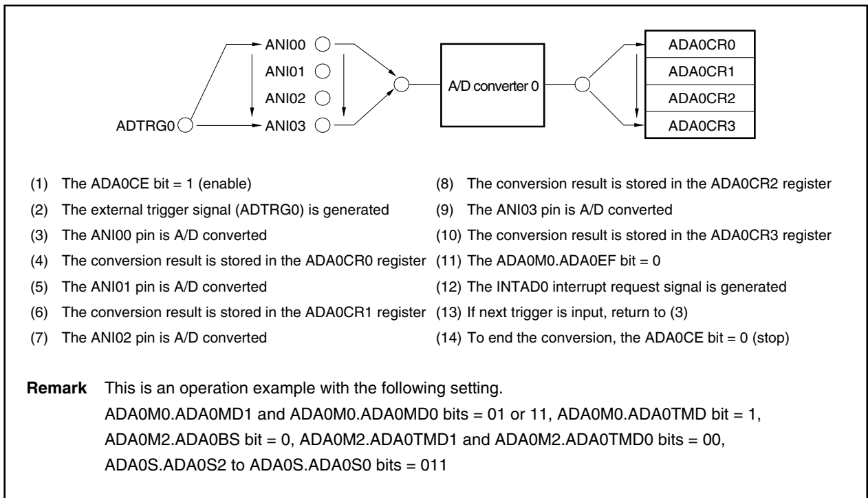
Figure 12-22. Example of Scan Mode Operation (Continuous Scan/One-Shot Scan by External Trigger): V850E/IA4
