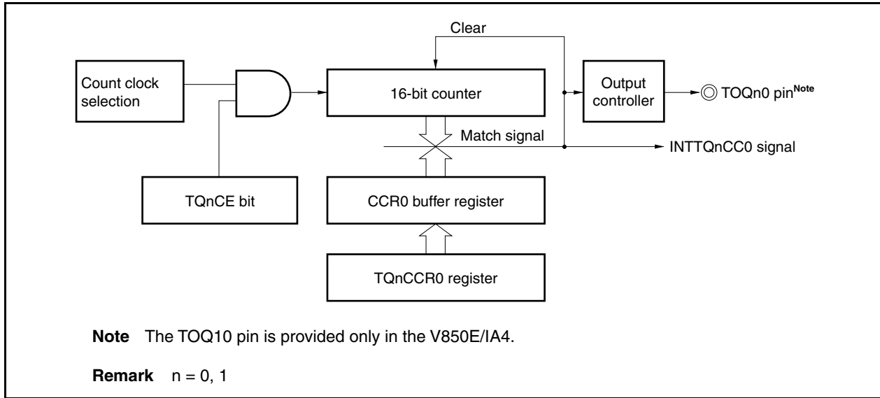
Figure 7-7. Interval Timer Configuration
