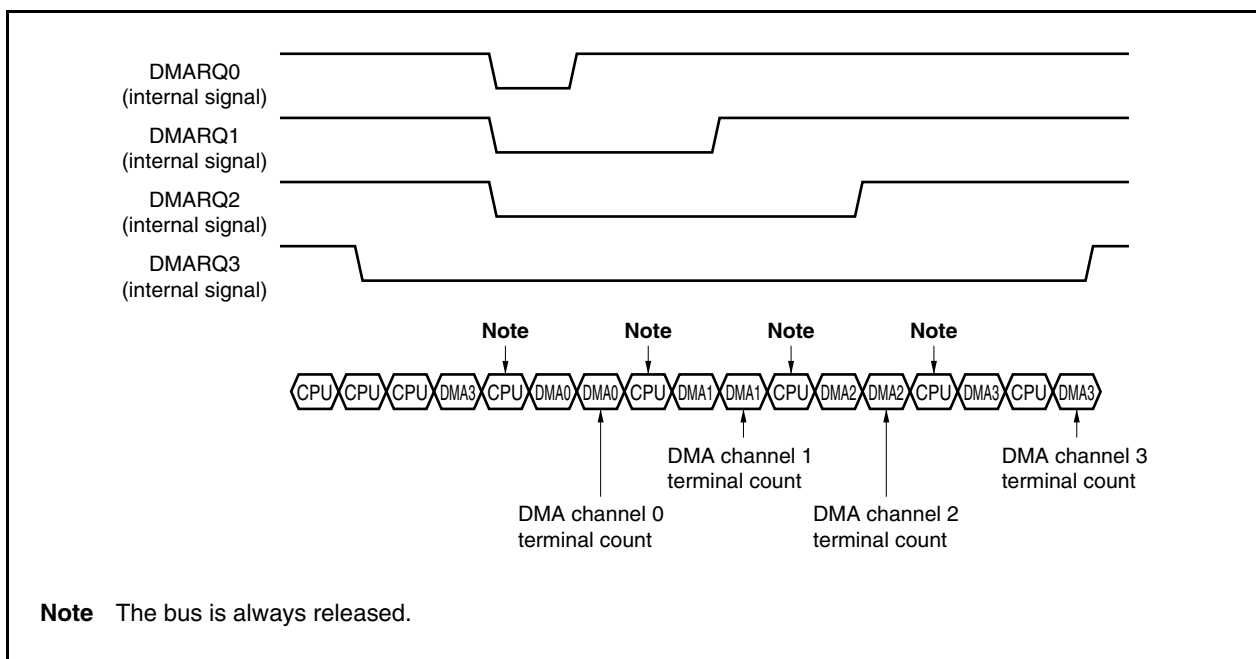
Figure 16-2. Single Transfer Example 2
