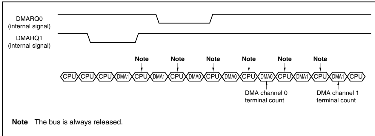
Figure 16-6. Single-Step Transfer Example 2
