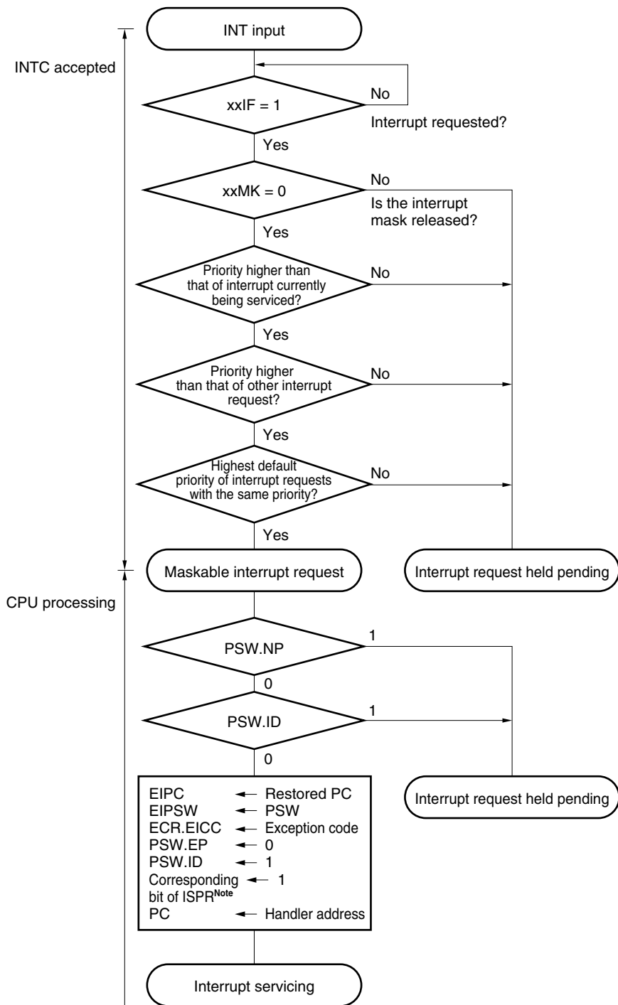
Figure 17-4. Maskable Interrupt Servicing
