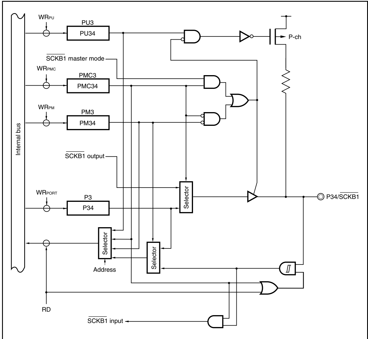
Figure 4-15. Block Diagram of P34 Pin
