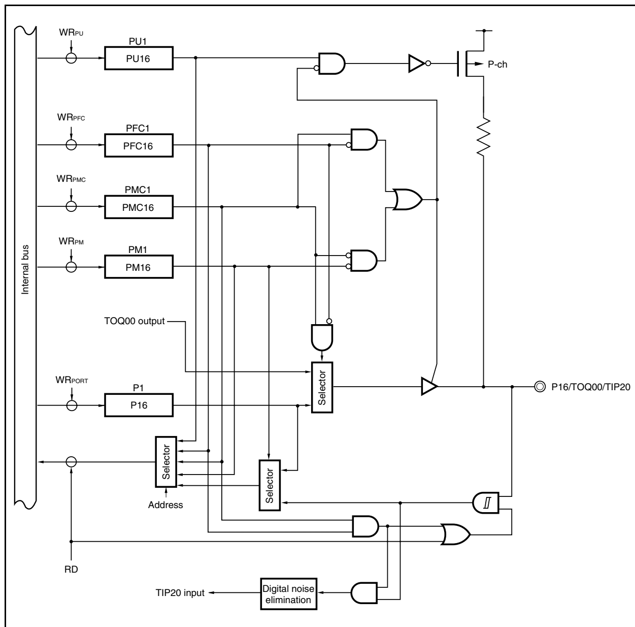
Figure 4-8. Block Diagram of P16 Pin
