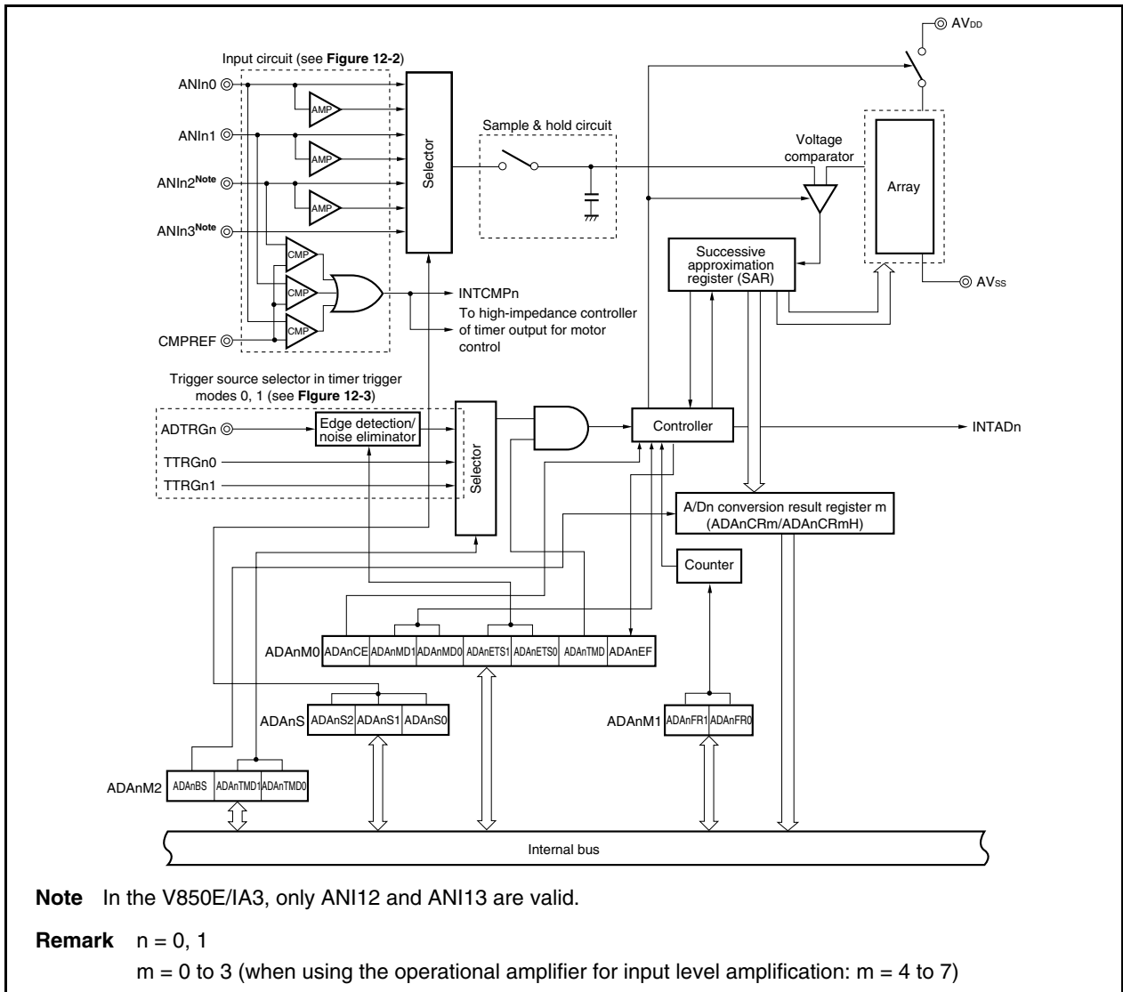
Figure 12-1. Block Diagram of A/D Converters 0 and 1
