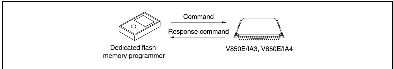
Figure 22-6. Communication Commands
