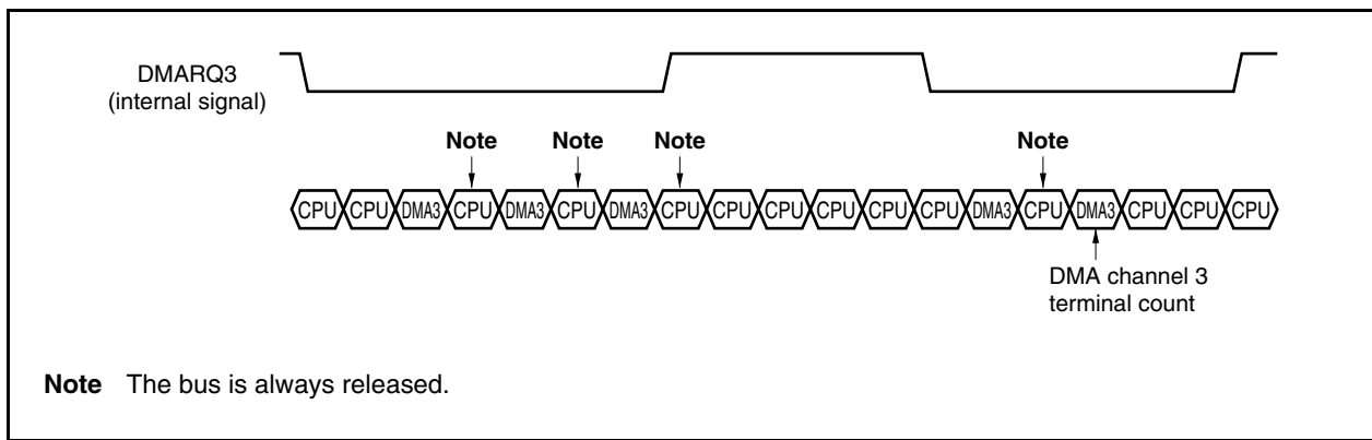
Figure 16-1. Single Transfer Example 1
