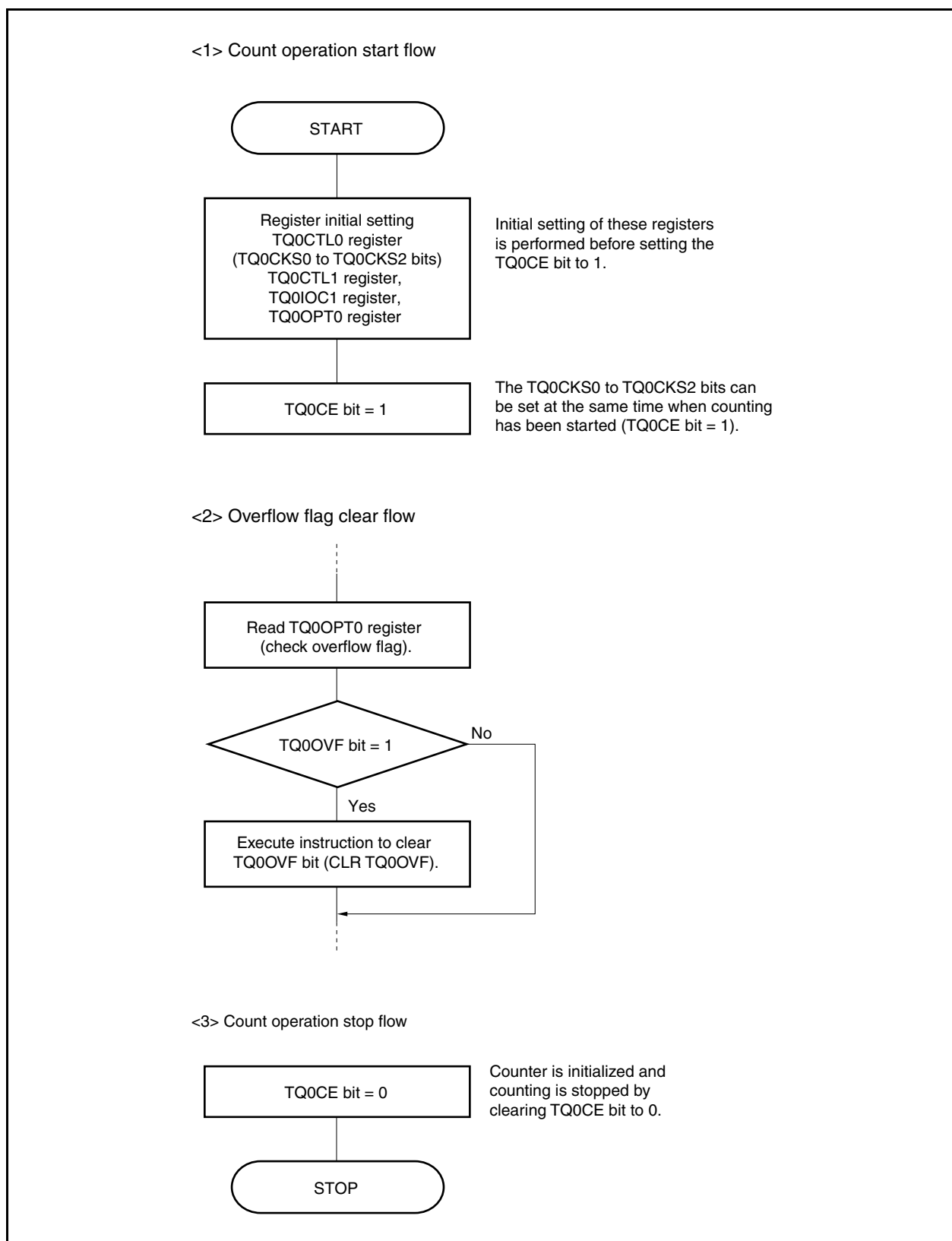
Figure 7-38. Software Processing Flow in Free-Running Timer Mode (Capture Function) (2/2)
