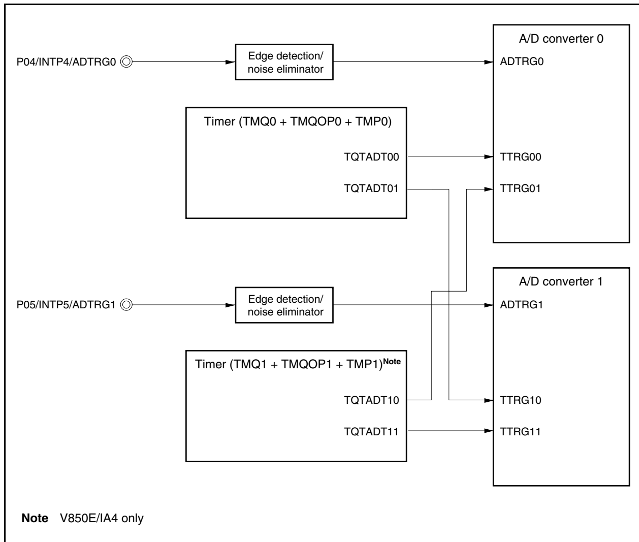
Figure 12-3. Block Diagram of Trigger Source Selector in Timer Trigger Modes 0 and 1
