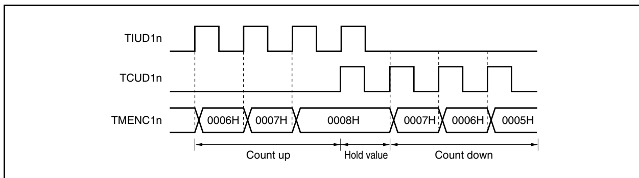
Figure 8-6. Mode 2 (When Rising Edge Is Specified as Valid Edge of TIUD1n, TCUD1n Pins)
