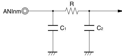
Figure 12-23. ANInm Pin Internal Equivalent Circuit
