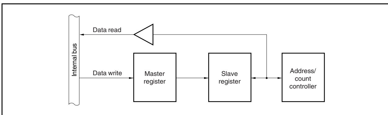
Figure 16-8. Buffer Register Configuration
