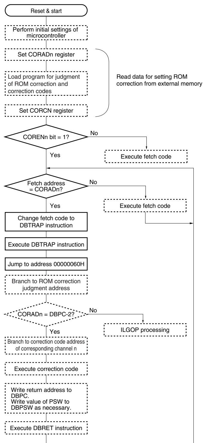
Figure 20-2. ROM Correction Operation and Program Flow
