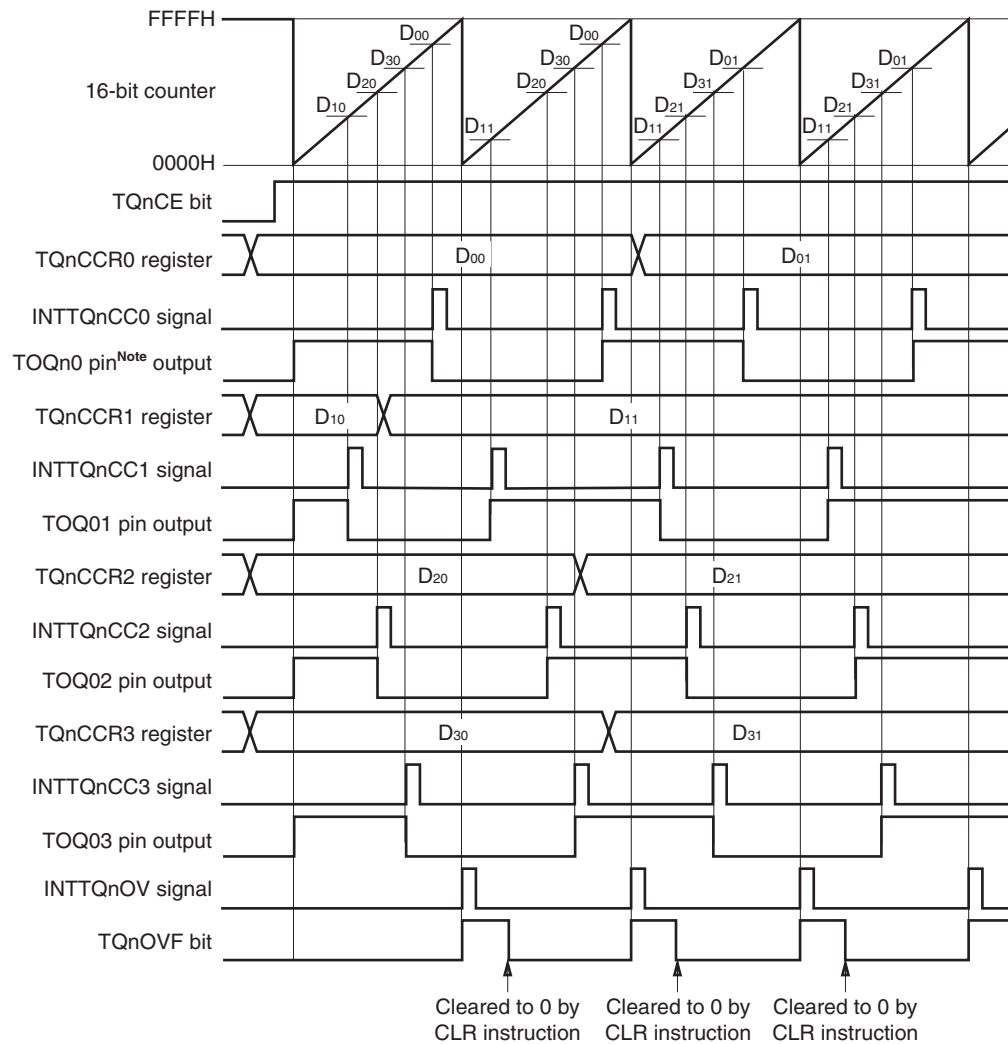
Figure 7-34. Basic Timing in Free-Running Timer Mode (Compare Function)
