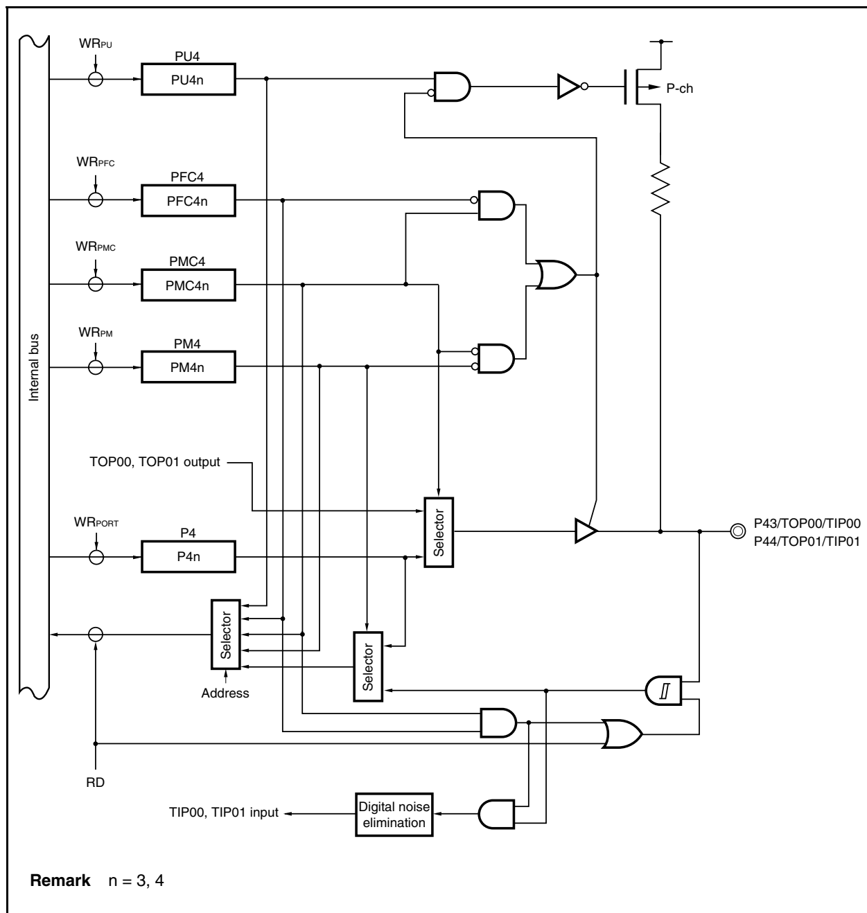
Figure 4-21. Block Diagram of P43 and P44 Pins
