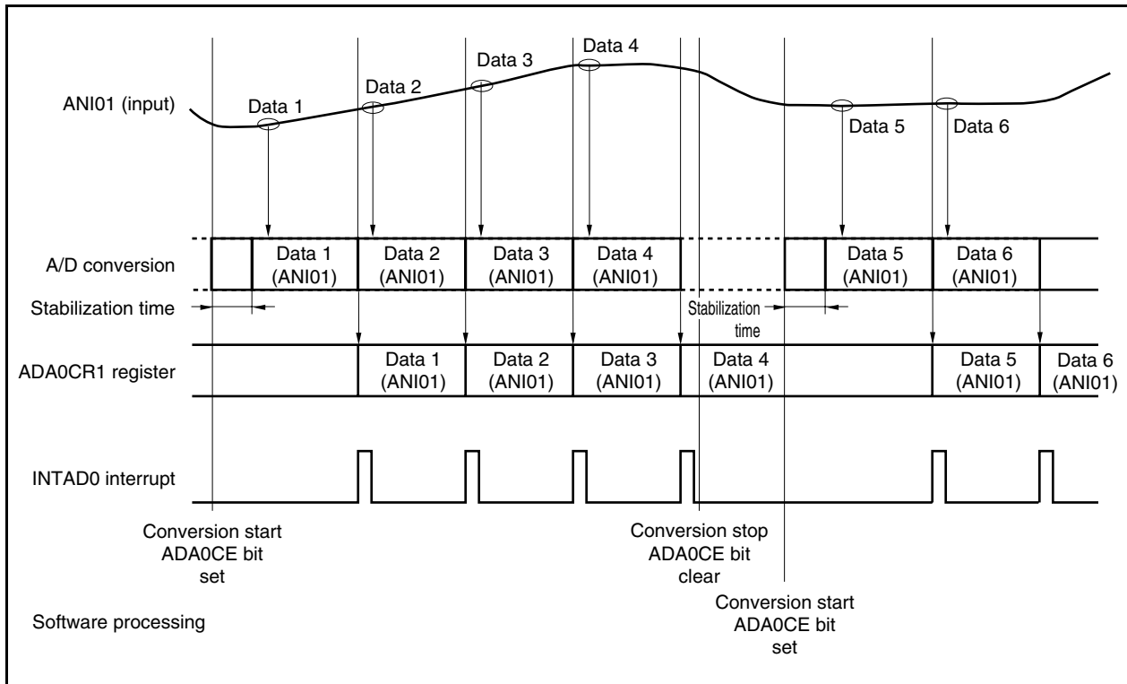
Figure 12-5. Continuous Select 1-Buffer Mode Operation Timing (When ADA0M0.ADA0MD1 and ADA0M0.ADA0MD0 Bits = 00, ADA0M2.ADA0BS Bit = 0, ADA0S.ADA0S2 to ADA0S.ADA0S0 Bits = 001): V850E/IA4
