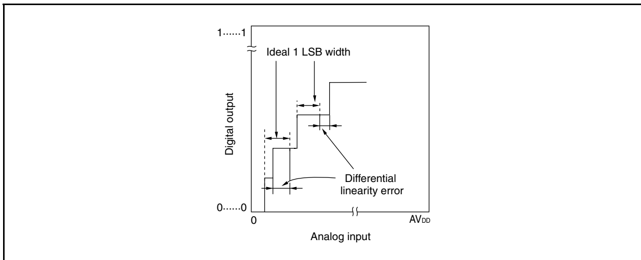
Figure 12-29. Differential Linearity Error
