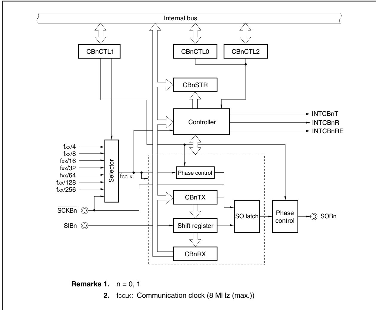
Figure 15-2. Block Diagram of CSIBn
