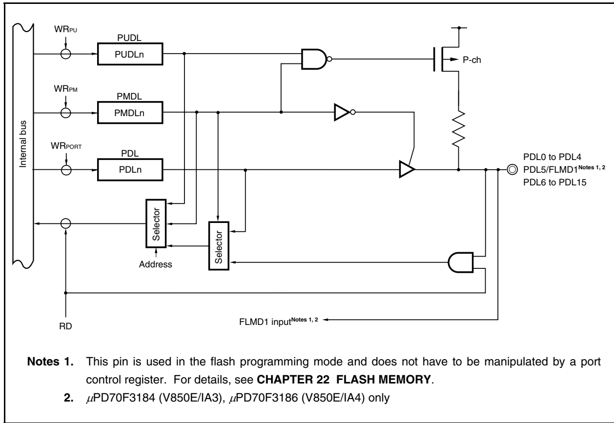
Figure 4-25. Block Diagram of PDL0 to PDL15 Pins
