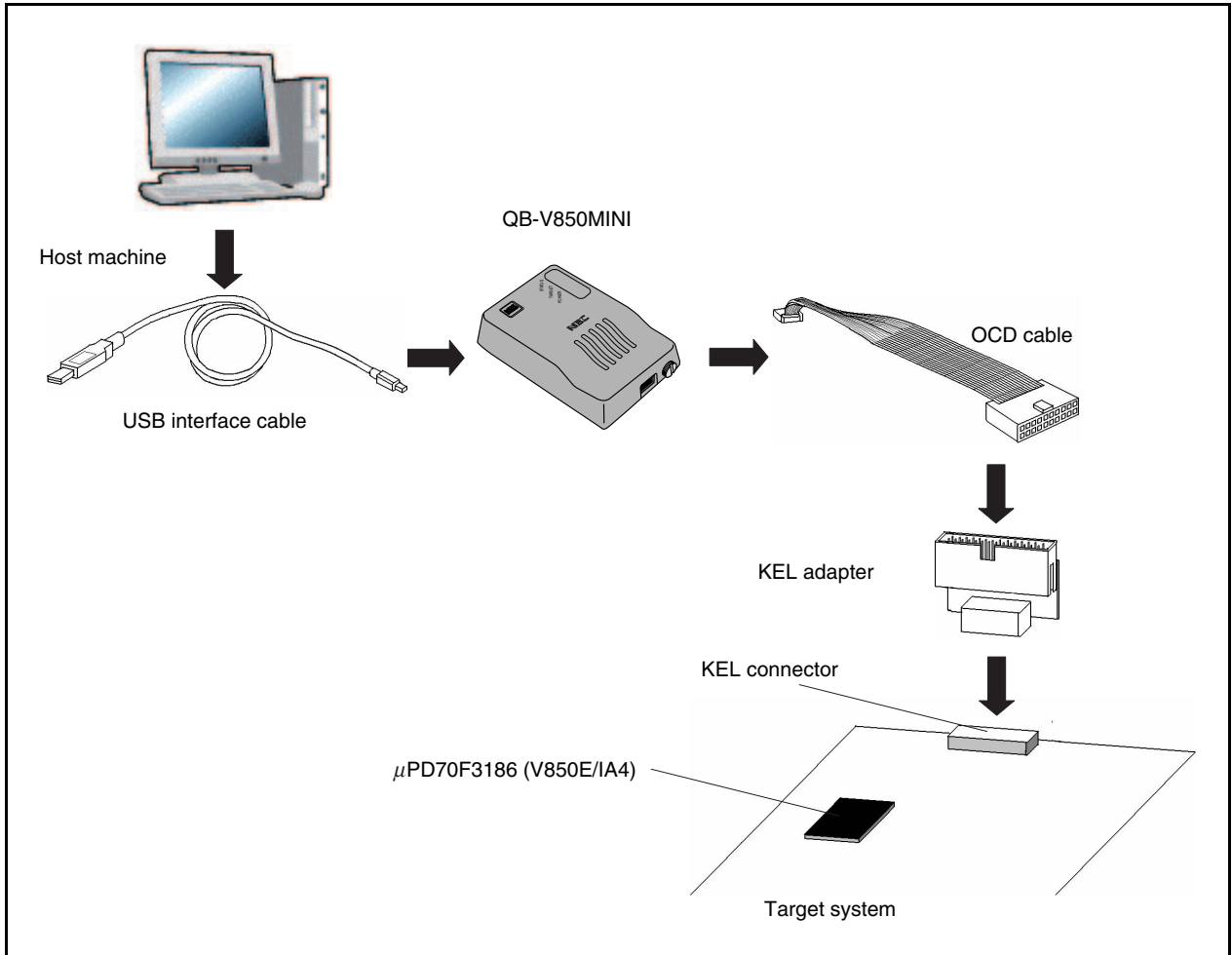
<R> Figure 21-1. Connecting On-Chip Debug Emulator (QB-V850MINI)
