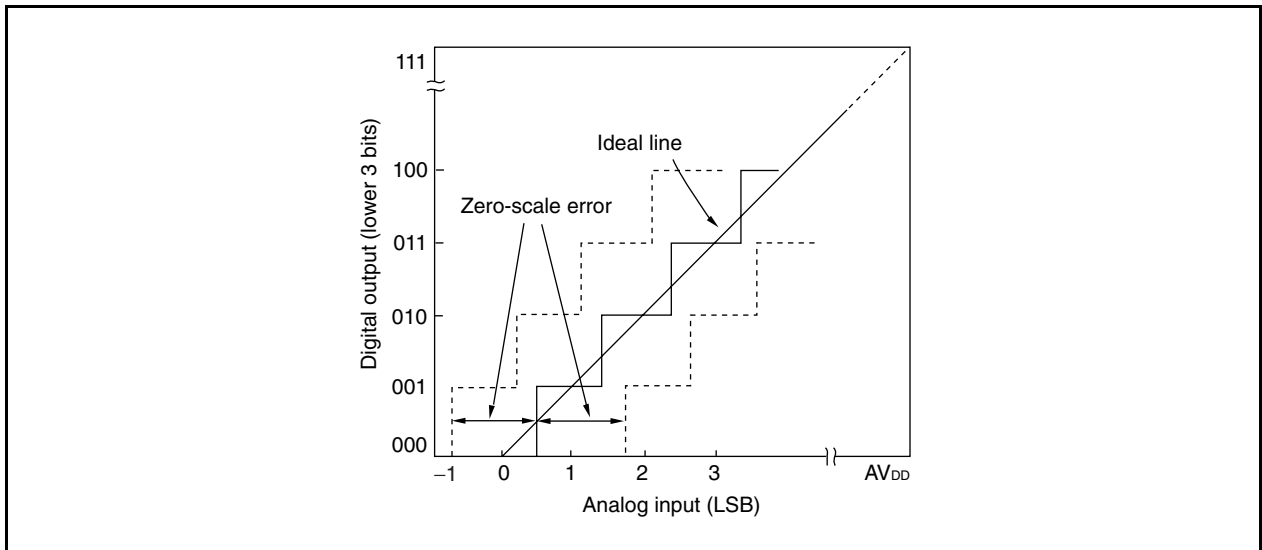
Figure 12-27. Zero-Scale Error
