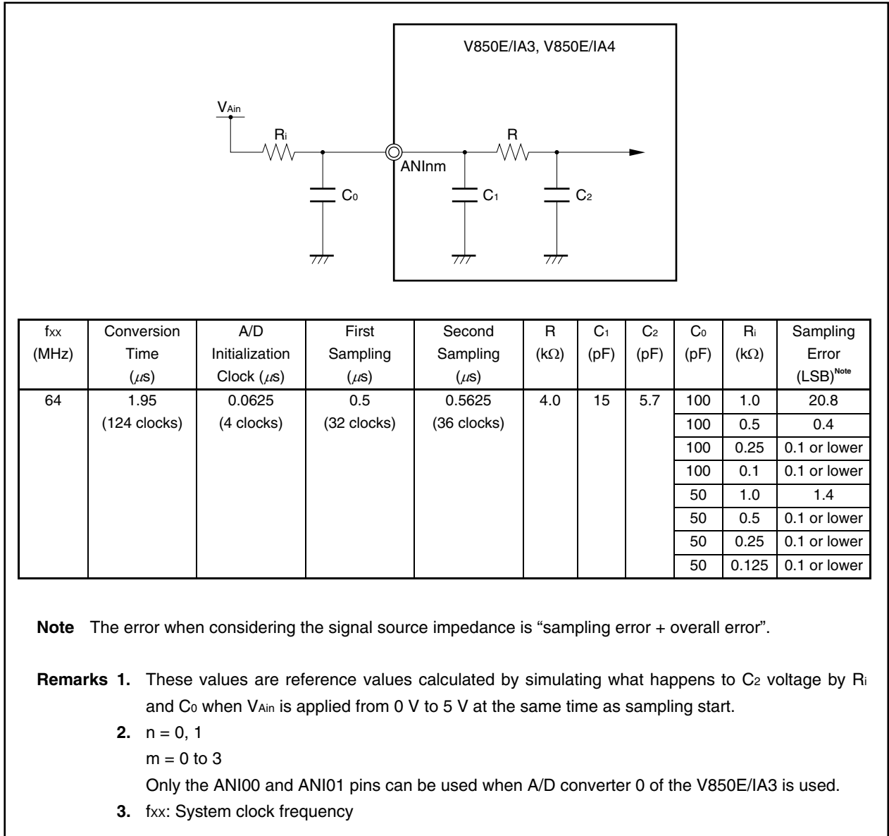
Figure 12-24. Example of Calculating Overall Error of A/D Converters 0 and 1
