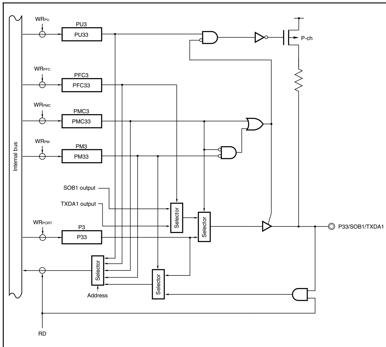
Figure 4-14. Block Diagram of P33 Pin
