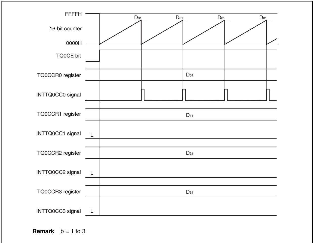
Figure 7-20. Timing Chart When D_{01} < D_{b1}
