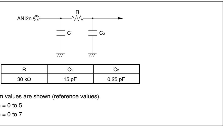
Figure 13-8. ANI2n Pin Internal Equivalent Circuit
