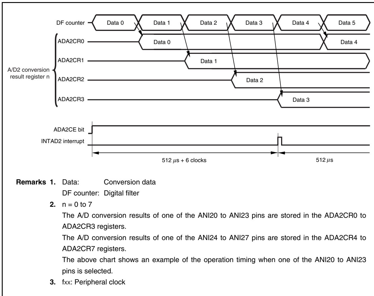
Figure 13-6. Example of Operation Timing in 4-Buffer Serial Mode (with 8-Bit Resolution, f xx = 64 MHz)
