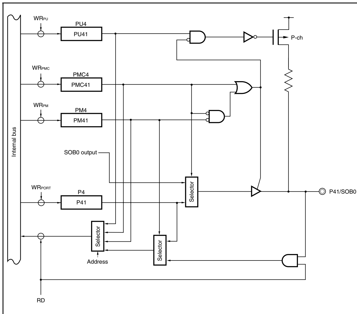
Figure 4-19. Block Diagram of P41 Pin
