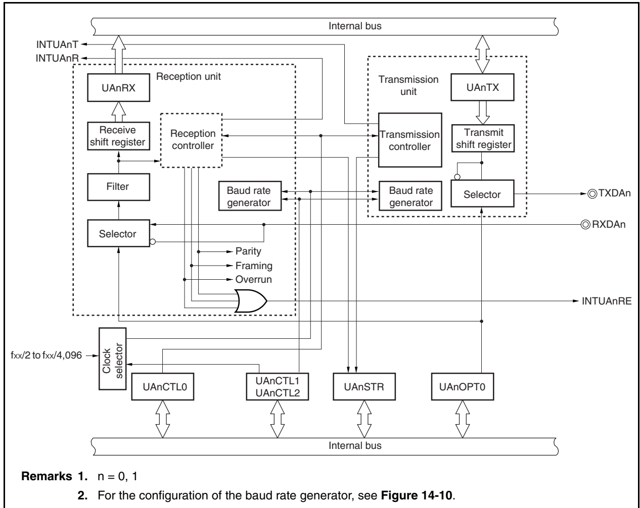
Figure 14-2. Block Diagram of UARTAn
