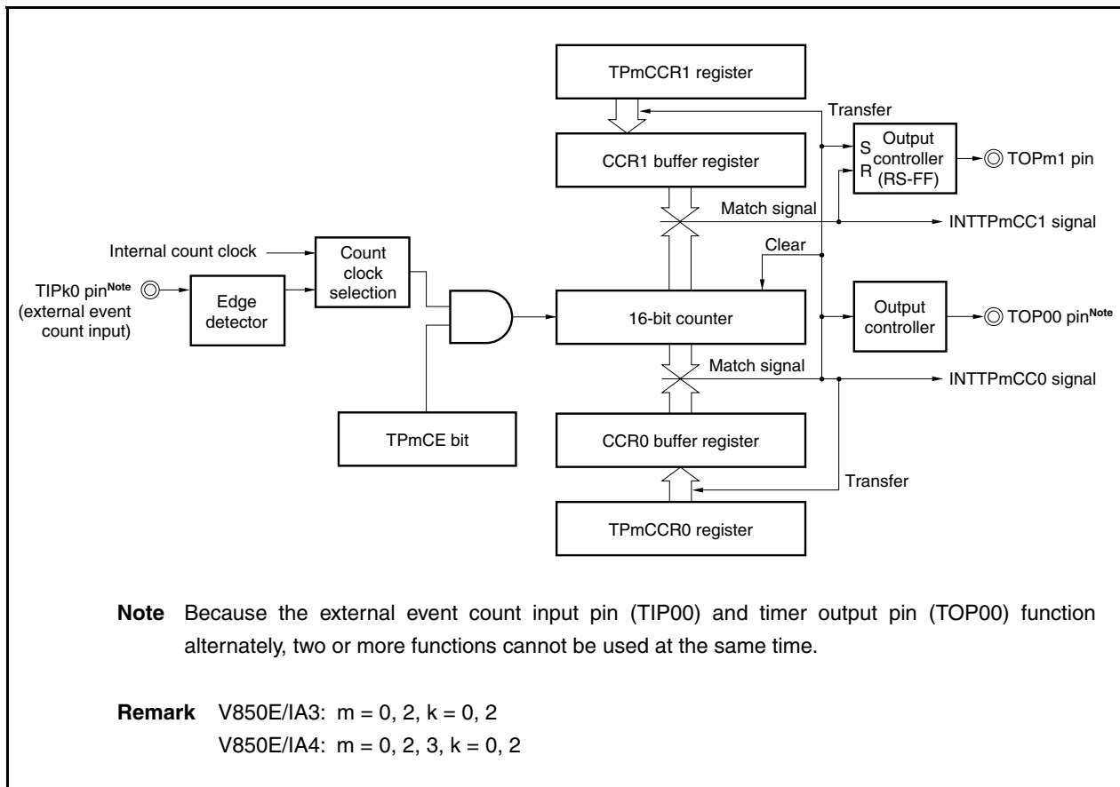
Figure 6-31. Configuration in PWM Output Mode
