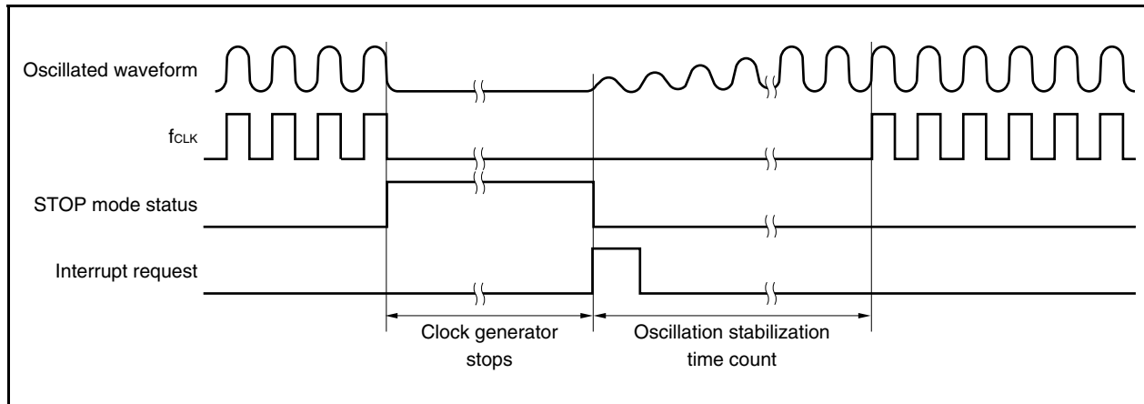
Figure 18-2. Oscillation Stabilization Time
