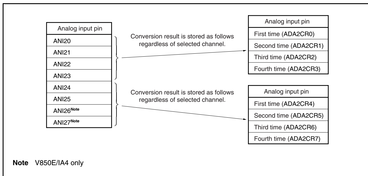
Figure 13-2. Correspondence Between Analog Input Pin and ADA2CRn Register in 4-Buffer Mode
