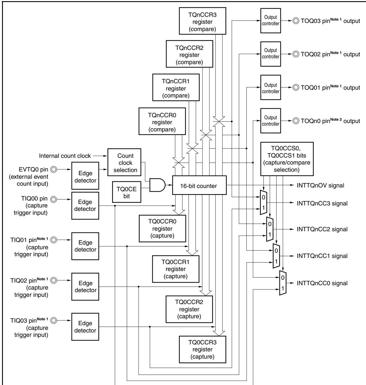
Figure 7-33. Configuration in Free-Running Timer Mode
