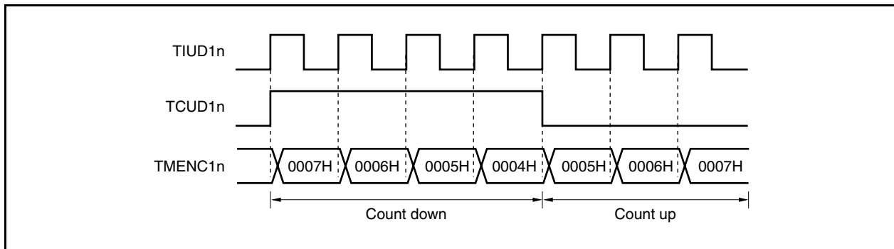
Figure 8-5. Mode 1 (When Rising Edge Is Specified as Valid Edge of TIUD1n Pin): In Case of Simultaneous TIUD1n, TCUD1n Pin Edge Timing
