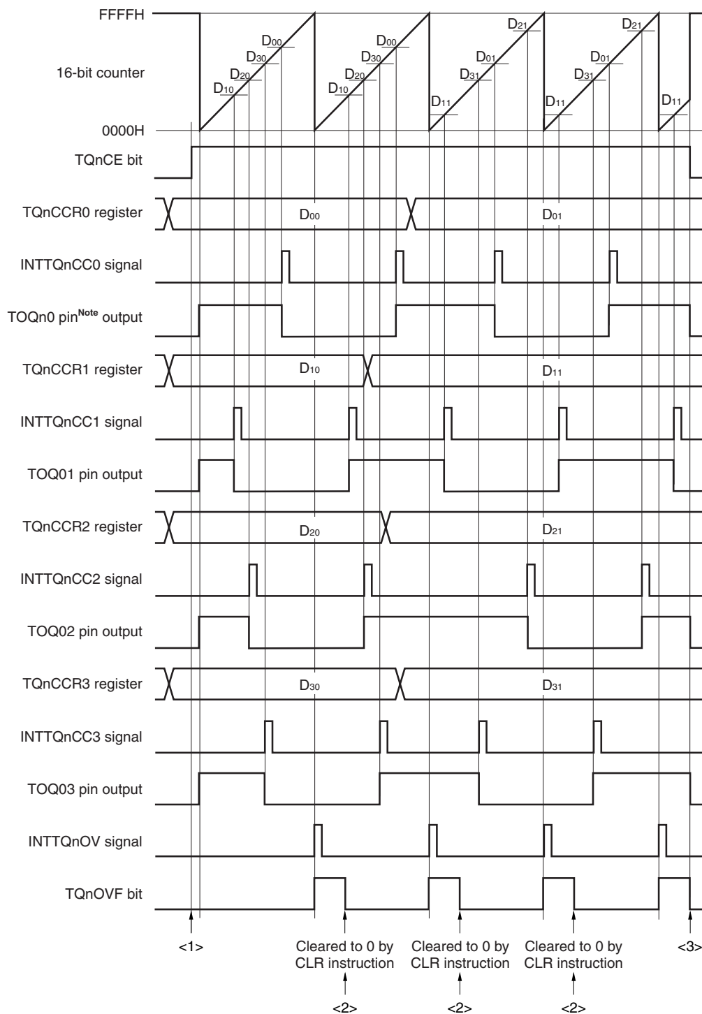
Figure 7-37. Software Processing Flow in Free-Running Timer Mode (Compare Function) (1/2)
