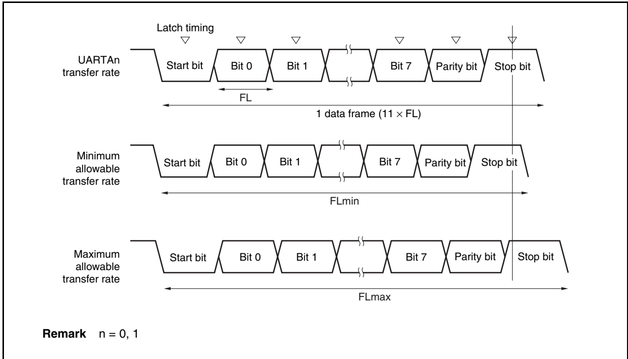
Figure 14-11. Allowable Baud Rate Range During Reception
