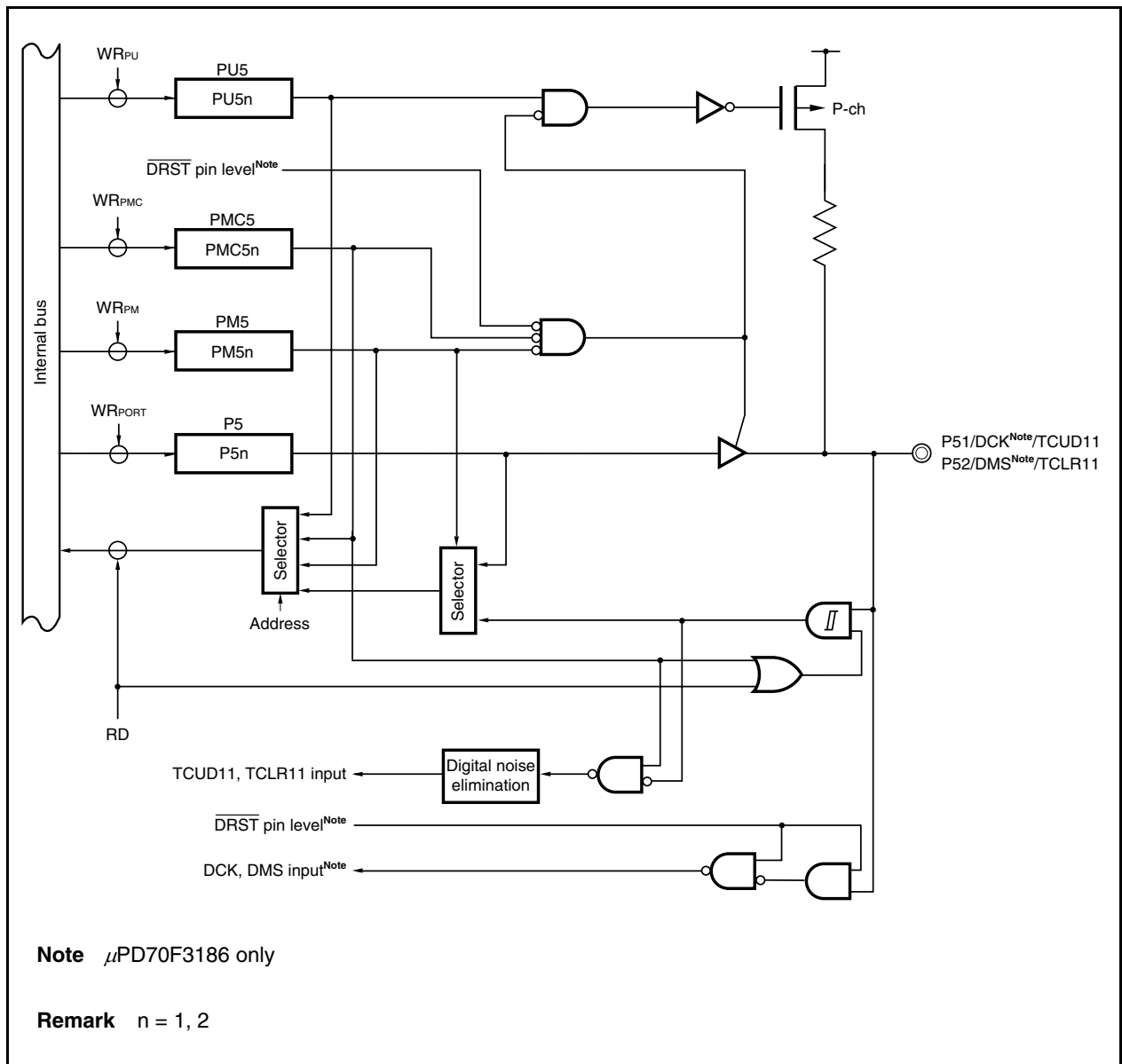
Figure 4-23. Block Diagram of P51 and P52 Pins
