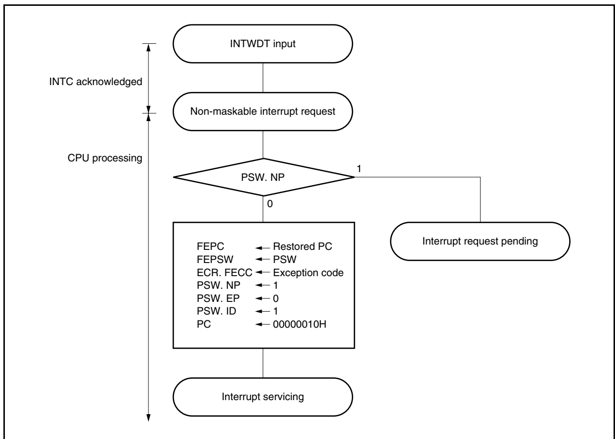
Figure 17-1. Non-Maskable Interrupt Servicing
