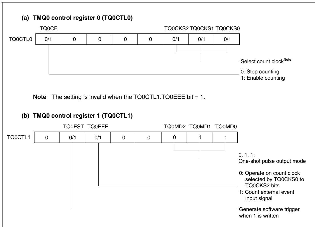
Figure 7-27. Register Setting in One-Shot Pulse Output Mode (1/3)
