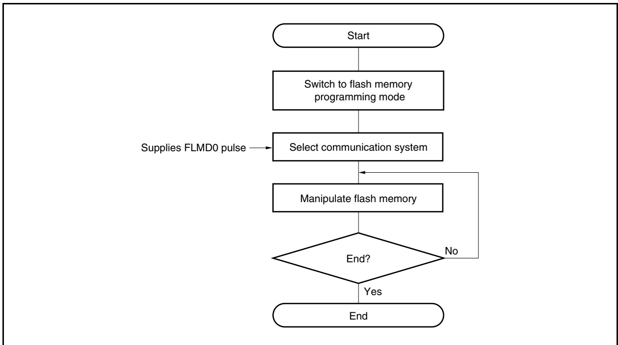
Figure 22-4. Procedure for Manipulating Flash Memory
