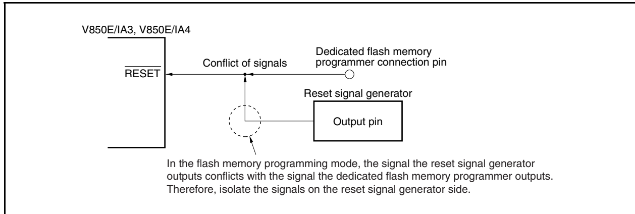
Figure 22-11. Conflict of Signals ( \overline{\text{RESET}} Pin)
