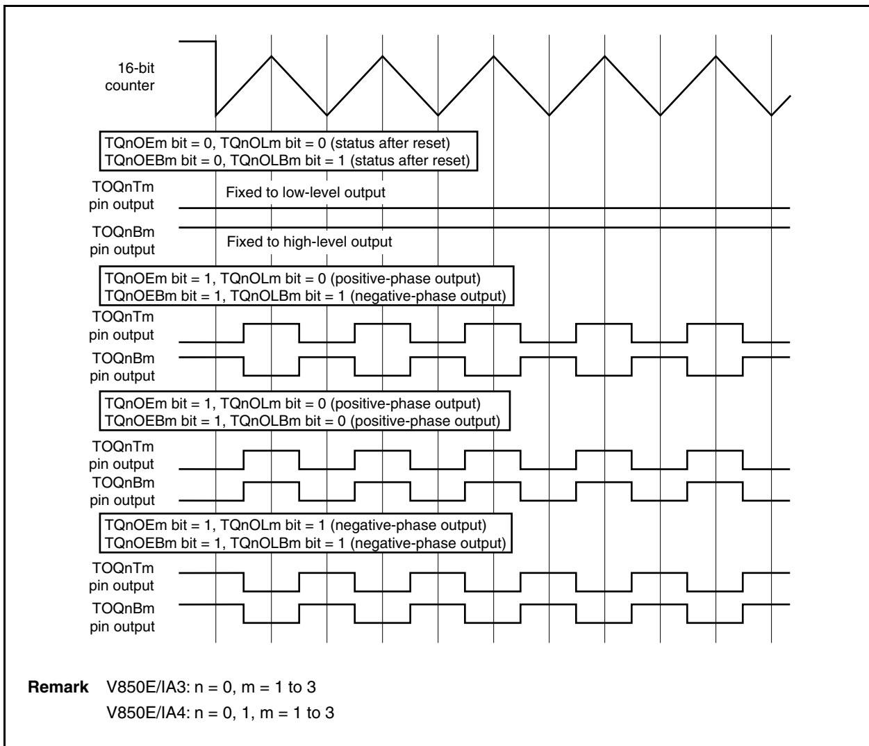
Figure 10-3. TOQnTm and TOQnBm Pin Output Control (Without Dead Time)
