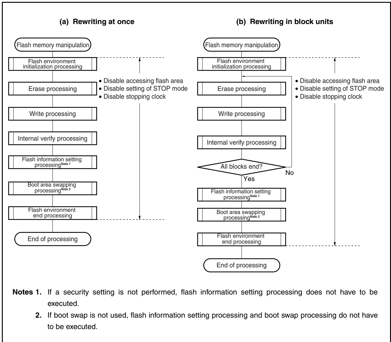
Figure 22-14. Standard Self Programming Flow
