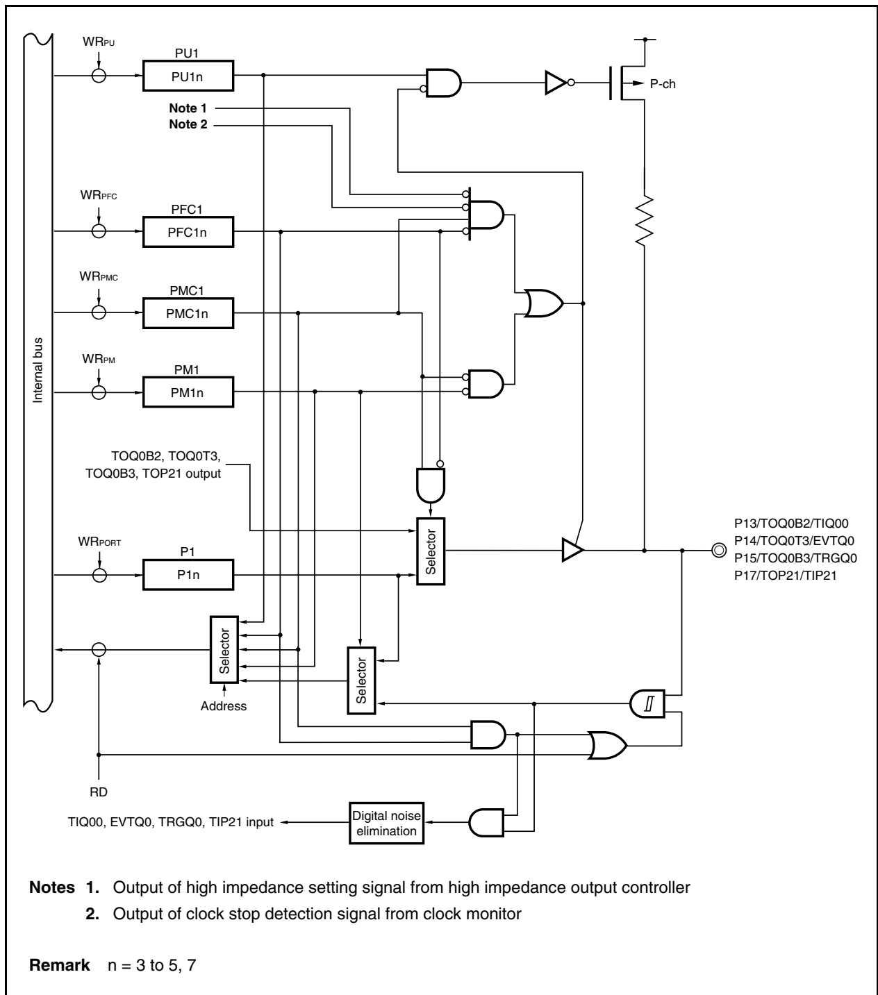
Figure 4-7. Block Diagram of P13 to P15 and P17 Pins
