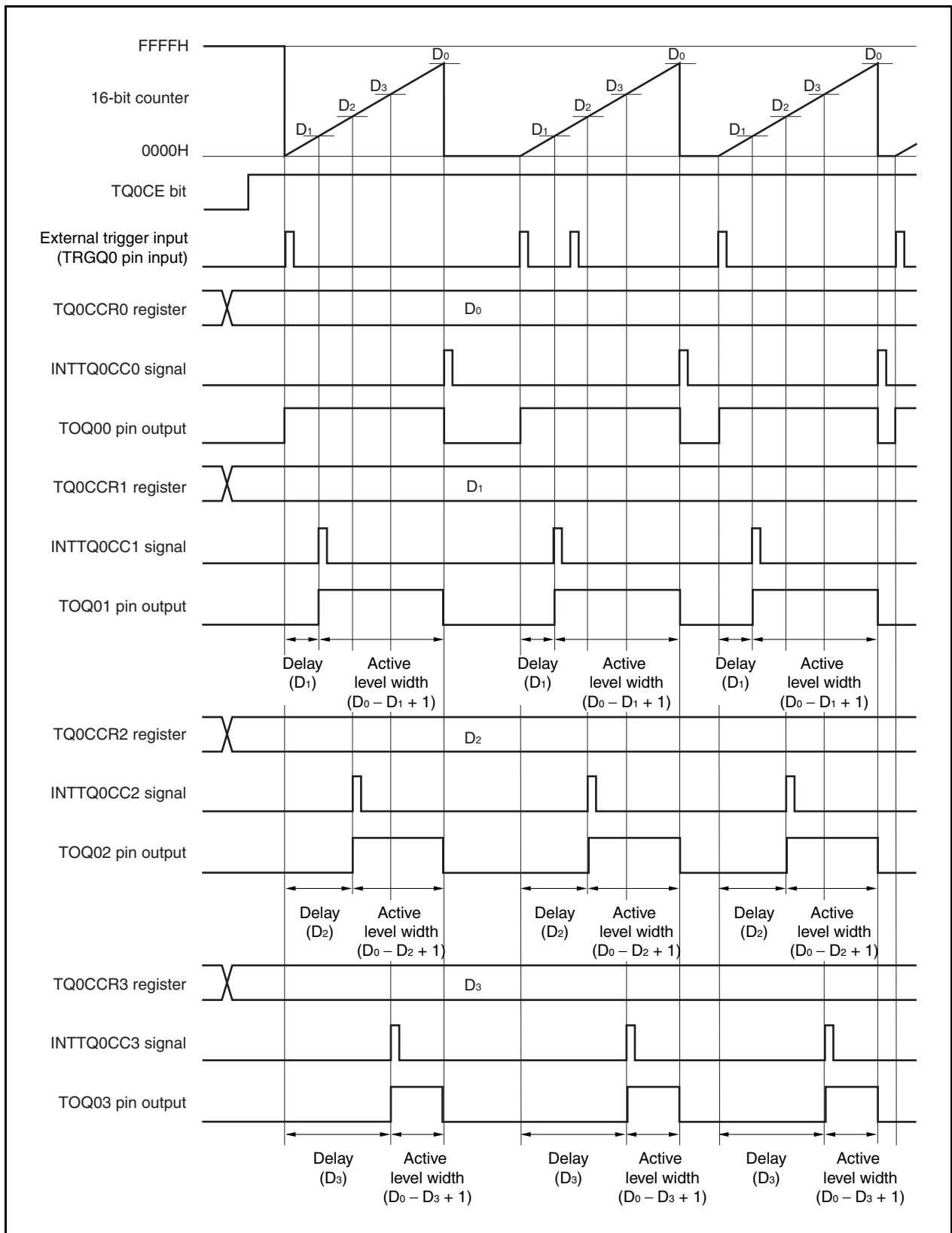
Figure 7-26. Basic Timing in One-Shot Pulse Output Mode
