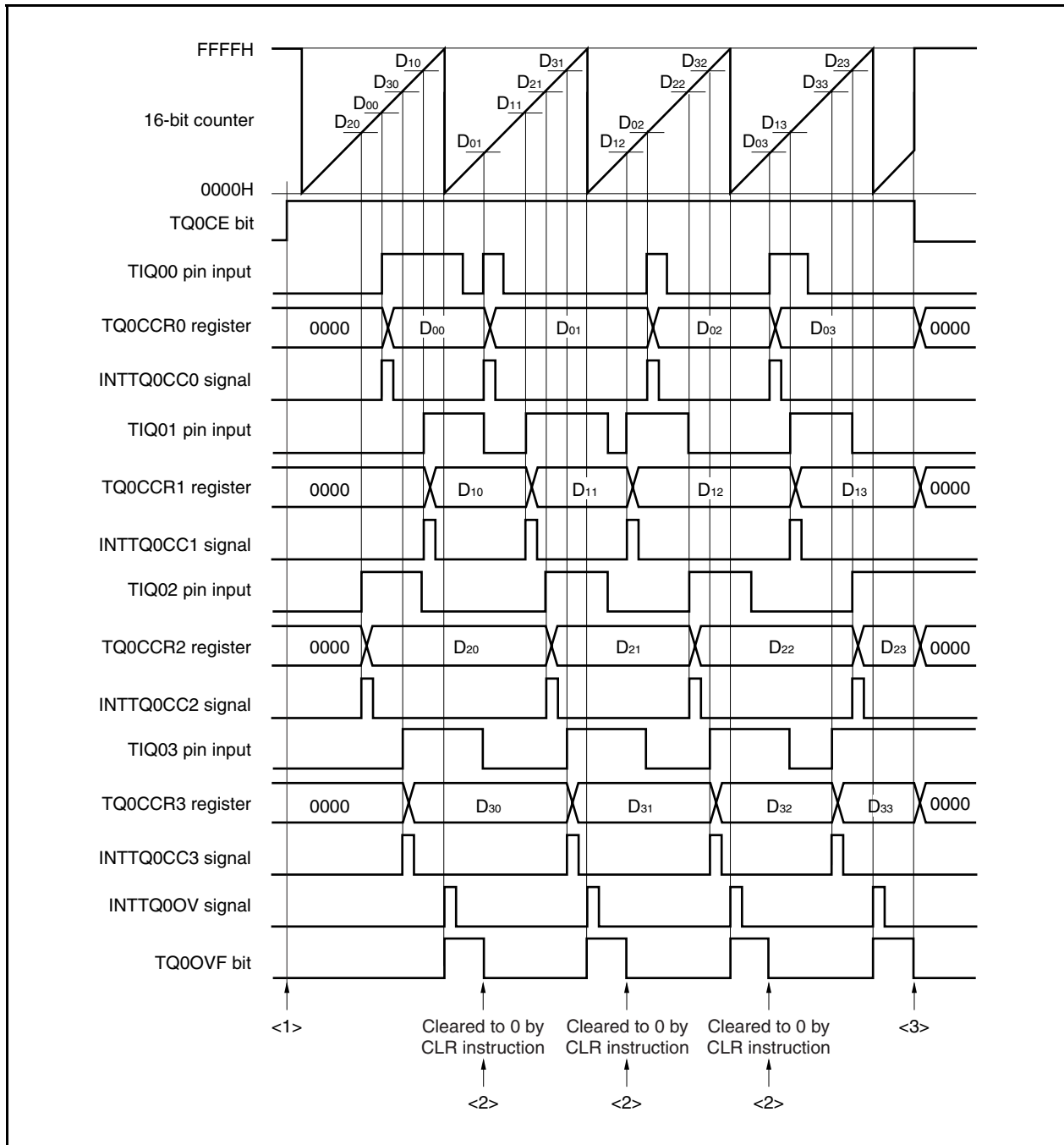
Figure 7-38. Software Processing Flow in Free-Running Timer Mode (Capture Function) (1/2)
