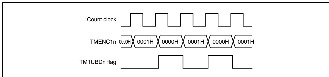
Figure 8-16. TM1UBDn Flag Operation
