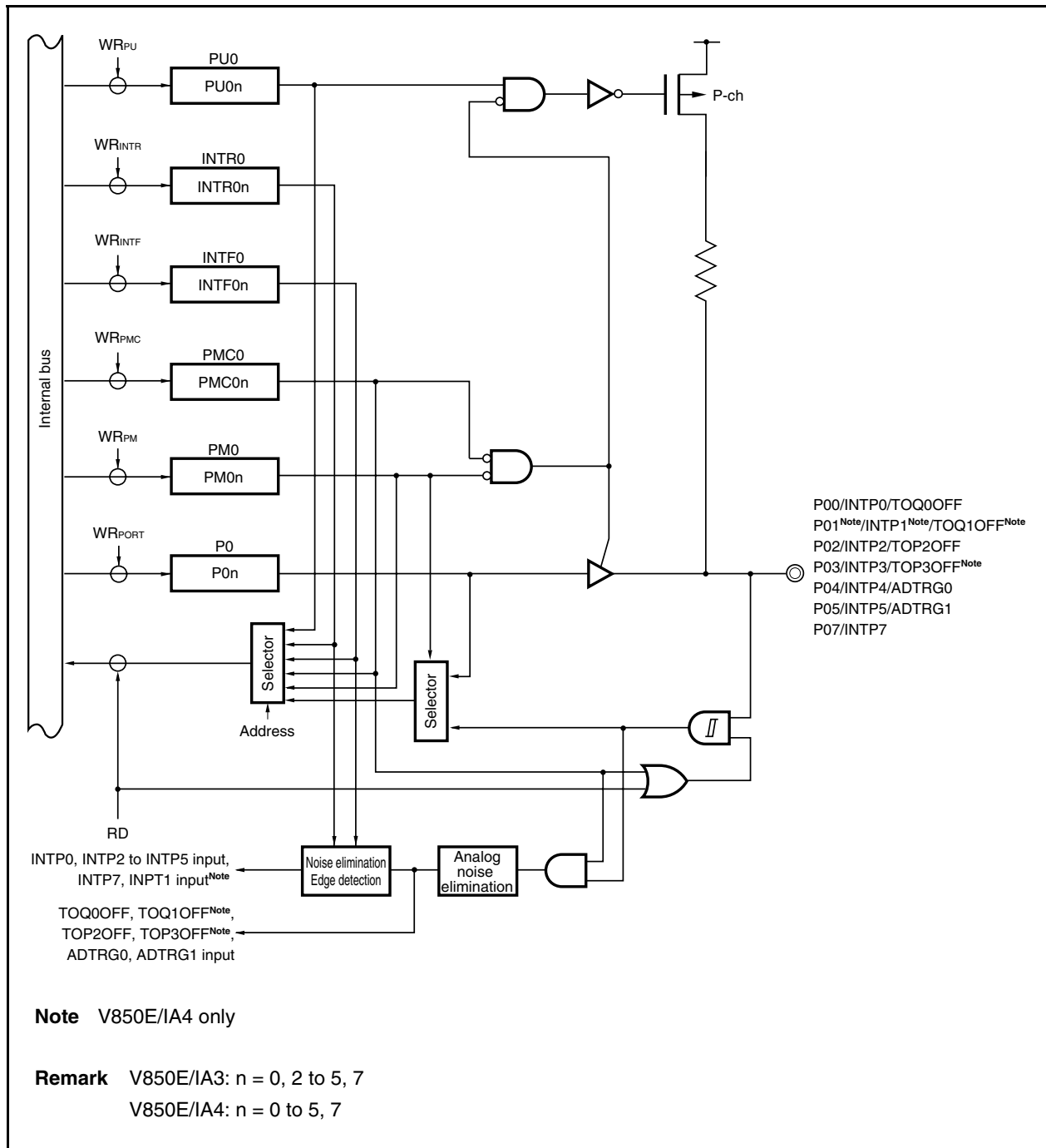
Figure 4-4. Block Diagram of P00 to P05 and P07 Pins
