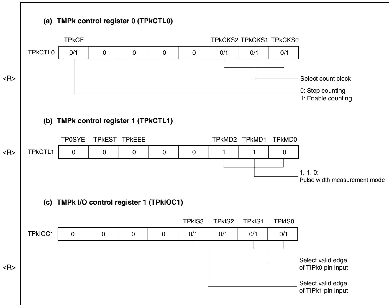
Figure 6-43. Register Setting in Pulse Width Measurement Mode (1/2)
