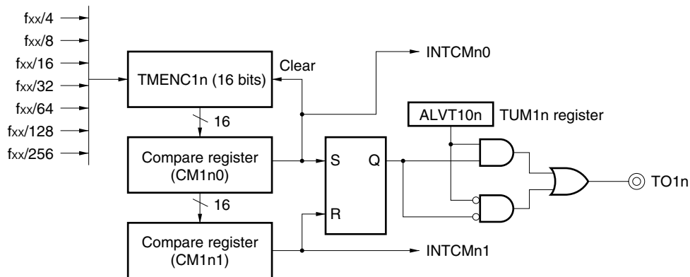
Figure 8-2. TMENC1n Block Diagram (During PWM Output Operation)
