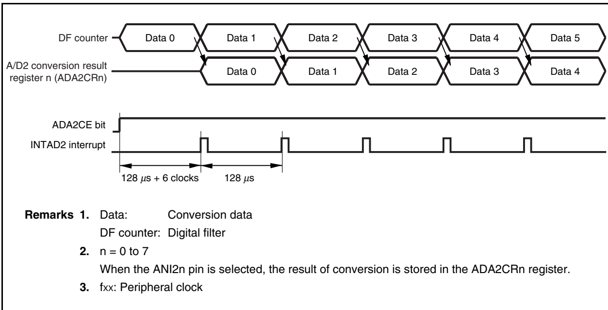
Figure 13-4. Example of Operation Timing in 1-Buffer Serial Mode (with 8-Bit Resolution, f xx = 64 MHz)
