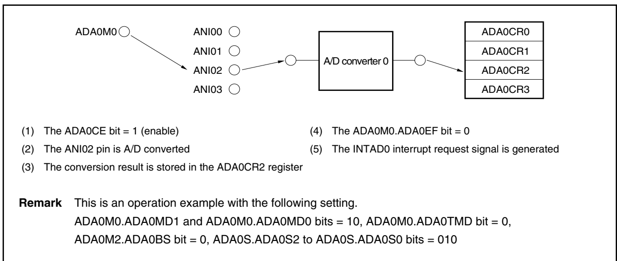
Figure 12-14. Example of 1-Buffer Mode Operation (1 Buffer of Software Trigger One-Shot Select): V850E/IA4
