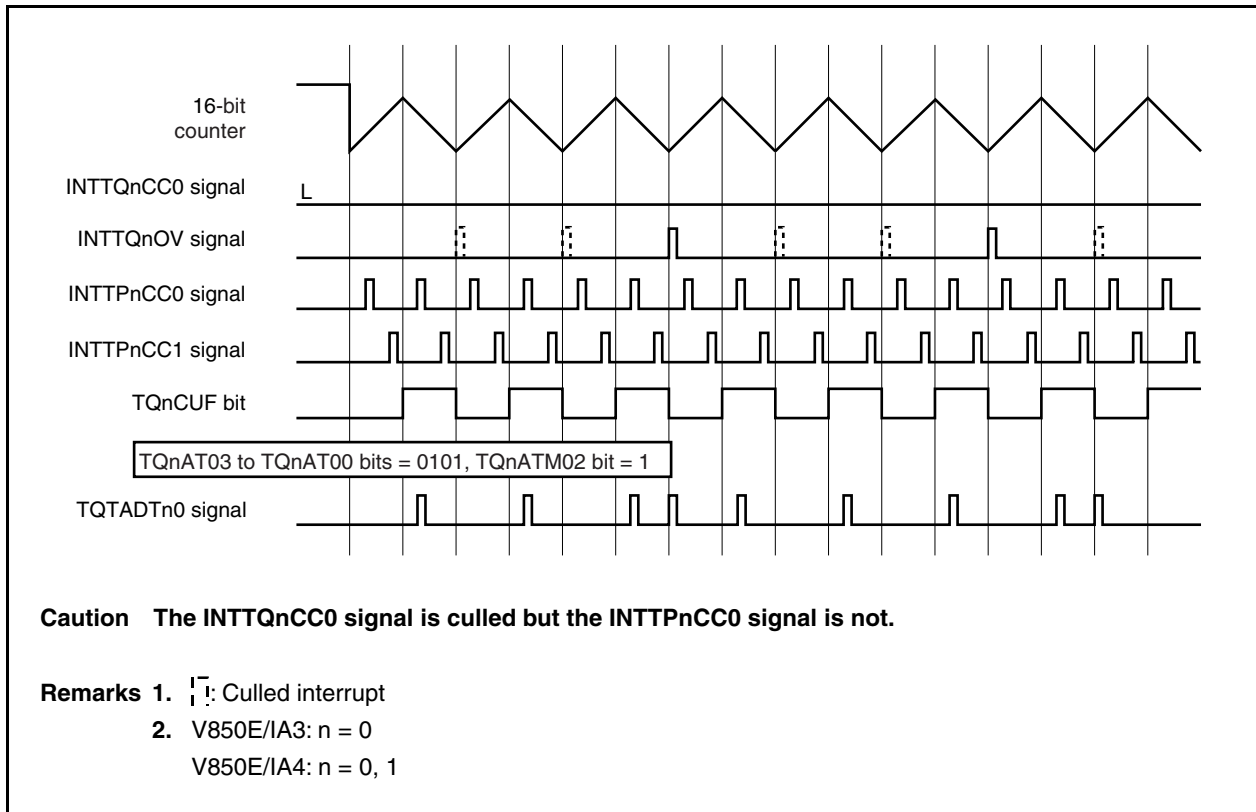
Figure 10-40. Example of A/D Conversion Start Trigger (TQTADTn0) Signal Output (TQnOPT1.TQnICE Bit = 0, TQnOPT1.TQnIOE Bit = 1, TQnOPT1.TQnID4 to TQnOPT1.TQnID0 Bits = 00010: With Interrupt Culling) (2)
