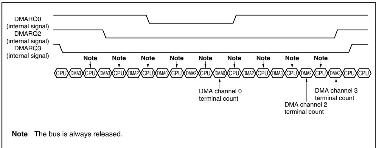
Figure 16-4. Single Transfer Example 4
