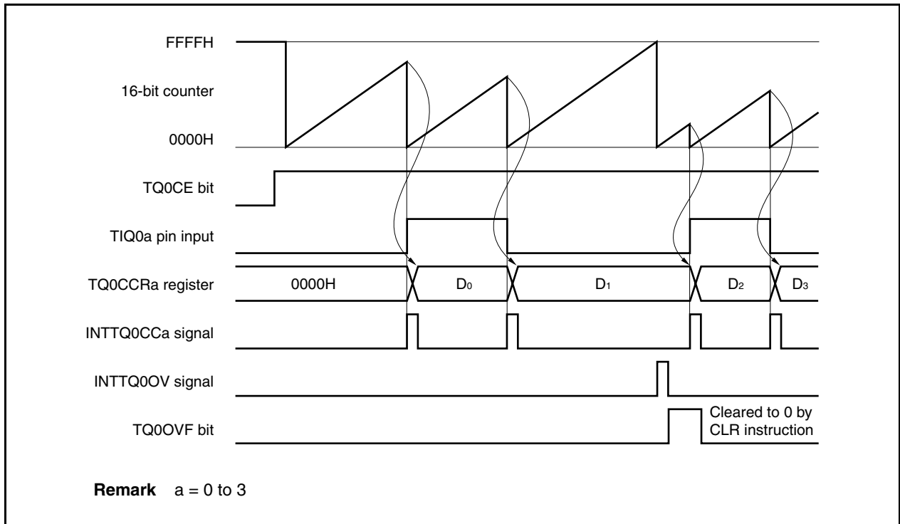
Figure 7-40. Basic Timing in Pulse Width Measurement Mode
