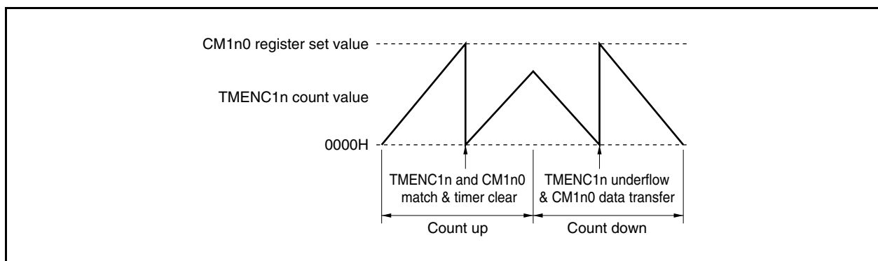
Figure 8-10. Example of TMENC1n Operation When Interval Operation and Transfer Operation Are Combined
