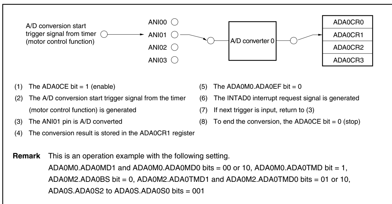
Figure 12-17. Example of 1-Buffer Mode Operation (1 Buffer of Continuous Select/One-Shot Select by Timer Trigger): V850E/IA4
