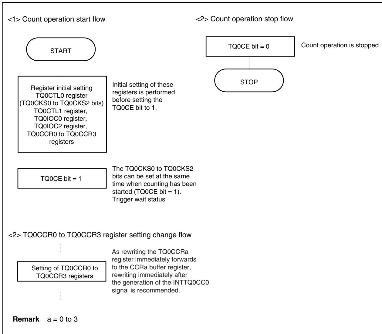
Figure 7-28. Software Processing Flow in One-Shot Pulse Output Mode (2/2)
