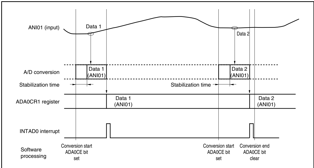
Figure 12-8. One-Shot Select 1-Buffer Mode Operation Timing (When ADA0M0.ADA0MD1 and ADA0M0.ADA0MD0 Bits = 10, ADA0M2.ADA0BS Bit = 0, ADA0S.ADA0S2 to ADA0S.ADA0S0 Bits = 001): V850E/IA4
