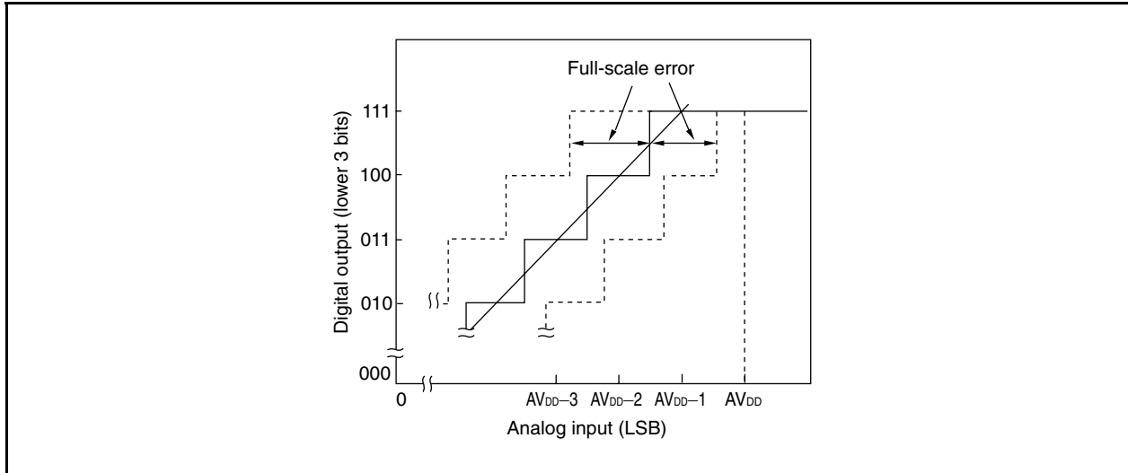
Figure 12-28. Full-Scale Error
