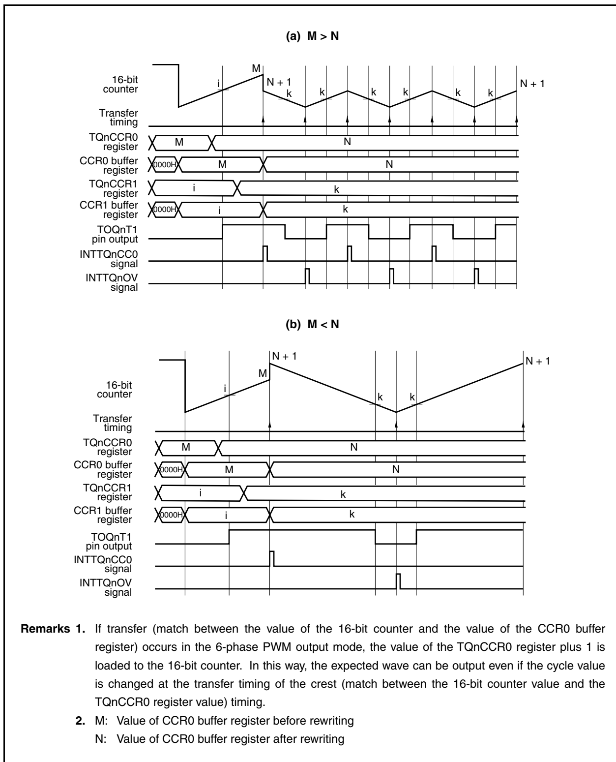
Figure 10-28. Example of Rewriting TQnCCR0 Register (During Counting Up)
