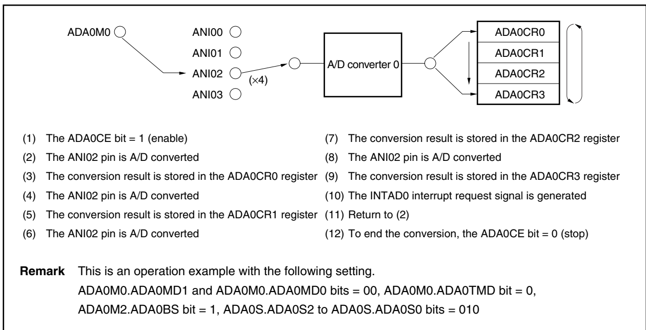
Figure 12-12. Example of 4-Buffer Mode Operation (4 Buffers of Software Trigger Continuous Select): V850E/IA4
