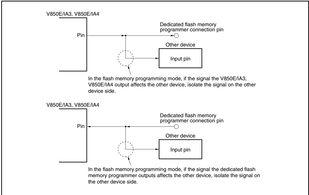
Figure 22-10. Malfunction of Other Device
