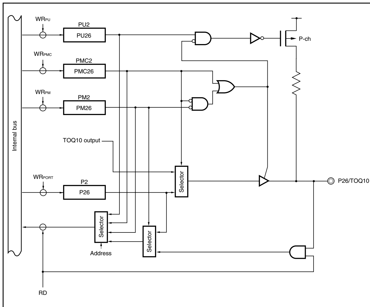
Figure 4-10. Block Diagram of P26 Pin
