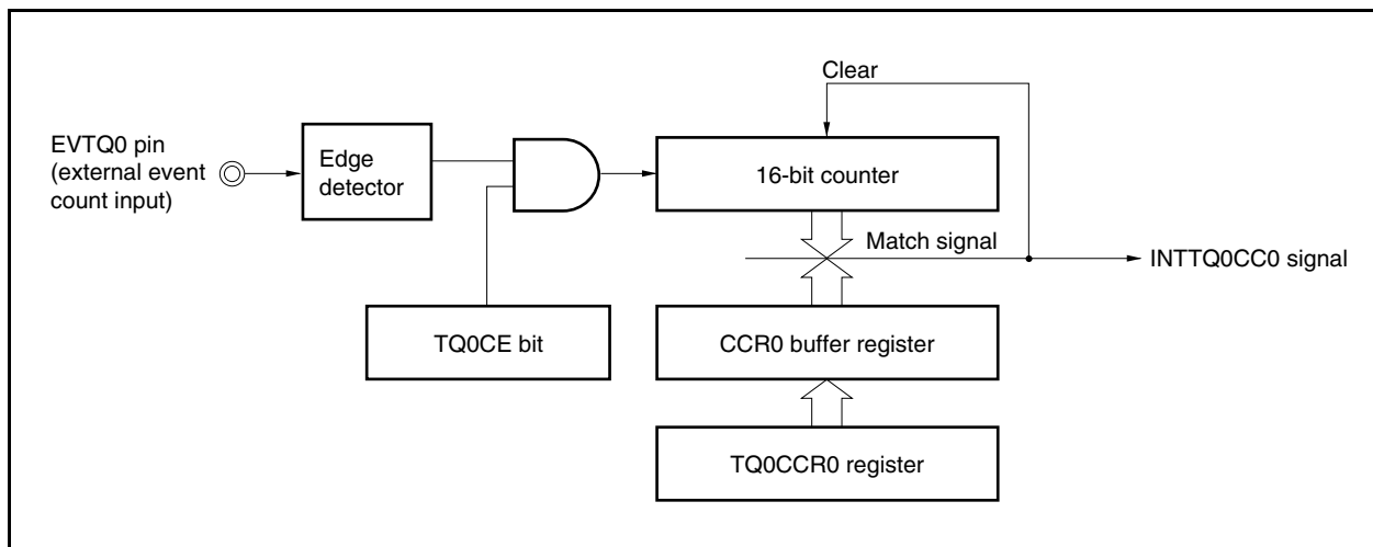
Figure 7-14. Configuration in External Event Count Mode
