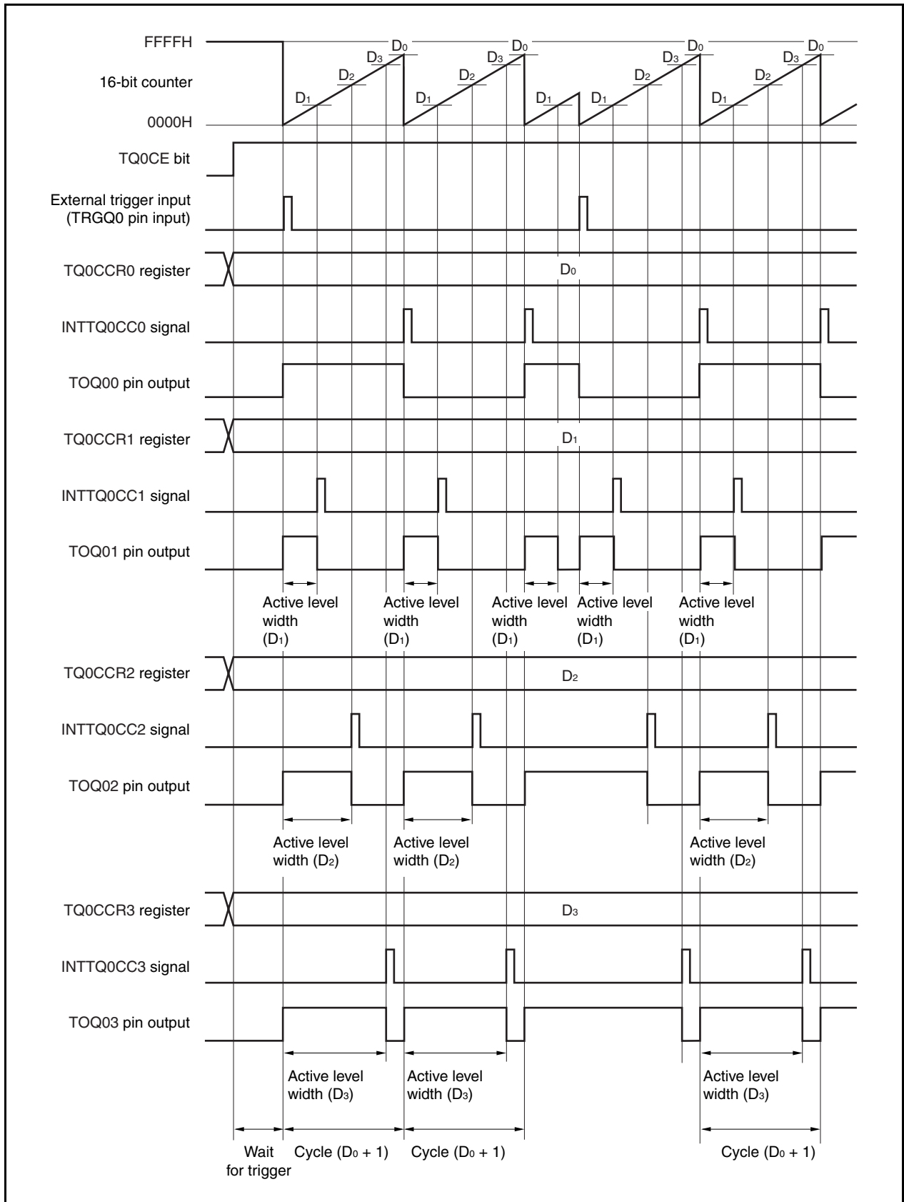
Figure 7-22. Basic Timing in External Trigger Pulse Output Mode
