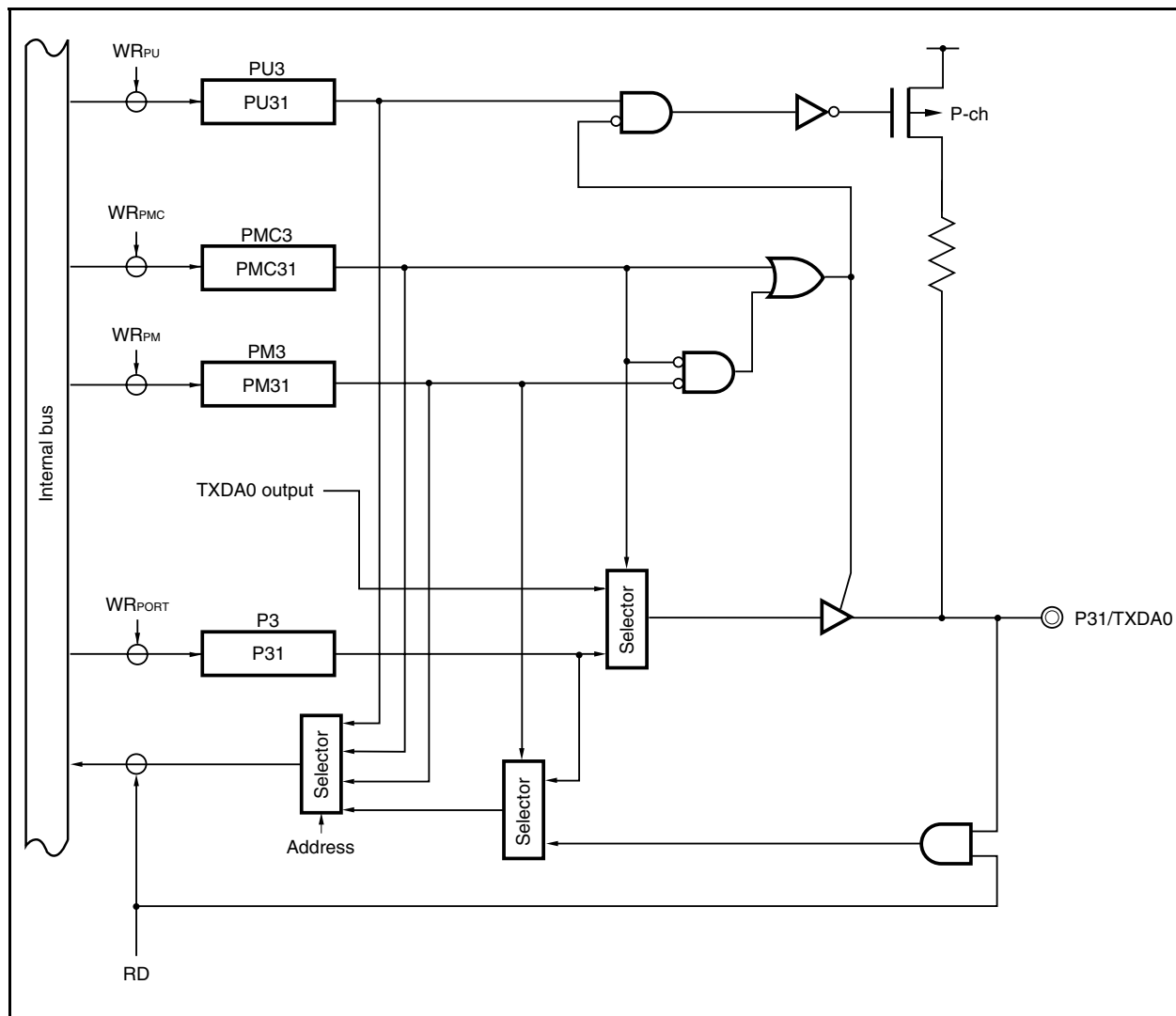
Figure 4-12. Block Diagram of P31 Pin
