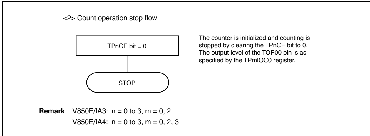
Figure 6-12. Software Processing Flow in Interval Timer Mode (2/2)
