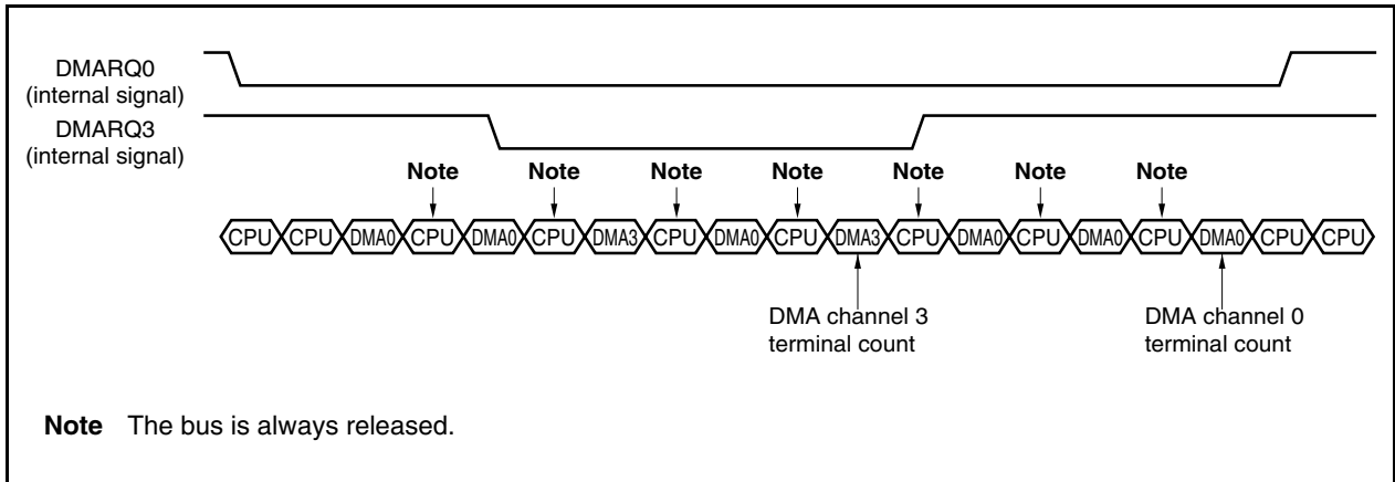
Figure 16-3. Single Transfer Example 3
