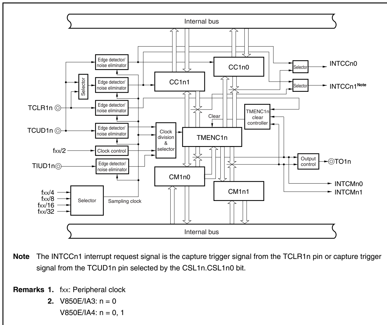
Figure 8-1. Block Diagram of Timer ENC1n
