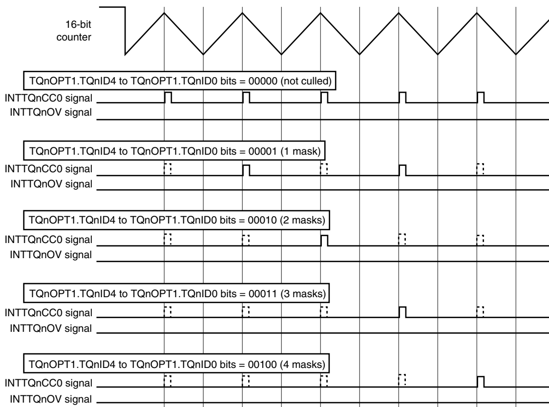
Figure 10-16. Interrupt Culling Operation When TQnOPT1.TQnICE Bit = 1, TQnOPT1.TQnIOE Bit = 0, TQnOPT2.TQnRDE Bit = 1 (Crest Interrupt Output)
