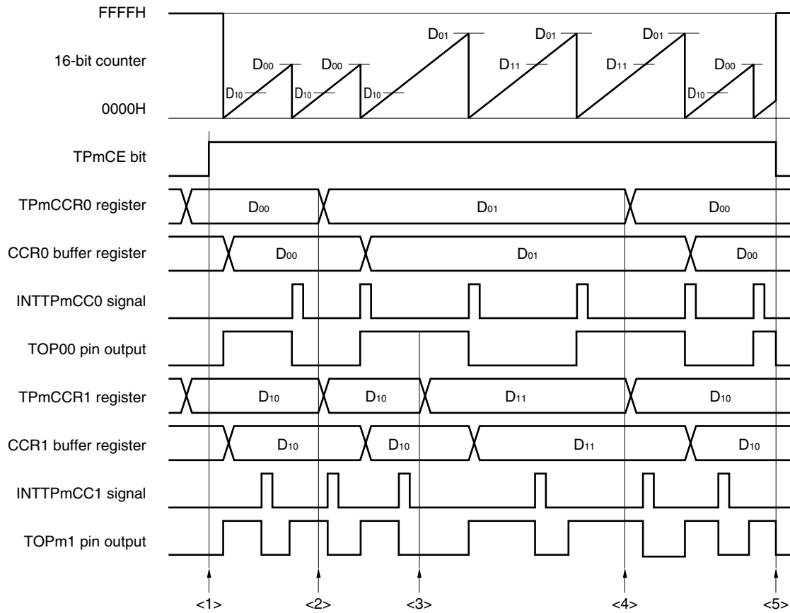
Figure 6-34. Software Processing Flow in PWM Output Mode (1/2)
