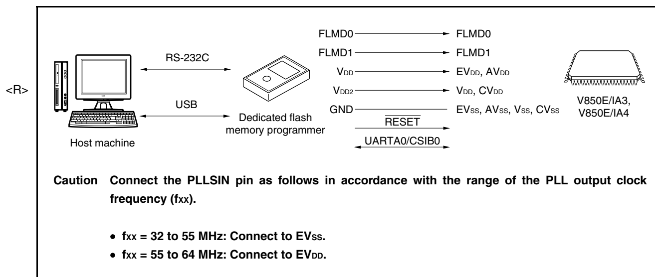
Figure 22-2. Environment Required for Writing Programs to Flash Memory
