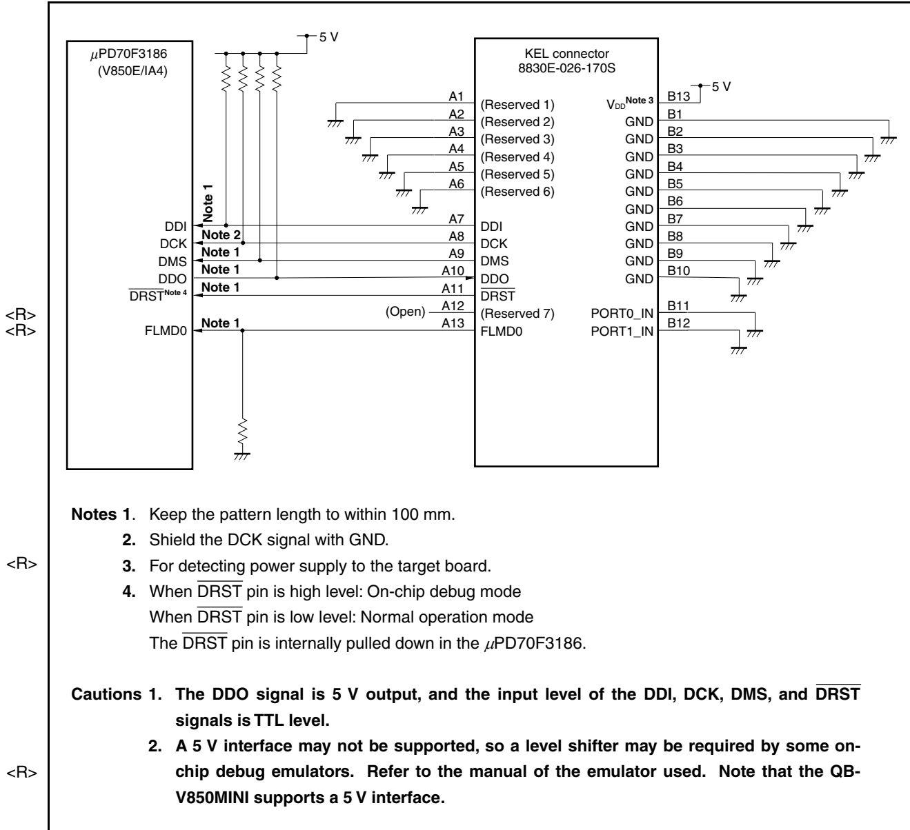
Figure 21-3. Example of Recommended Connection of \mu PD70F3186 (V850E/IA4) and KEL Connector
