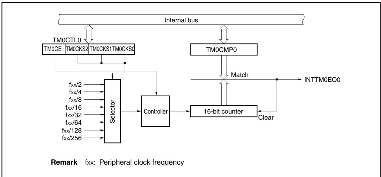
Figure 9-1. Block Diagram of TMM0
