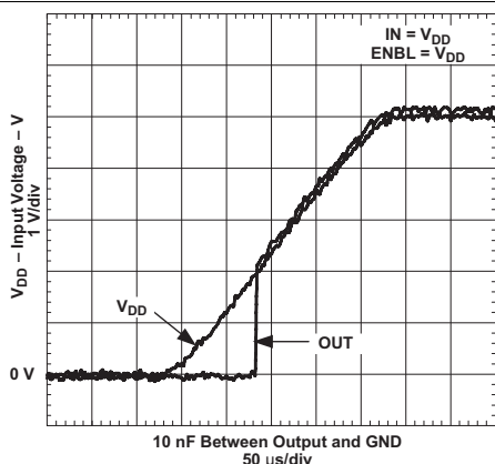
Figure 28. Output Behavior vs VDD (UCC37322)
