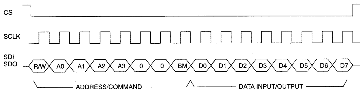
Figure 2. SERIAL PORT READ/WRITE
