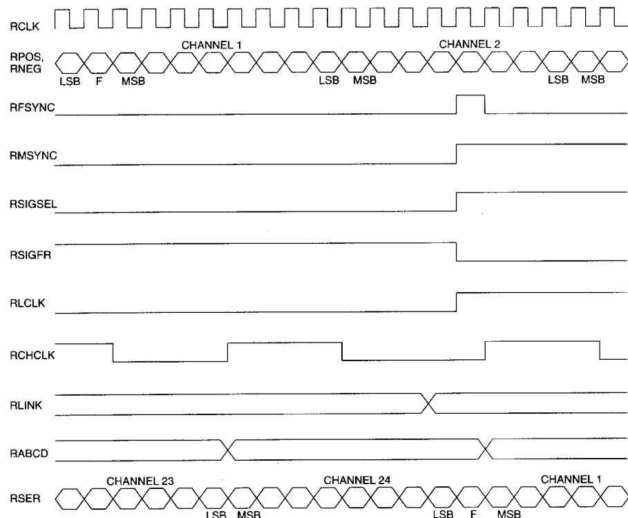
Figure 5. RECEIVE MULTIFRAME BOUNDARY TIMING
