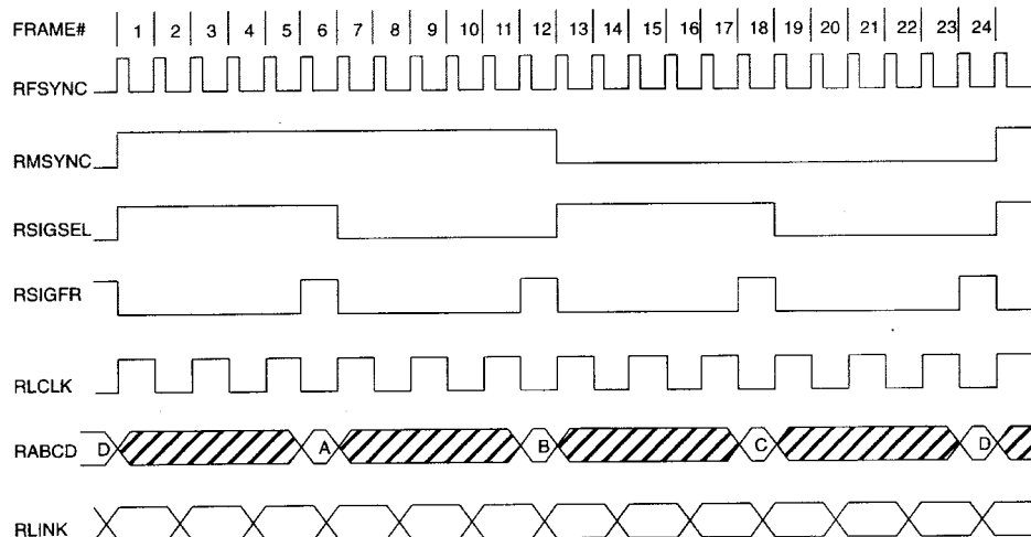
Figure 4. 193E RECEIVE MULTIFRAME TIMING
