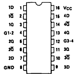
(TOP VIEW) Pin Assignment
