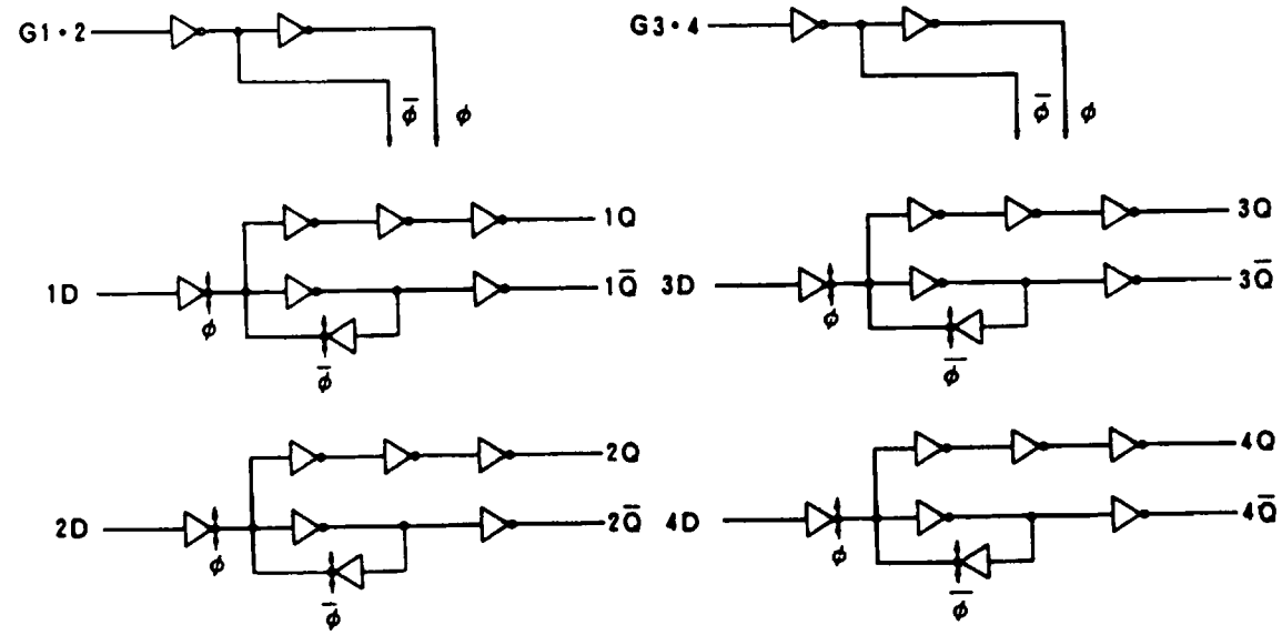
Logic Diagram
