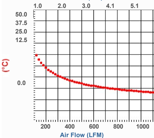
Heat Sink Temperature Rise Above Ambient (100W Dissipated)
