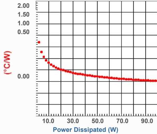
Heat Sink Thermal Resistance
