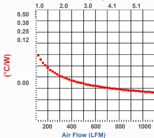
Heat Sink Thermal Resistance
