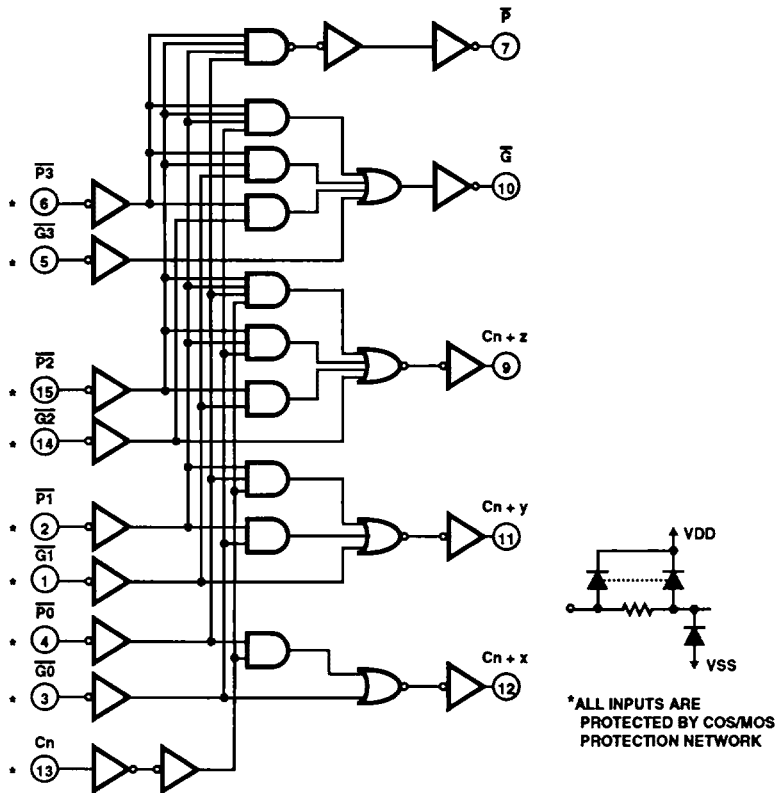
FIGURE 1. CD40182BMS LOGIC DIAGRAM
