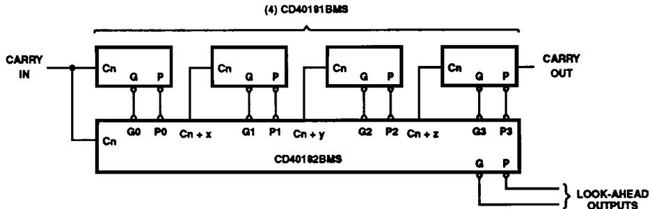
FIGURE 9. 16-BIT TWO-LEVEL LOOK-AHEAD ALU
