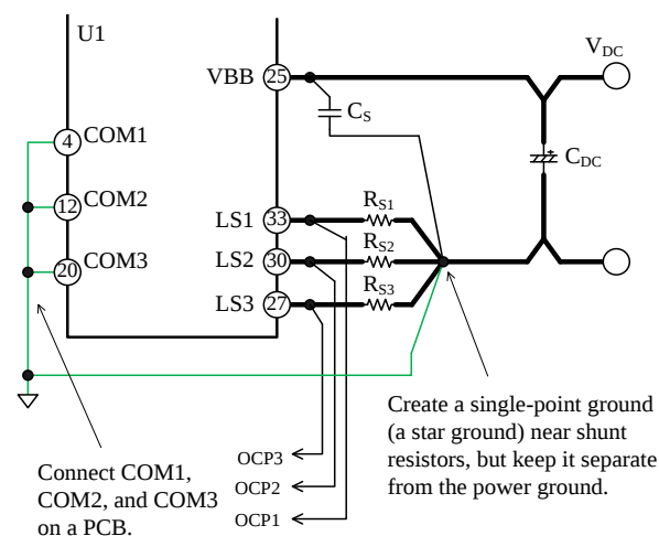
Figure 12-4. Connections to ground pin
