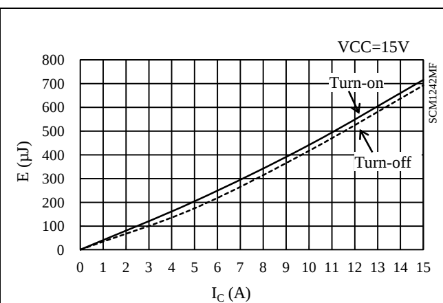
Figure 15-42. Low-side switching loss ( T_j = 125^\circ\text{C} )
