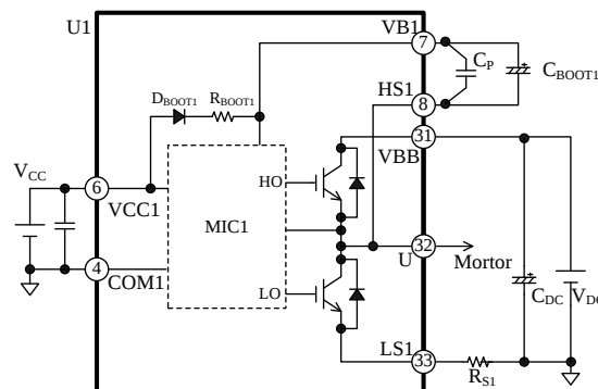
Figure 12-1. Bootstrap circuit
