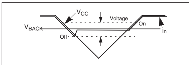
Figure 2. Power Control
