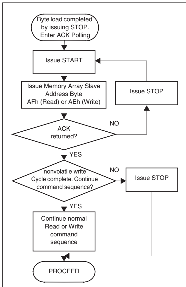
Figure 15. Acknowledge Polling Sequence
