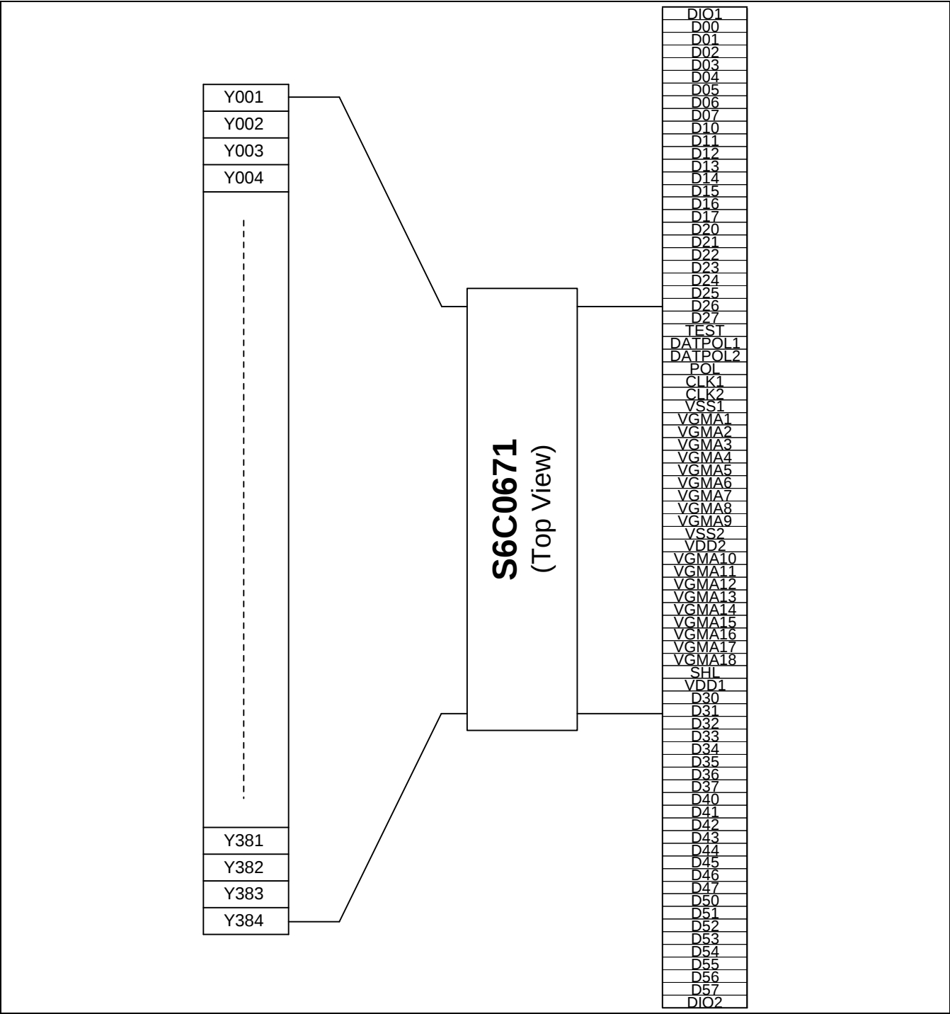
Figure 2. S6C0671 Pin Assignments
