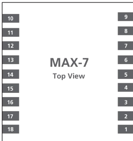
Figure 2: Pin Assignment
