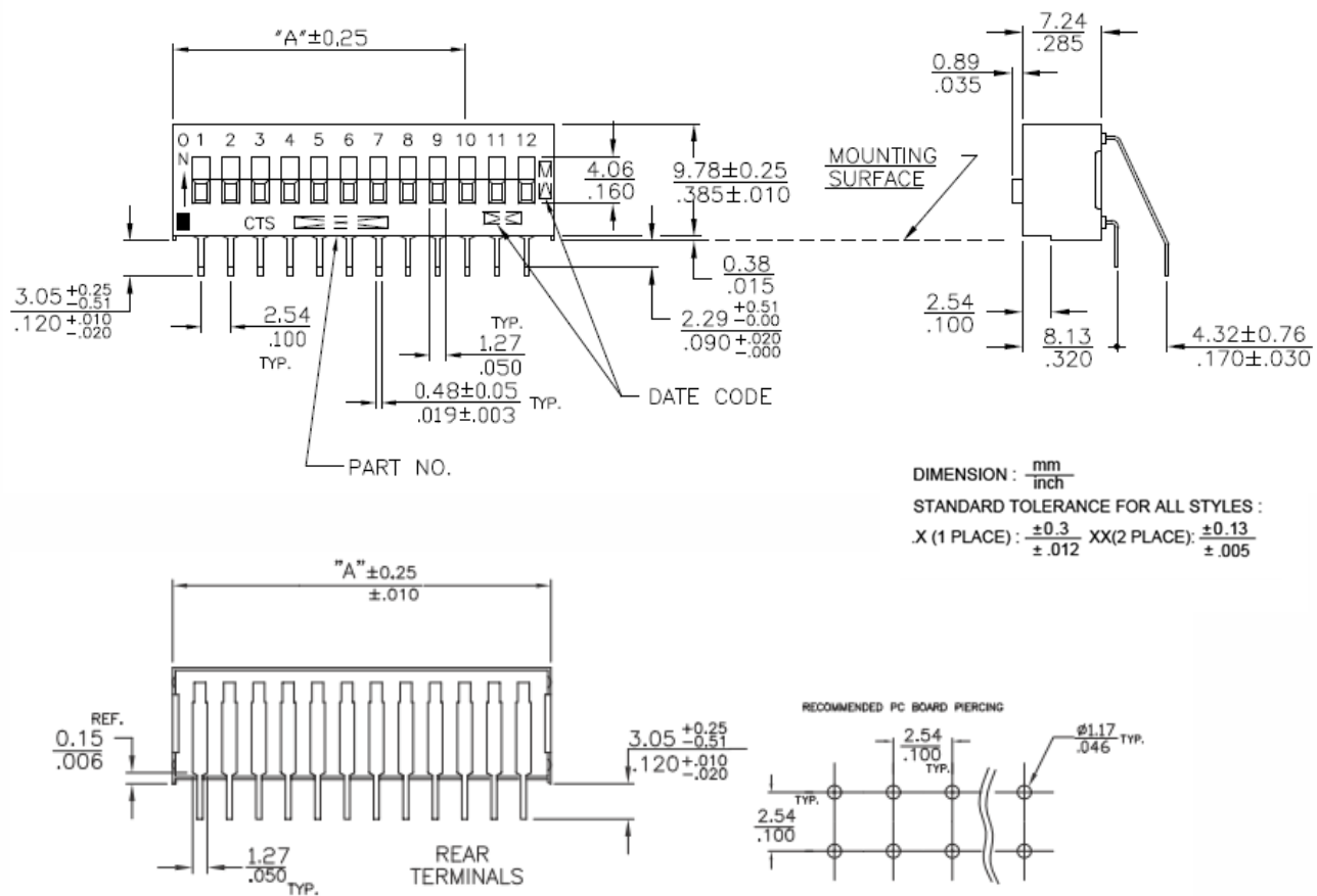
Figure 1 – SPST
