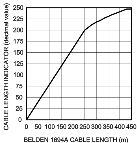
FIGURE 12. CLI vs. Belden 1694A Cable Length
