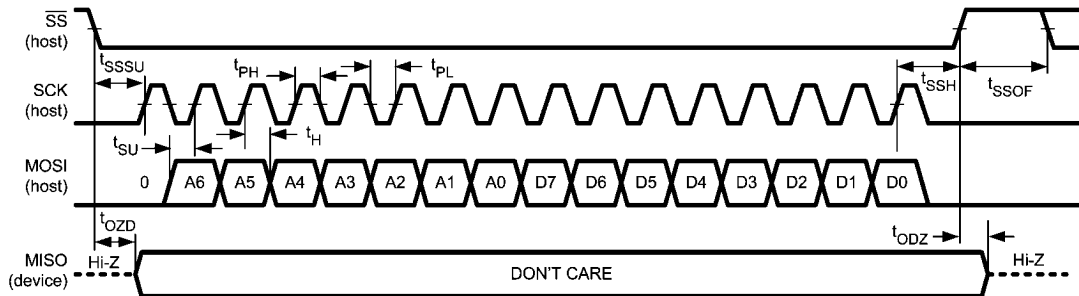
FIGURE 2. SPI Write
