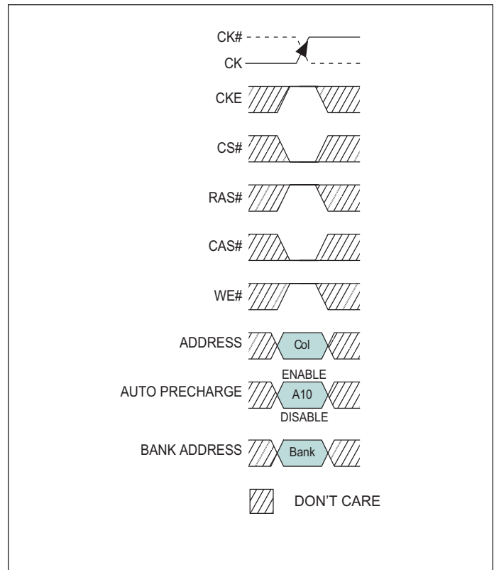
FIGURE 11 – READ COMMAND
