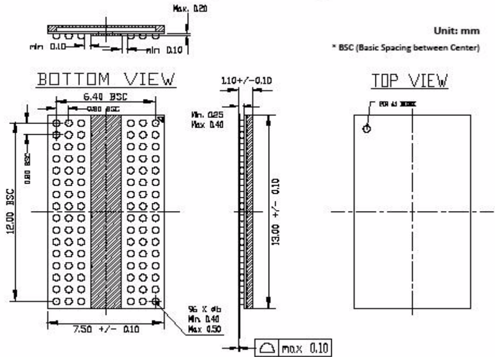
Package Outline Drawing
