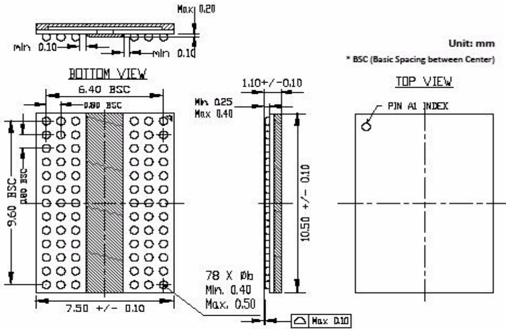
Package Outline Drawing
