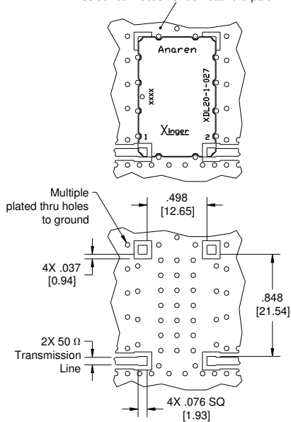
Dimensions are in Inches [Millimeters] XDL20-1-027 Mounting Footprint
