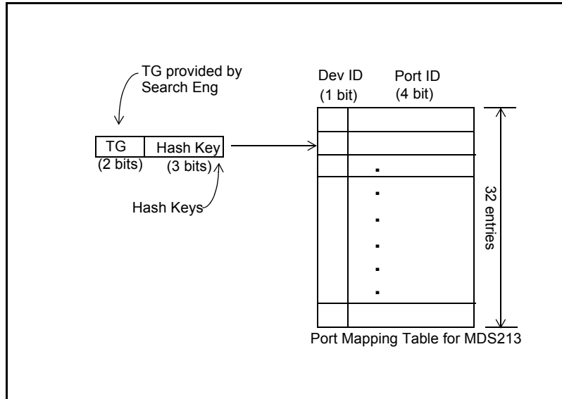
Figure 23 - Port Mapping Table
