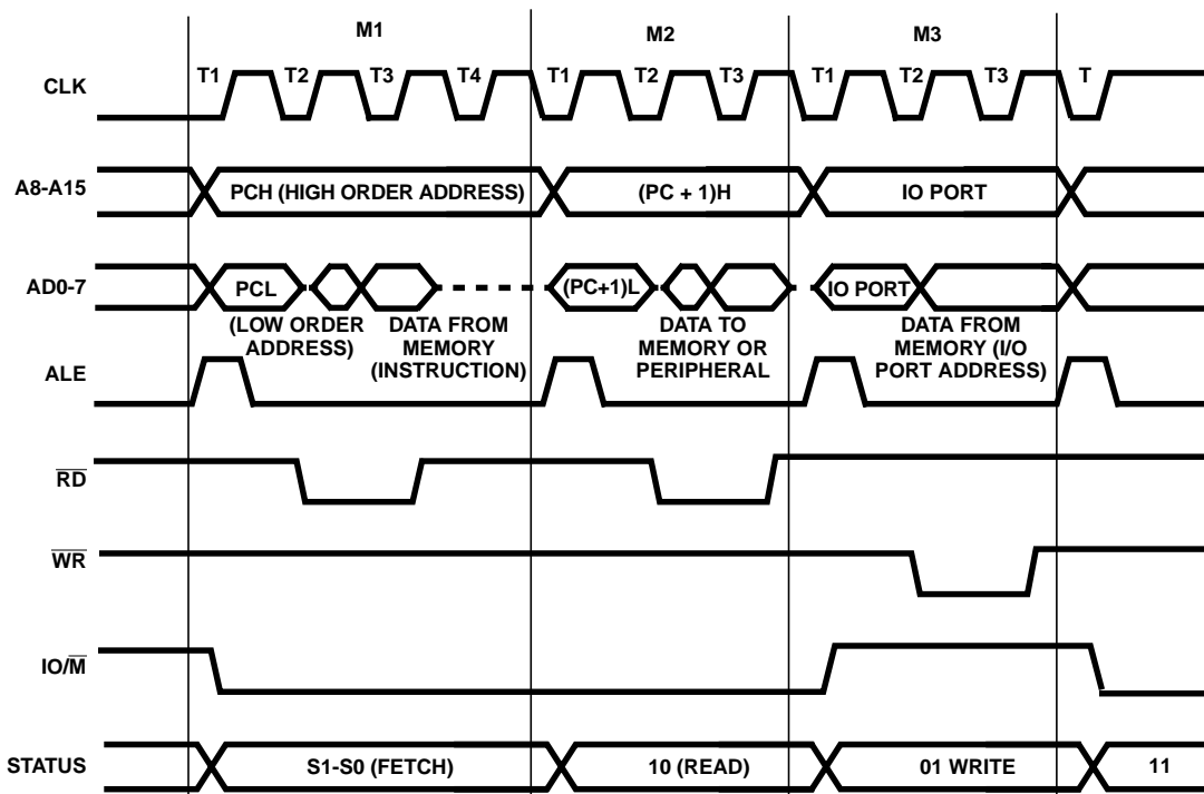
FIGURE 15. 80C85RH BASIC SYSTEM TIMING
